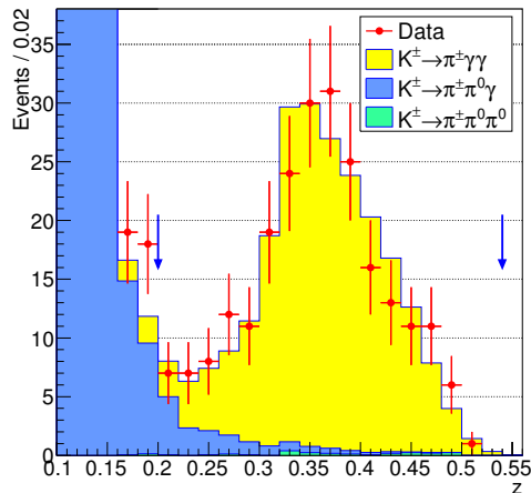
Figure 4: Reconstructed z spectrum. The estimated signal corresponds to the result of a ChPT O(p^6) fit. Signal region limits are indicated with vertical arrows.
