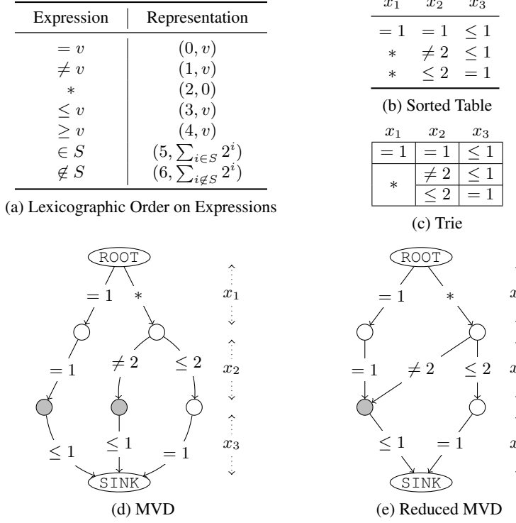
Fig. 3: Turning a bs -table into a bs -MVD using \text{pReduce}_{bs} .
