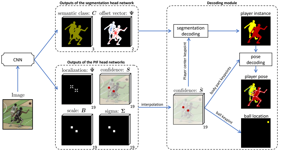
Figure 1: An overview of DeepSportLab. Our CNN outputs: (i) semantic class scores, (ii) offset vectors to associate pixels to their instance center, and (iii) a set of low resolution outputs used to generate the high-resolution keypoint confidence maps. This set includes the keypoints confidence map, the keypoints localization vectors, the size (or width) of the keypoints, and the scale parameters, which is used for scaling the per-keypoint localization loss (see Eq. (2)). The segmentation decoding module fuses the first two outputs and the high-resolution confidence map ( i.e. , only the map of the center-of-the-player keypoint) in order to predict the player masks. The confidence maps of the body part keypoints and the resulting player masks are then fused by the pose decoding module and yield the player poses. Finally, the location of the ball is extracted from the high-resolution map of the ball keypoint. Such pipeline results in a light-weight decoding process. Note that the images in this figure are only for visualization purposes and are neither the ground truth annotations nor the predicted maps. In the outputs of the PIF head networks, we only show the maps associated with the center-of-the-player keypoint.
