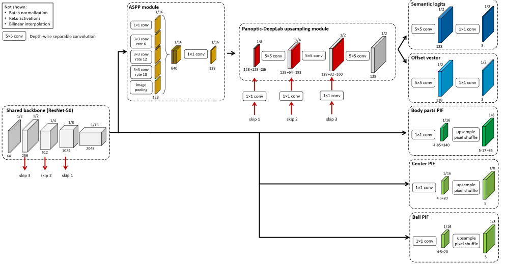
Figure 2: CNN architecture of DeepSportLab. Our network adopts an ASPP module, an upsampling module, and a dual-branch for the segmentation head. The upsampling module involves a bilinear interpolation before each concatenation step. The network also adopts a dual-PIF head network outputting the PIFs for the 19 keypoint-types. For lighter visualization, we concatenated the three PIF outputs in Fig. 1.
