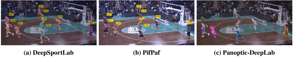
Figure 3: Pose recognition and mask segmentation samples. Body parts are shown with red and green colors as prediction and ground truth, respectively. The numbers highlighted in yellow are OKS values for their corresponding prediction-annotation matching. In addition, colors are used to show the segmented player masks.
