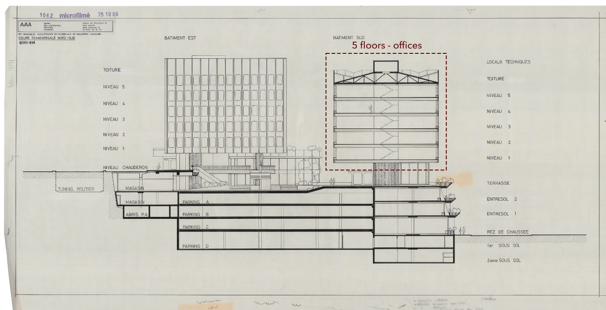
Fig. 3. Chauderon Administrative building, transversal section. In the red box the five office stories analyzed in the present paper. (For interpretation of the references to colour in this figure legend, the reader is referred to the Web version of this article.)
