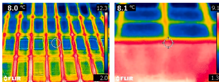
Fig. 5. Thermography results underline the relevant thermal losses through the panels' joints (left) and in correspondence of the porch slab (right).
