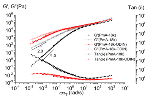
Figure 5. Built master curve of PmA-18k and PmA-18k-ODIN at T \approx T_g + 40 °C using the shift factors of PmA.
