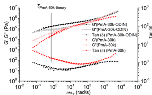
Figure 6. Master curve of PmA-30k-ODIN in comparison with PmA-30k at T \approx T_g + 40^\circ\text{C} using the shift factors of PmA. The vertical line shows the theoretical terminal relaxation time for linear PmA with 60 kg mol -1 at T = 55^\circ\text{C} .
