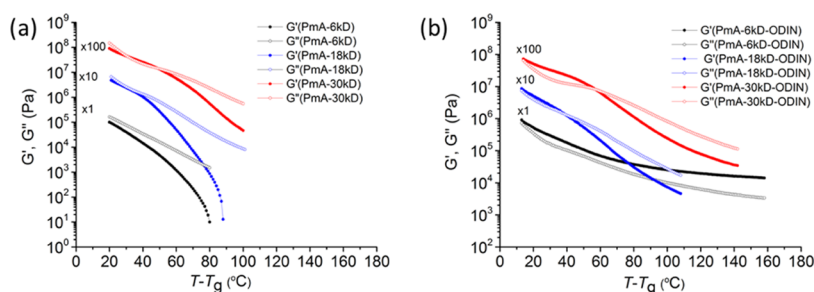
Figure 2. Temperature sweep measurements (at \omega = 1 Hz) for (a) PmA- i and (b) PmA- i -ODIN using the small-amplitude oscillatory shear (SAOS) technique.
