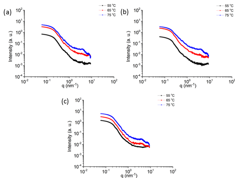
Figure 9. Variable-temperature small-angle X-ray scattering (VT-SAXS) for (a) PEG-1-ODIN, (b) PEG-2-ODIN, and (c) PEG-4-ODIN at 55, 65, and 75 °C (at T > T_m ) (data are shifted vertically for clarity).
