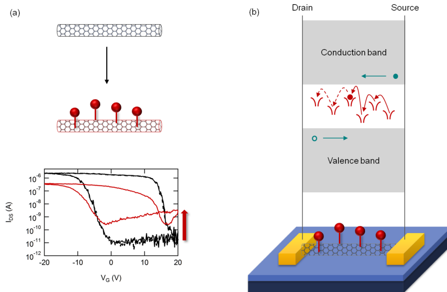
Figure II.20. (a) Transfer curves of pristine and covalent functionalized SWCNTs, highlighting the increase of the OFF-state and (b) representation of the hopping transport between functionalization induced gap states.
