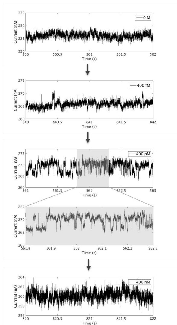
Figure VII.7. Real-time electrical response of device A6 ( V_G = 0 V; V_{DS} = 100 mV) upon exposure to dimethylphenylsilane solutions in concentrations of 0 M, 400 fM, 400 pM and 400 nM. I(t) curves are shown over 2 s and 0.5 s time intervals (zoom, grey shaded areas).
