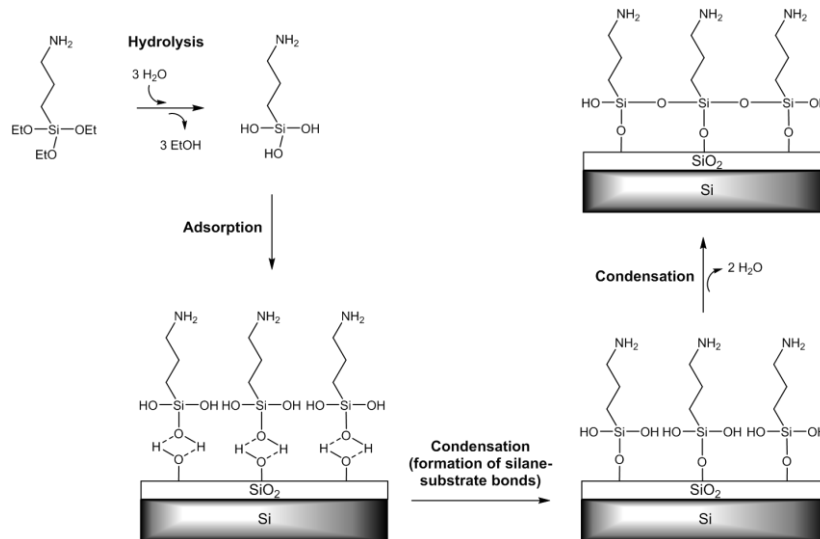
Figure III.2. Schematic representation of the functionalization of oxidized silicon substrate by APTES. Figure inspired from Howarter et al. 222
