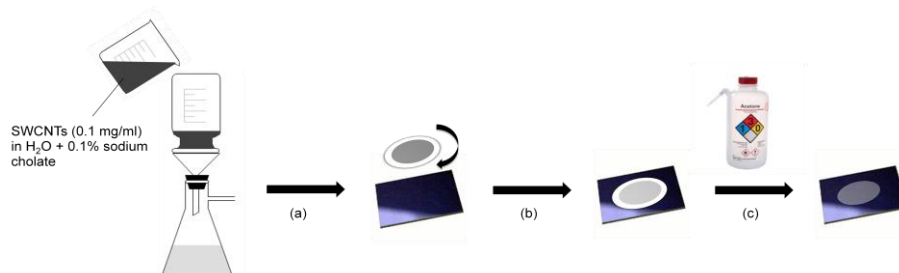
Figure IV.7. Schematic representation of the deposition process of SWCNTs films on Si/SiO 2 substrate: (a) a SWCNTs film is prepared by filtration on nitrocellulose membrane of a diluted suspension of SWCNTs in aqueous solution; (b) the film is deposited on a clean Si/SiO 2 wafer; (c) the nitrocellulose membrane is dissolved by acetone.
