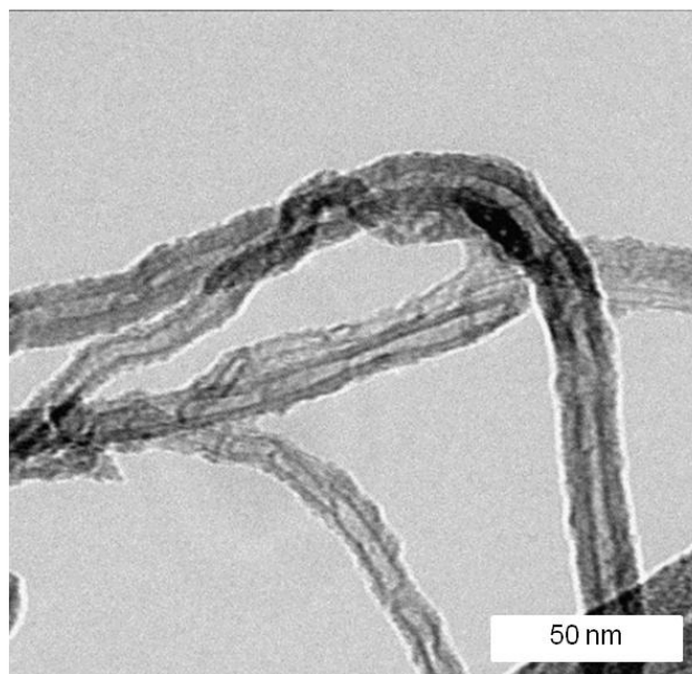
Figure V.6. TEM images of Ru/MWCNTs before catalysis and after 6 runs of catalysis.
