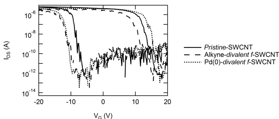
Figure VI.14. Transfer curves ( V_{\text{DS}} = 1 \text{ V} ) of pristine -SWCNT, alkyne-divalent f -SWCNT and Pd(0) complexes coordinated on divalent f -SWCNT.
