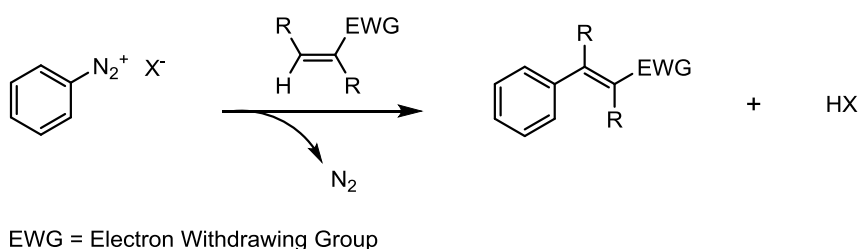
Figure IV.1. Schematic representation of the Meerwein reaction between an aryl diazonium salt and an alkene.
