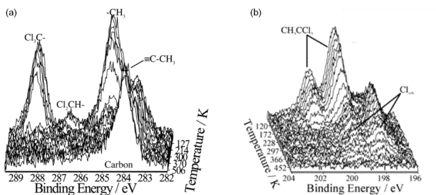
Figure I.15. Time resolved XPS spectra of 1,1,1-trichloroethane reaction in function of temperature: (a) C 1s and (b) Cl 2p spectra. Adapted with permission from 101 . Copyright © 2004 American Chemical Society.
