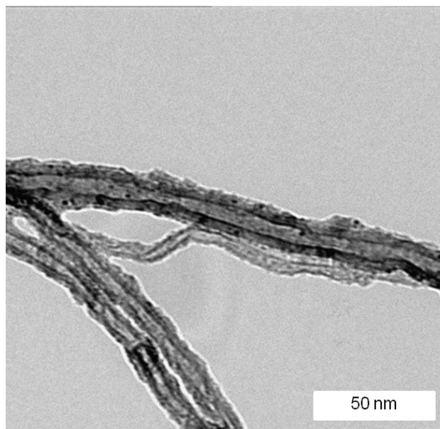
Figure V.7. TEM images of Ru 5 Pt/MWCNTs before catalysis and after 6 runs of catalysis.
