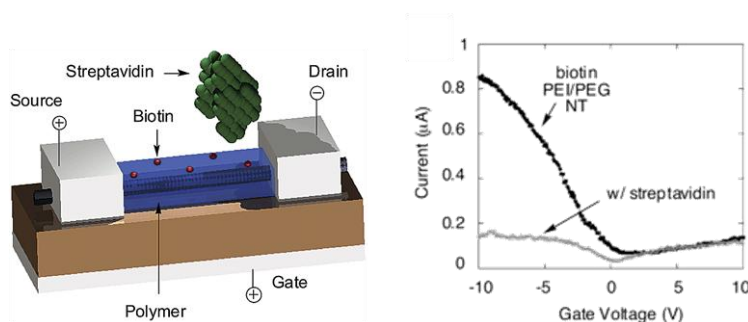
Figure I.8. (Left) Schematic representation of a biotin-functionalized CNT sensor for the selective detection of streptavidin. (Right) Electrical response of the device in absence and presence of streptavidin. Adapted with permission from 49 . Copyright © 2003 American Chemical Society.
