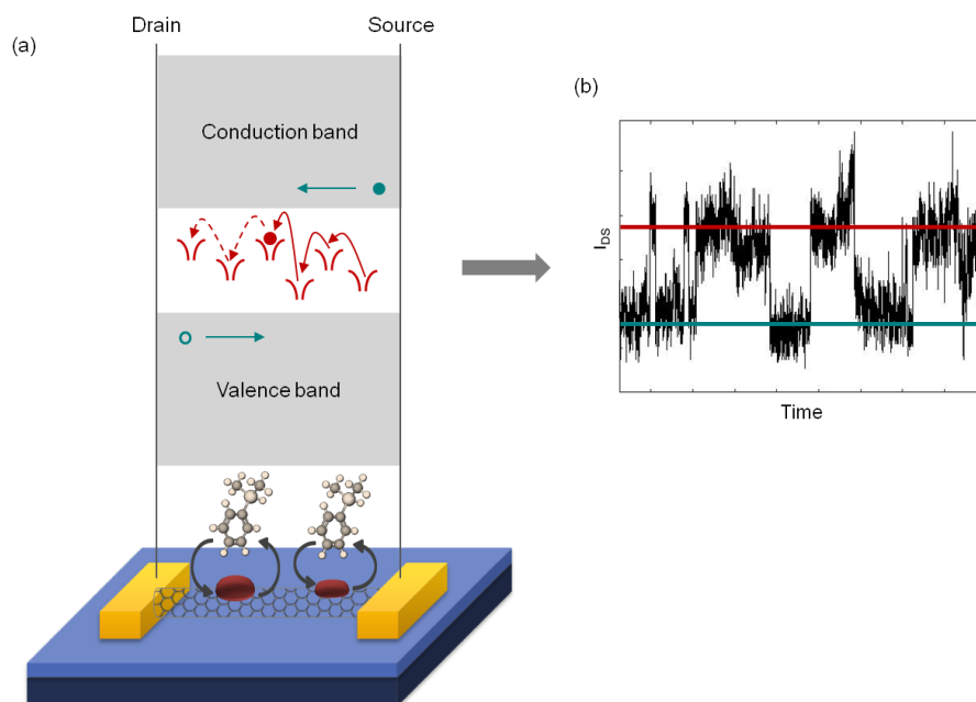
Figure VII.6. Schematic representation of the midgap states-induced two level current fluctuations: (a) formation of midgap states induced by specific interactions between nanoparticles and dimethylphenylsilane molecules and (b) impact of these midgap states on the nanotube conductance. Red line in (b) corresponds to the current flowing through valence or conduction band and blue line corresponds to the current flowing through the midgap states induced by the NP/silane interactions.
