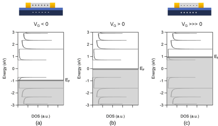
Figure II.16. Representation of the effect of the gate voltage on the doping of sc-nanotube: (a) hole conduction; (b) absence of conduction and (c) electron conduction.
