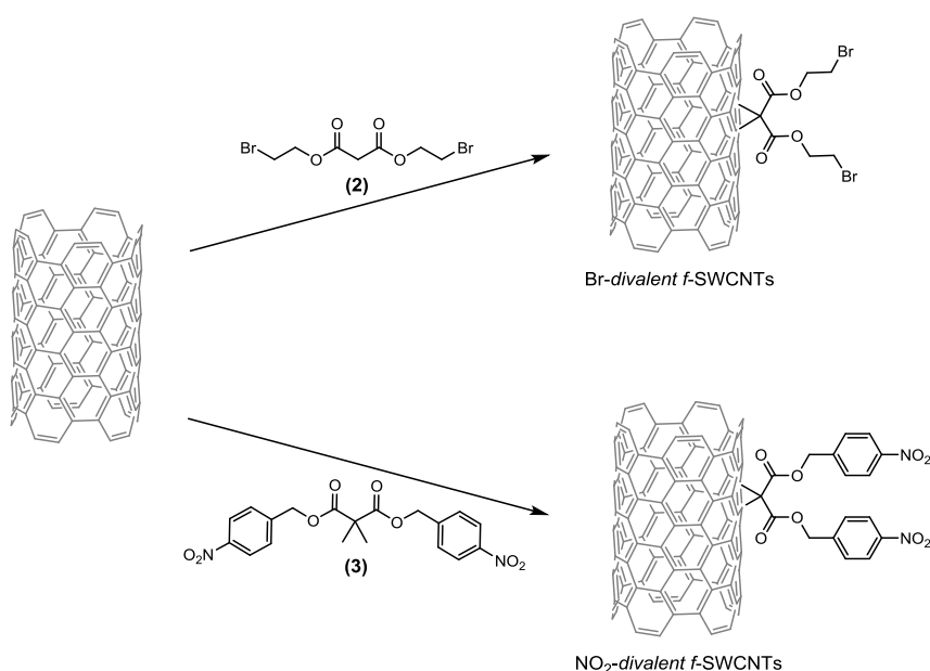
Figure VI.11. Schematic representation of the divalent functionalization of SWCNTs by Br-malonate (2) and NO 2 -malonate (3) .
