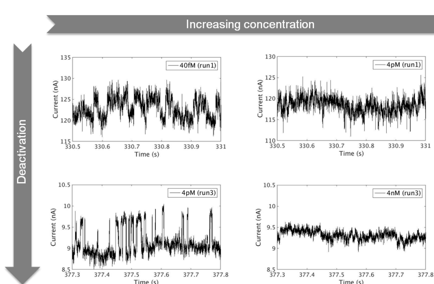
Figure VII.13. Evolution of the electrical response of device C7 ( V_G = 0 V; V_{DS} = 100 mV) with the dimethylphenylsilane concentration and catalyst deactivation: (top) first run of experiments, (bottom) third run of experiments. I(t) curves are shown over 0.5 s time intervals.
