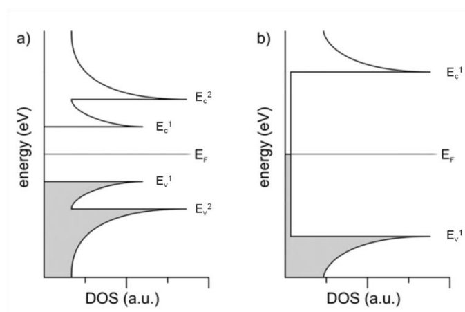
Figure II.5. Typical density of states (DOS) of (a) semiconducting SWCNT and (b) metallic SWCNT. Adapted from 133 with permission of The Royal Society of Chemistry, http://dx.doi.org/10.1039/b716732f .
