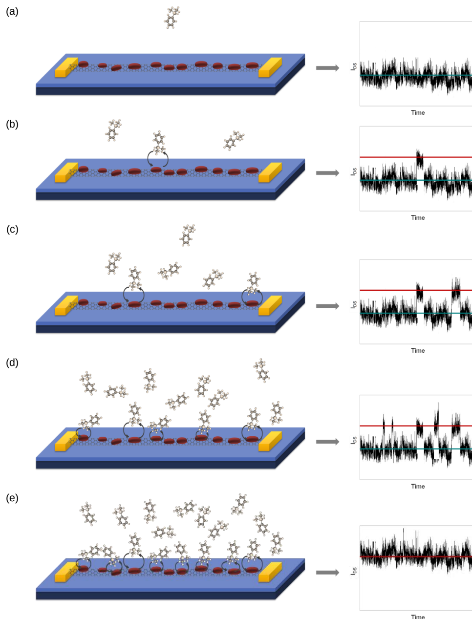
Figure VII.10. Evolution of the CNT conductance when the dimethylphenylsilane concentration is gradually increased to be (a) below the lower concentration threshold; (b) at the lower concentration threshold; (c, d); above the lower concentration threshold and (e) above the upper concentration threshold.
