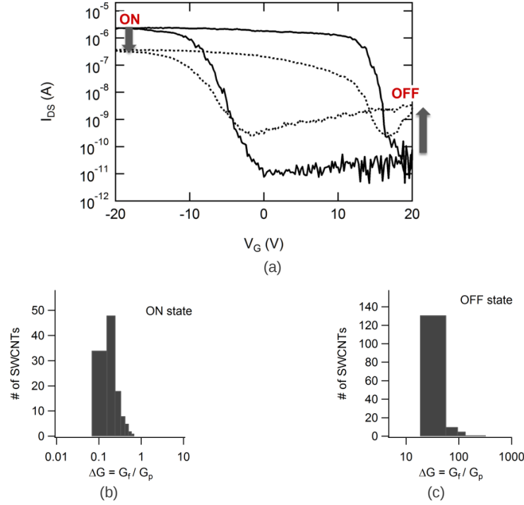
Figure IV.15. Effect of covalent functionalization of sc-SWCNT in the ON and OFF states: (a) Transfer curves for pristine (—) and functionalized (.....) SWCNT; distribution of \Delta G = G_r / G_p (b) in the ON state for 116 devices and (c) in the OFF state for 153 devices.
