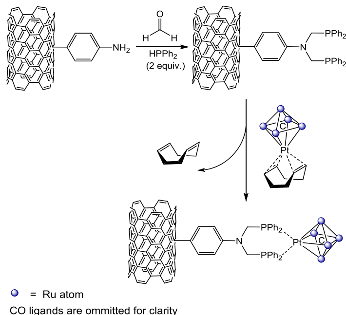
Figure IV.11. Anchoring of phosphine ligands on \text{NH}_2 -Ph- f -SWCNTs and coordination of [\text{Ru}_5\text{PtC}(\text{CO})_{14}\text{COD}] .
