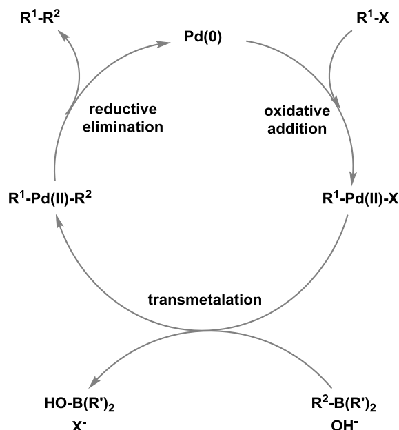
Figure VI.5. Schematic representation of the general catalytic cycle for the Suzuki-Miyaura reaction. In this catalytic cycle, the base is considered to be \text{OH}^- for clarity, but other bases can be used.
