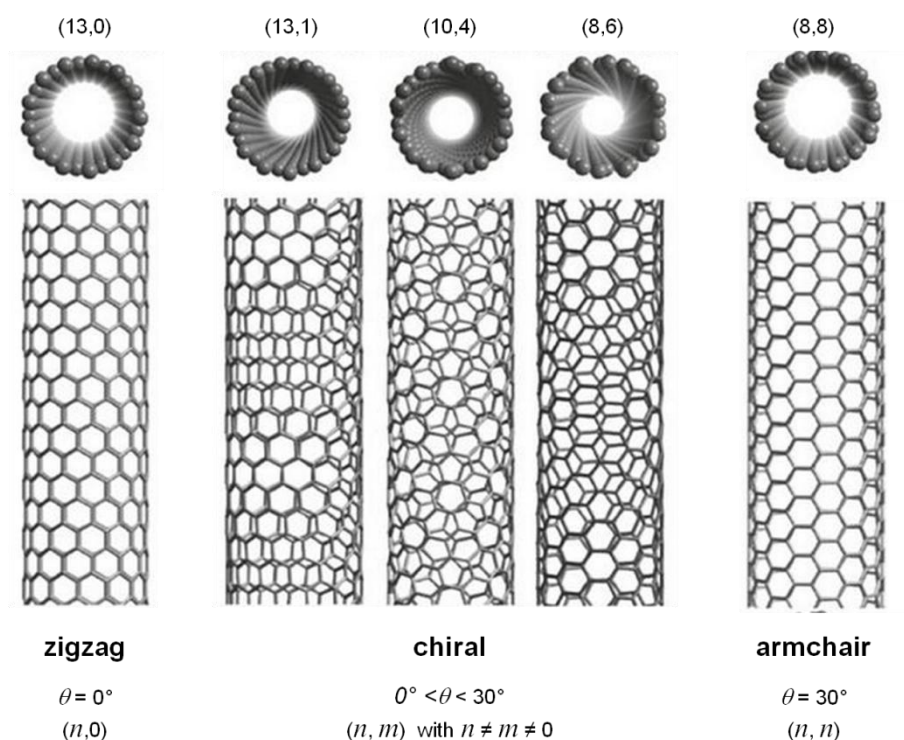
Figure II.4. Examples of zigzag, chiral and armchair SWCNTs and summary of the classification parameters. Reproduced with permission from 123 . Copyright © 2012 John Wiley & Sons Ltd.
