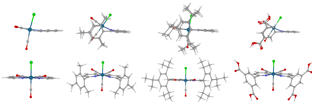
Figure 8. Calculated structures for catalysts 1 , 2 , 3 and 4 , from left to right. The tilting angles were in agreement with those determined from the crystal structure ( Figure 3 ).
