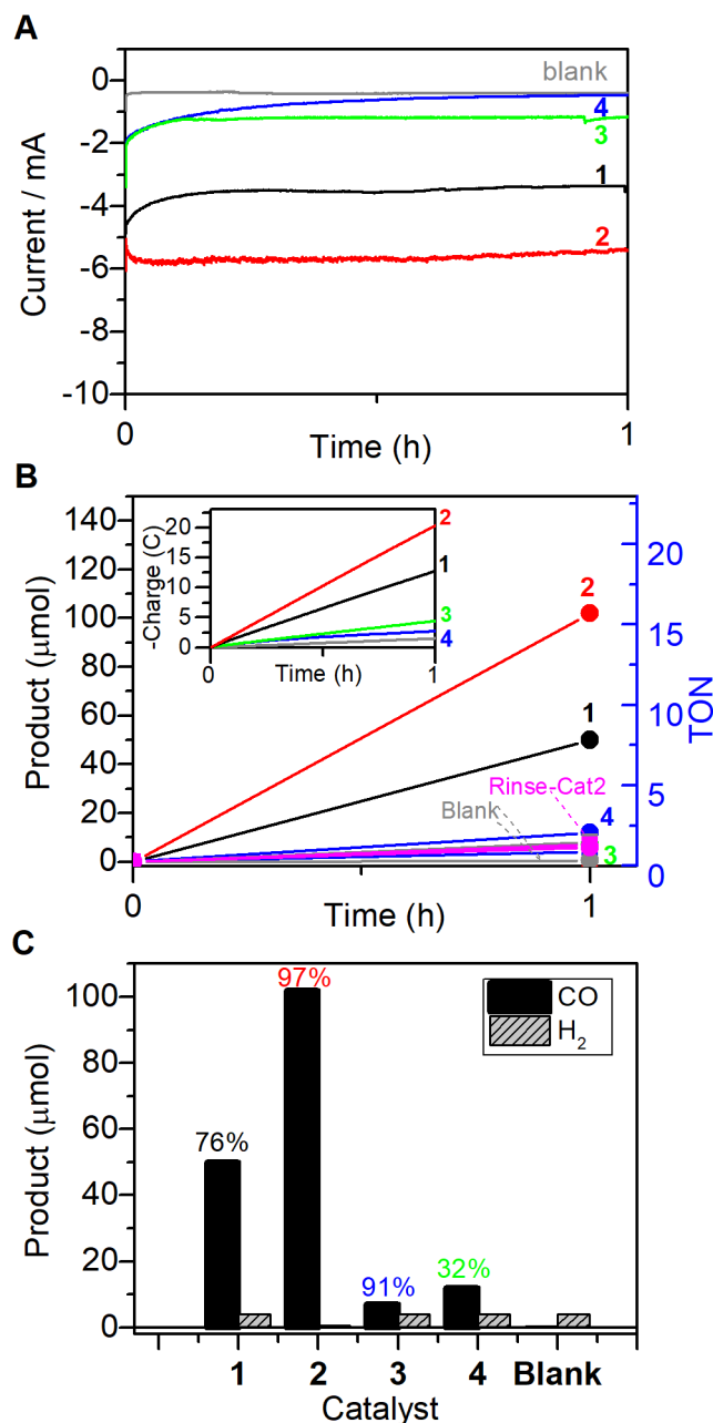
Figure 6. Controlled potential electrolysis (CPE) experiment at -1.80 V (vs. Ag/AgCl) of \text{CO}_2 -saturated DMF solutions in the presence of 6.2 M MeOH for the blank (grey), and with 1 mM of catalyst 1 (black), 2 (red), 3 (green) and 4 (blue). (A) Current-time plot for 1 hour CPE experiment. (B) product distribution analysis (circles: CO, squares: \text{H}_2 ) from the 1 hour CPE experiment along with the rinse test (magenta) by which the working electrode used with catalyst 2 was gently dipped in DMF and then the electrolysis was repeated in \text{CO}_2 saturated freshly made electrolyte in the presence of 6.2 M MeOH (inset) the corresponding charge-time plot. (C) Bar chart for the analysis of the gaseous product for CO (black solid bars) and \text{H}_2 (dashed bars), the CO Faradaic efficiency is indicated on the top of the bar for each catalyst.
