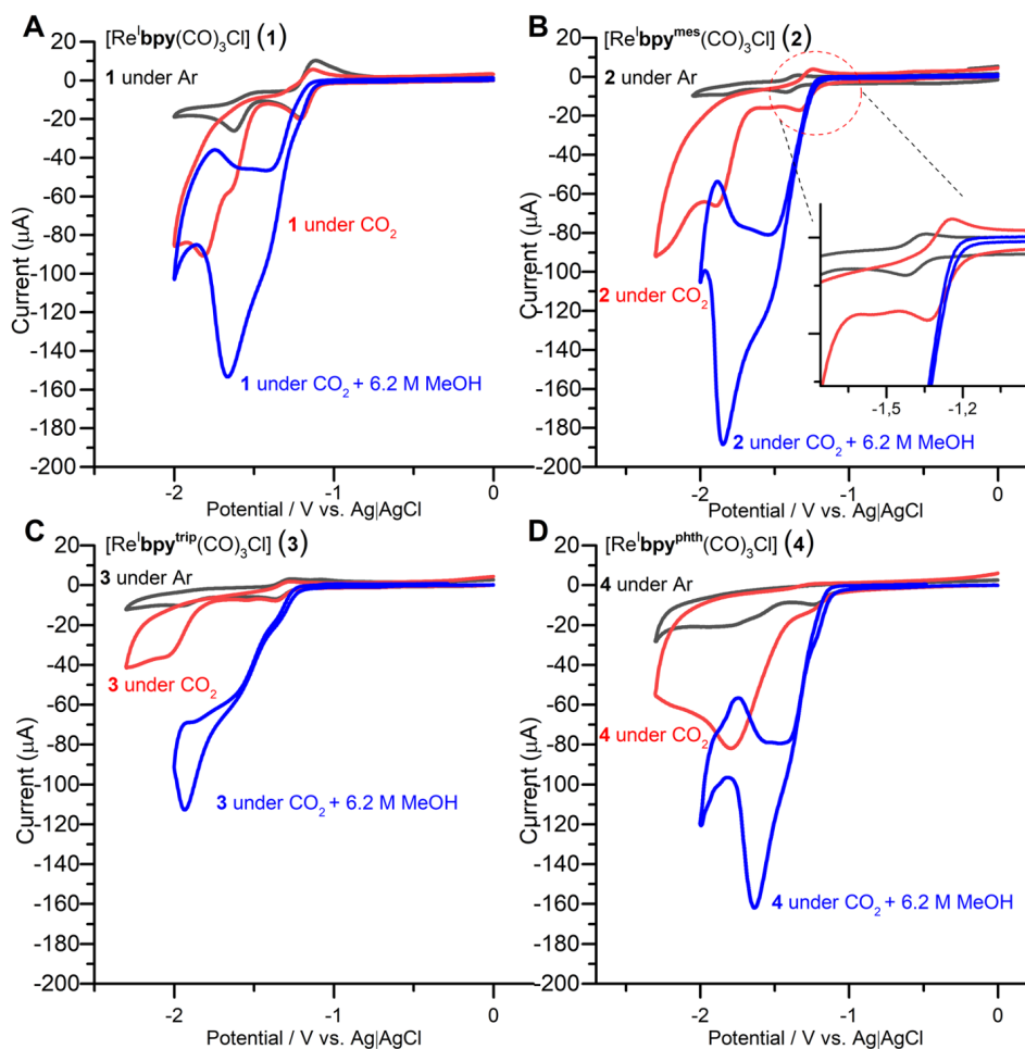
Figure 5. Cyclic voltammetry of 1 mM DMF solutions of [\text{Re}^{\text{I}}(\text{bpy})(\text{CO})_3\text{Cl}] 1 (a), [\text{Re}^{\text{I}}(\text{bpy}^{\text{mes}})(\text{CO})_3\text{Cl}] 2 (b), [\text{Re}^{\text{I}}(\text{bpy}^{\text{trip}})(\text{CO})_3\text{Cl}] 3 (c), and [\text{Re}^{\text{I}}(\text{bpy}^{\text{phth}})(\text{CO})_3\text{Cl}] 4 (d) recorded under Ar (black), \text{CO}_2 (red) and \text{CO}_2 in the presence of 6.2 M MeOH (blue). Plots with other proton sources are shown in ESI Section 6 with catalytic performance summarized in Table 3 . Inset in B shows an enlarged portion of the CV where the pre-catalytic wave is observed near the first reduction event of 2 . Conditions: 0.1 M (\text{Bu}_4\text{N})\text{PF}_6 supporting electrolyte, scan rate 100 mV/s, glassy carbon working electrode ( d = 2 mm, A = 0.03 cm ^2 ) vs. Ag|AgCl references electrode and Pt counter electrode at 20 °C. In this system E_{1/2}(\text{Fc}^+/\text{Fc}) = 0.45 \pm 0.01 V.
