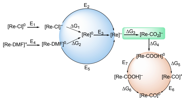
Figure 7. Computed activation steps for [\text{Re-Cl}]^0 and solvated [\text{Re-DMF}]^+ species.
