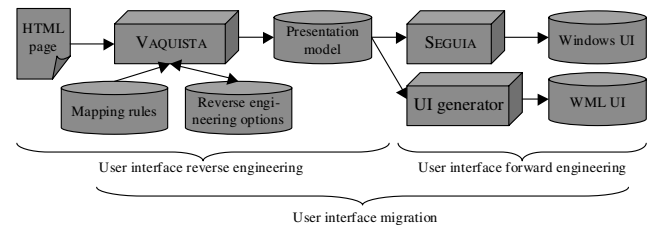
Fig. 4. The complete process envisioned with VAQUISTA.
