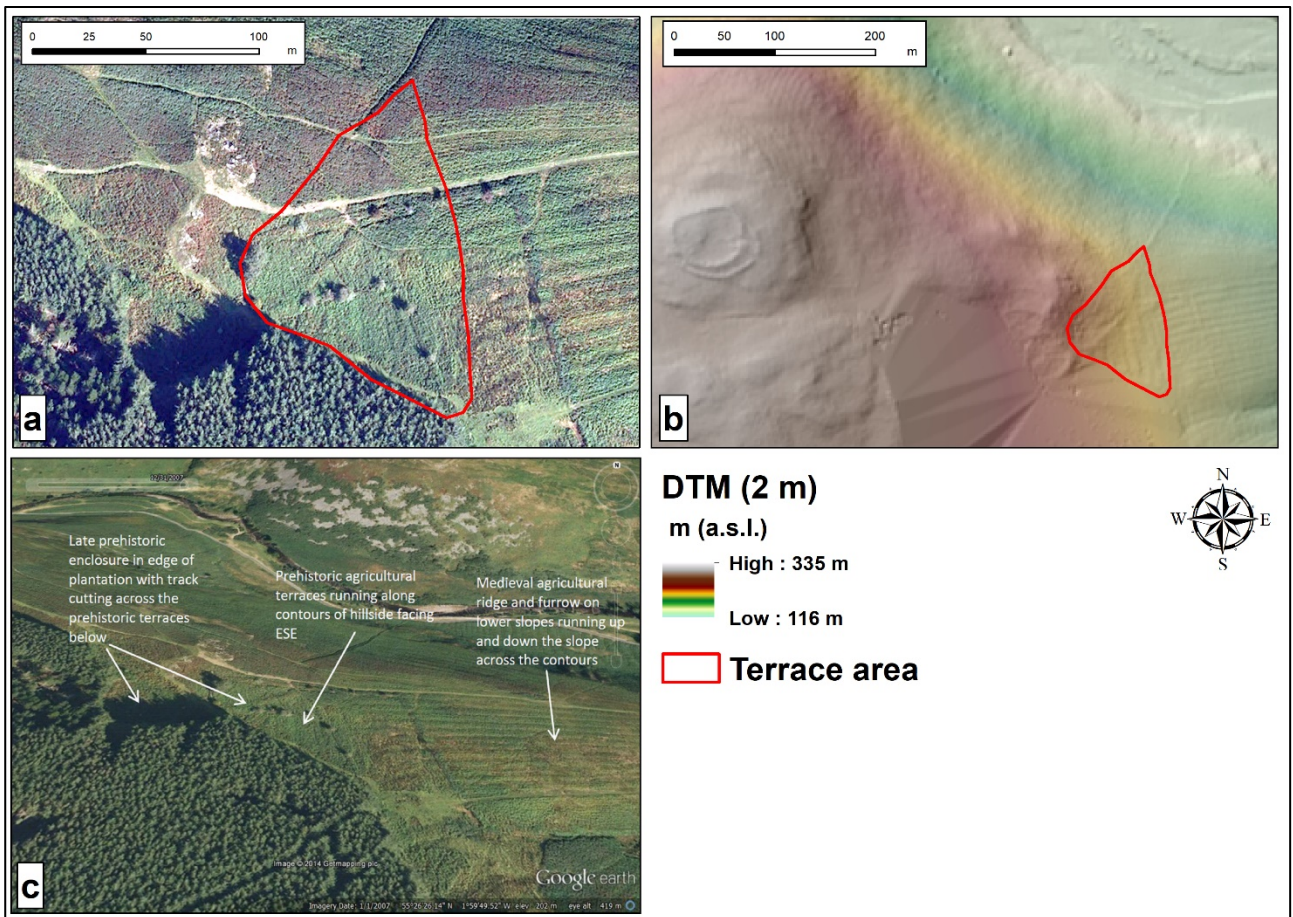
Figure 2: The Ingram terrace site: a) Orthophoto of terraces site in 2007. b) DTM of Ingram Valley at 2 m resolution provided by the UK Environment Agency. c) Screenshot of satellite imagery from Google Earth of Ingram terraces site with the prehistoric agricultural terraces, Plantation Camp enclosures, and the medieval ridge and furrow marked.
