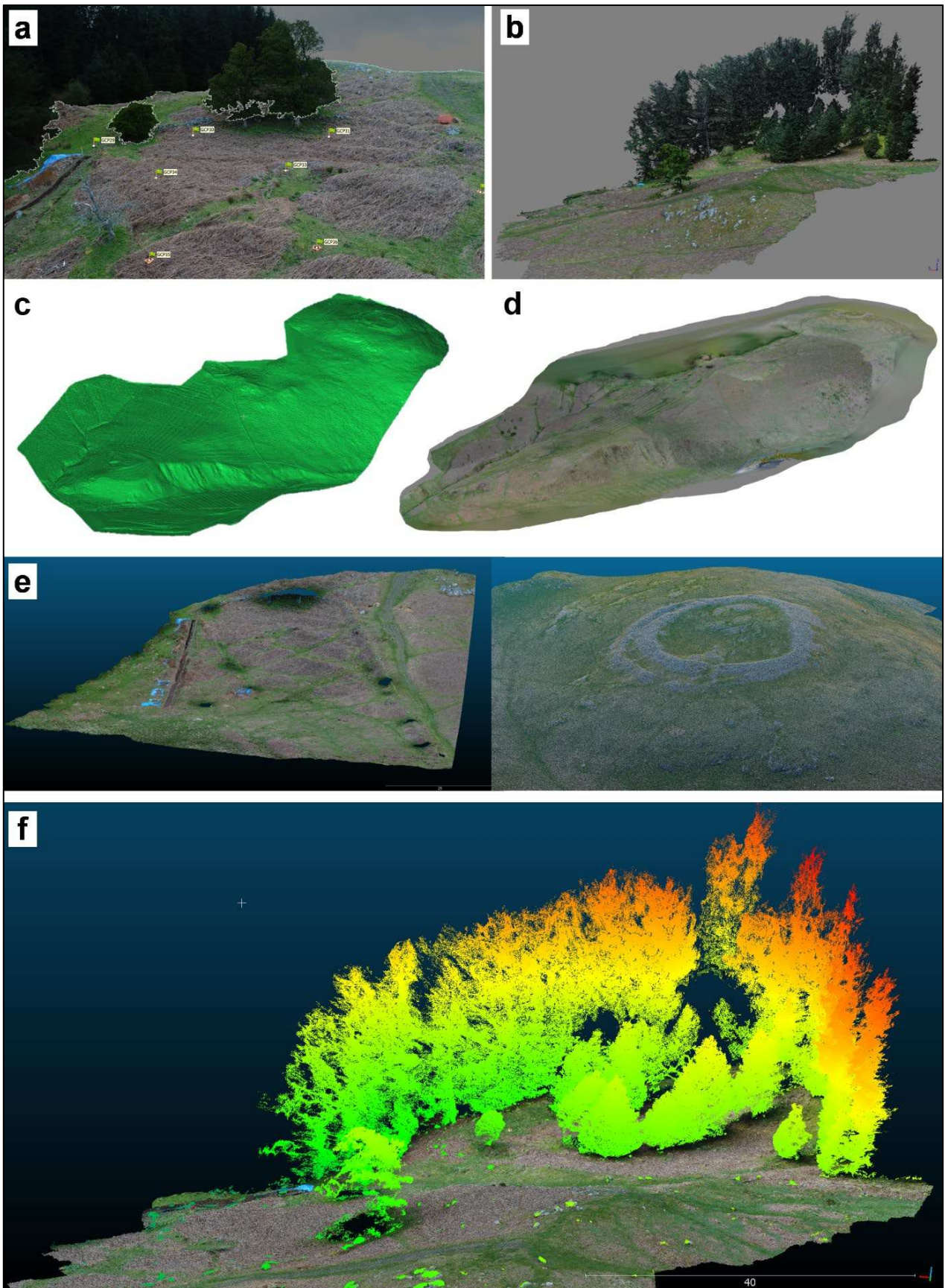
Figure 5: Examples of SfM processing steps and outputs. a) Photo of Ingram terrace area where the vegetated parts were masked and GCPs were manually located in Agisoft Photoscan. b) Point cloud of vegetated area (Fig. 4c). c) Examples of the point cloud in Ingram
