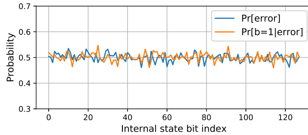
Fig. 5: Behavior of internal bits distributions.
