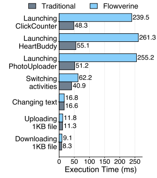
Fig. 8: Runtime benchmarking tests results.
