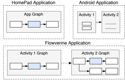
Fig. 2: Programming models compared.
