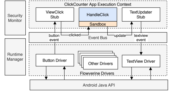
Fig. 5: Execution runtime of a ClickCounter application.
