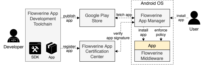
Fig. 3: Flowverine framework components and workflow.
