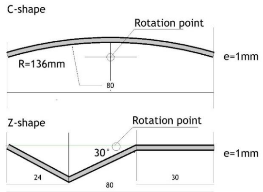
Figure 4: C-shaped (top) and Z-shaped (bottom) slats
