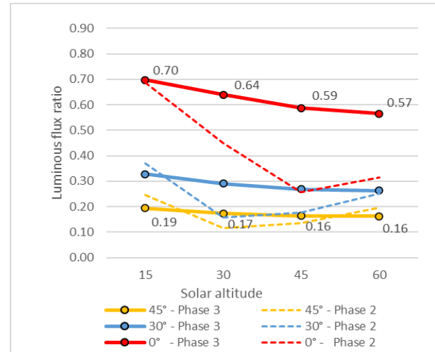
Figure 2: Luminous flux ratios for tilt angles positions – Comparison between Phase 2 and Phase 3 evaluations
