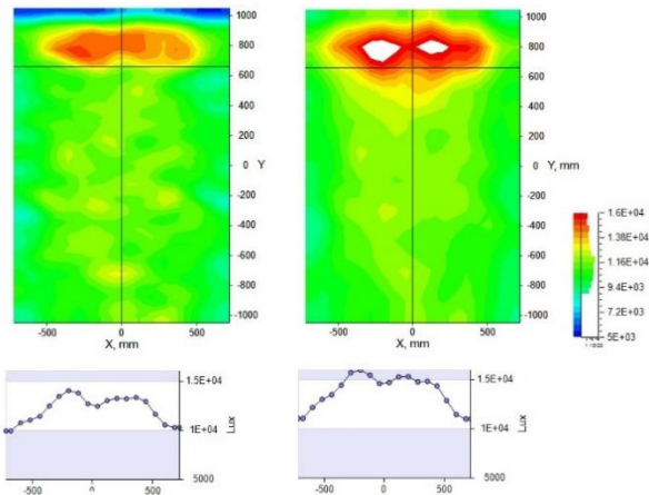
Figure 5: Illuminance map on the vertical reference plane for a shading system with Z-shaped slats (left) and Z-shaped slats with a specular tip (right) (Phase 3)
