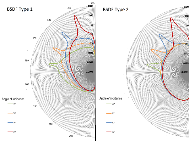
Figure 3: BSDF data for two typical slat types measured at incidence angles of 10°, 30°, 50° and 70° (The radial axis has a logarithmic scale)
