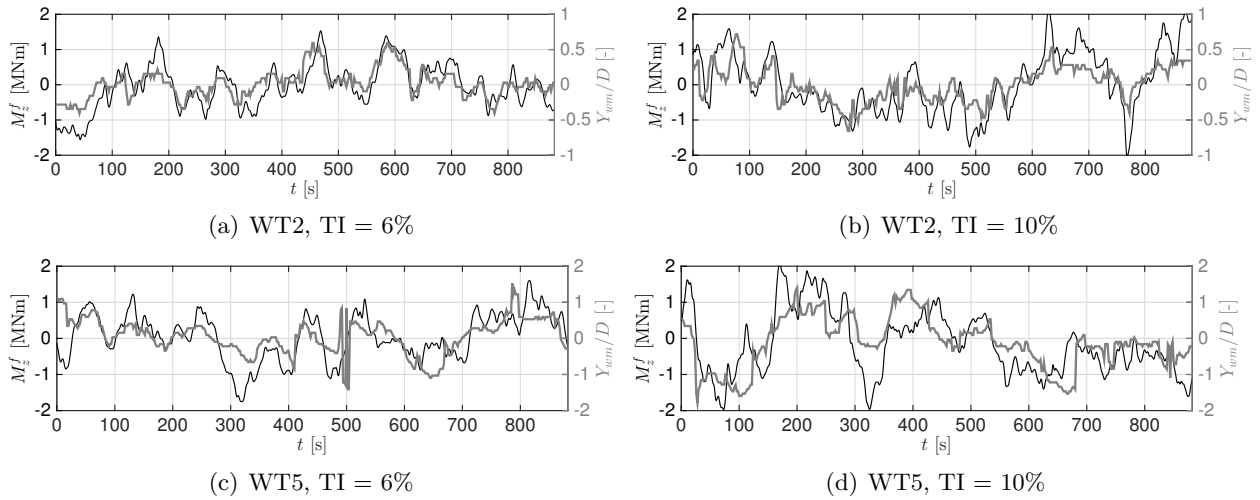
Figure 3: Comparison between the wake centerline position just upstream of WT _i (solid grey line) and the resulting filtered yaw moment on WT _i (solid black line). Two wind turbines are studied, WT2 (top) and WT5 (bottom), for the two TIs (left : 6% and right, 10%)
