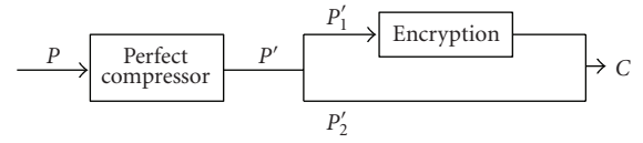
FIGURE 3: In perfect compression configuration, a subset of the bitstream can be encrypted; protected part is not predictable from the public one.
