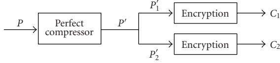
FIGURE 2: Fully layered system: the whole compressed bitstream is encrypted.
