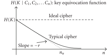
FIGURE 1: Key equivocation function.
