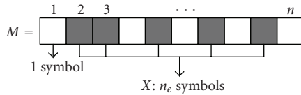
FIGURE 7: Selectively encrypting a message M , only gray units are encrypted.
