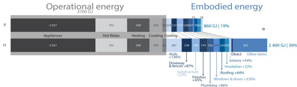
Figure 2: Life cycle energy of case study house based on process (P) and hybrid (H) analysis, by use.
