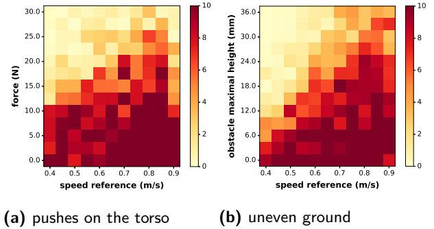
Figure 13. For the whole spectrum of speed references, COMAN faced two kinds of external disturbances. In panel (a), pushes were applied on its torso (Experiment 6). The color map represents the number of pushes the robot resisted (averaged over five runs) before falling, as a function of the pushes amplitude. In panel (b), COMAN was walking on the irregular ground displayed in Figure 17 (Experiment 9). The values of the corresponding H_i heights were randomly selected in the range whose maximum value is reported on the vertical axis. The color map represents the forward distance (i.e. along the x axis [m] ) COMAN walked before falling (limited to 10\text{ m} and averaged over five runs).
