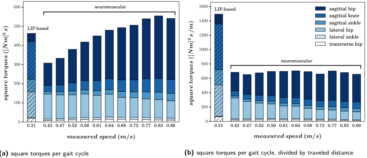
Figure 12. Estimate of the energetic consumption of both controllers tested in Experiment 5. Panel (a) reports the sum of square of the joint torques for the LIP-based controller (hatched) and the neuromuscular one (non-hatched), both integrated over one gait cycle, i.e. one stride. The measures were performed on the right leg at different speeds, and averaged over 20 gait cycles. The contributions of each joint correspond to different colors (see legend). Panel (b) displays the same result, normalized by the distance traveled during one gait cycle.
