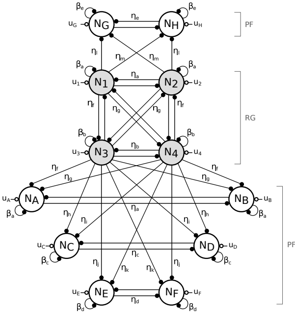
Figure 4. Full CPG network inter-neuron excitations are indicated with an empty circle, while plain circles represent inhibitions. The "rhythm generator" neurons (RG, shaded) affect the "pattern formation" ones (PF), but not vice versa. The corresponding CPG equations are provided in Appendix C.
