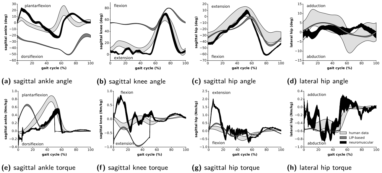
Figure 9. Kinematic and dynamic profiles of Experiment 5: the human data from (Bovi et al., 2011) (natural speed) is compared to our neuromuscular controller ( 0.75 \text{ m/s} ) and to the LIP-based controller ( 0.31 \text{ m/s} ) from (Faraji et al., 2014). The averages of the different measures are displayed over one gait cycle (starting at right foot strike), augmented by their standard deviations (shaded areas).
