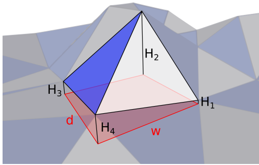
Figure 17. Description of the irregular uneven ground generated for Experiment 9. Each triangle composing the ground mesh is based on a rectangle of size d \times w with four randomly selected heights H_i at its corners ( d = w = 50 \text{ cm} ).
