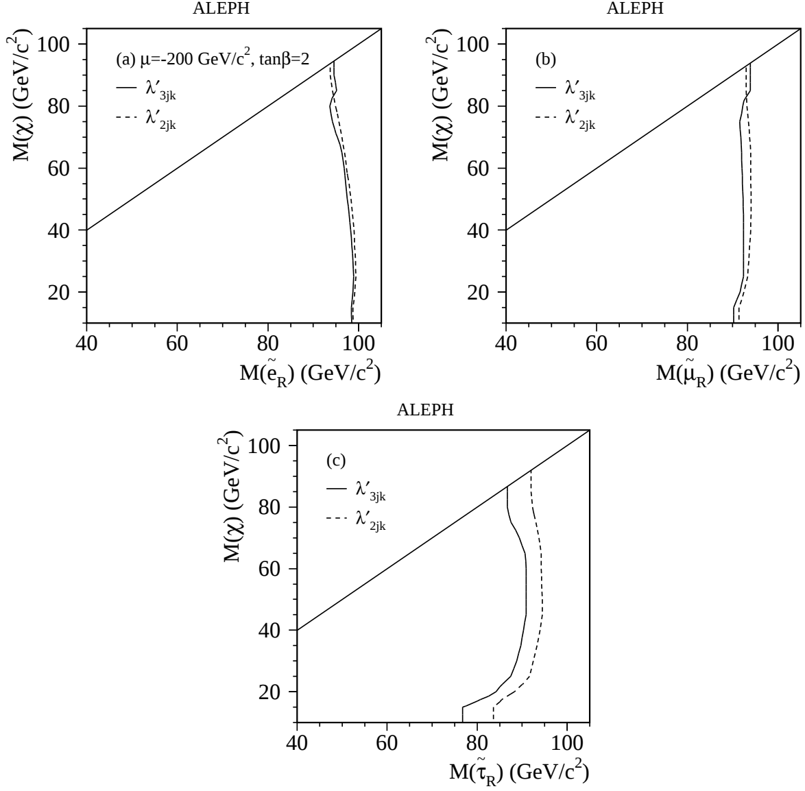
Figure 10: The 95% C.L. limits in the (m_\chi, m_{\tilde{\ell}_R}) plane for (a) selectrons, (b) smuons and (c) staus decaying indirectly via a dominant LQ\bar{D} operator. The two choices of \lambda'_{2jk} and \lambda'_{3jk} correspond to the most and least stringent exclusions, respectively. The selectron cross section is evaluated at \mu = -200 \text{ GeV}/c^2 and \tan\beta = 2 . The limit from the \Gamma_Z measurements excludes m_{\tilde{\ell}} < 38 \text{ GeV}/c^2 .
