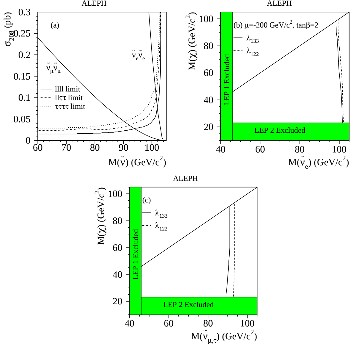
Figure 6: (a) The 95% C.L. cross-section upper limits for sneutrinos decaying directly via a dominant LLE\bar{E} operator. The three curves correspond to different possible final states, with \ell = e or \mu , due to the specific choice of sneutrino flavour and \lambda_{ijk} . The MSSM cross section for pair production of muon and electron sneutrinos are superimposed; the tau sneutrinos have the same cross section as the muon type. The 95% C.L. limits in the (m_\chi, m_{\tilde{\nu}}) plane for \tilde{\nu}_e (b) and for both \tilde{\nu}_\mu and \tilde{\nu}_\tau (c) indirect decays. The two choices of \lambda_{122} and \lambda_{133} correspond to the most and least stringent exclusions, respectively. The electron sneutrino cross section is evaluated at \mu = -200 GeV/c 2 and \tan\beta = 2 .
