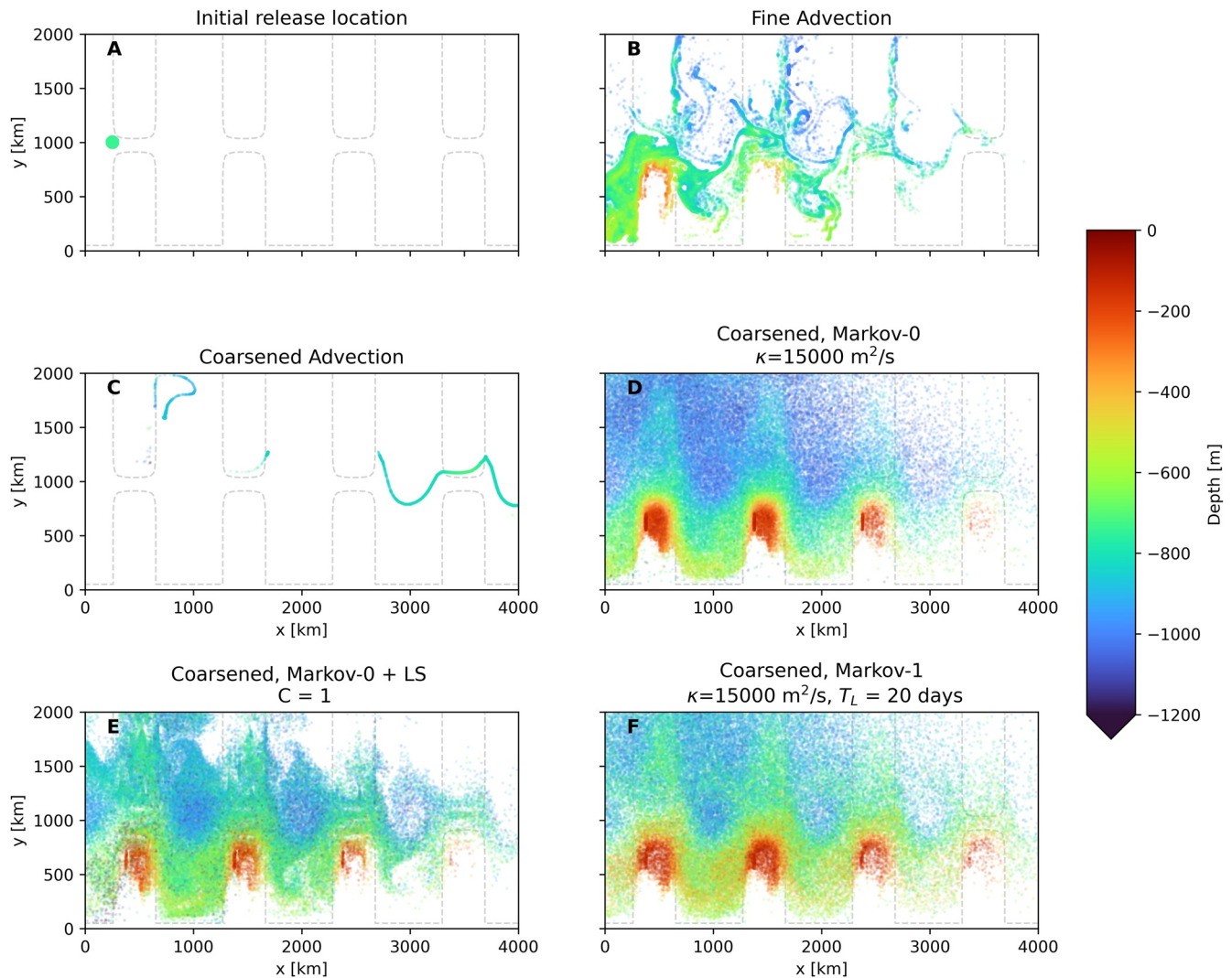
Figure 10. (a) Initial particle positions at z = -736 \text{ m} , (b–f) show particle locations and depths after 180 days of simulation with \Delta t = 40 \text{ min} (b and c) show particles advected with the fine-resolution and coarsened model fields, while (d–f) use the diffusion/Markov-0 and Markov-1 models. Particles that fall within the mixed layer are not shown (see Appendix B).
