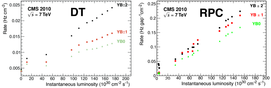
Figure 38. Left: the DT background rates vs. LHC luminosity for the barrel wheels (YB0 is closest to the IP, YB±2 are farthest away). Right: the RB backgrounds vs. luminosity for the barrel wheels. The patterns are similar, increasing as the distance from the IP increases. The difference in rates occurs, in part, because the RB rates are maximum rates whereas the DT rates are averages.
