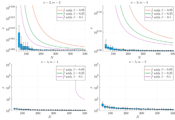
Fig. 1. Boxplots of the ratio \bar{r} defined in (6) for different dimensions n and data sizes N = |\mathcal{D}| . For each n , a different randomly generated system with m := |\mathcal{A}| = n matrices was used. For a given n and for each N , the boxplots were obtained by running 32 experiments, with different randomly sampled data sets \mathcal{D} . We also represented the bound \tilde{f} := f(\beta, \delta^{(n-1)/2}, N, d, \alpha, n) on the inflation factor \tilde{f} for different values of \beta , and for \delta = 5 and \alpha = 1/m . For the bottom plots, some curves are not visible because their value is so large ( > 10^4 ) that it is outside of the vertical range.
