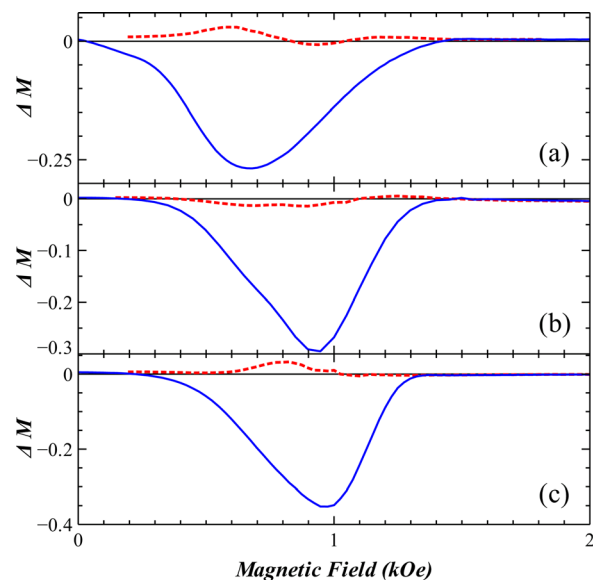
FIG. 7. \Delta M plots obtained from the as-measured (continuous line) and corrected (dashed line) IRM and DCD remanence curves, for samples (a) S1 [Ni], (b) S5 [Co], and (c) S9 [NiFe].
