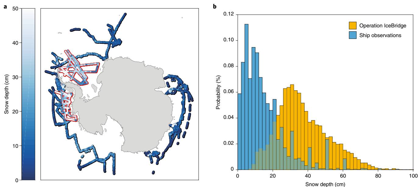
Fig. 3 | Antarctic snow depth distributions. a , September–November (austral spring) snow depth distributions on Antarctic sea ice based on ship observations 51 (black outline) and from Operation IceBridge aerial surveys 86 (red outline). The deeper snow depth retrievals from Operation IceBridge may result from greater sampling of thicker, more deformed ice later in the season relative to the ship-based observations (which tend to avoid regions of thick/deformed ice). b , Snow depth distributions for September–November from ship observations and Operation IceBridge. The histogram excludes snow-free values from the ship observations (~10% of the total) for an objective comparison with the airborne data, which excludes snow-free values. The bin size is 2 cm.
