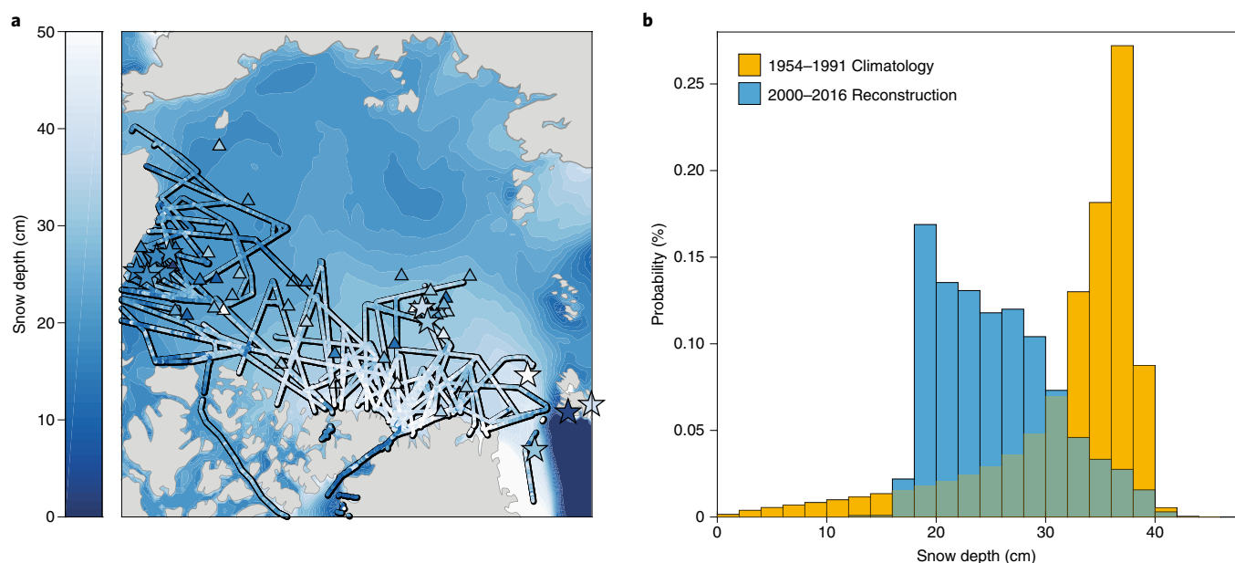
Fig. 2 | Arctic snow depth distributions. a , Snow depth reconstruction on Arctic sea ice in March–April 2000–2016 from ERA-Interim reanalysis snowfall 97 . Snow depth observations from different sources in 2000–2016 are overlaid: ice mass balance buoys 95 (triangles); mean snow depths from field campaigns (stars) and NASA Operation IceBridge aerial surveys (basin-scale lines) 85 . The Operation IceBridge retrievals exclude snow-free (zero) values. b , Snow depth distributions for March–April from the 1954–1991 climatology 20 and the 2000–2016 reconstruction, which show a marked reduction in depth. The bin size is 2 cm.
