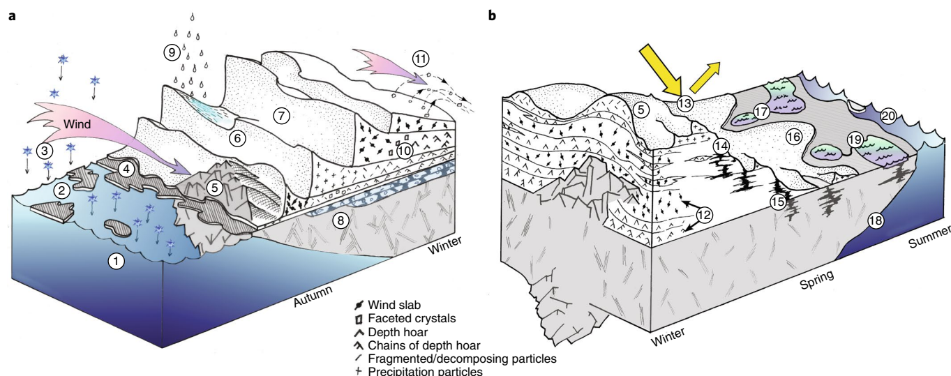
Fig. 1 | A schematic of the complex set of processes that takes place between snow and sea ice. a, Autumn to winter. b, Winter to summer. We exclude midwinter and mid-to-late summer from the illustrations to highlight the dominant snow processes. Box 1 contains the descriptions of the processes numbered in the figure. Certain processes are more dominant in one hemisphere than the other; for example, melt ponds in the Arctic, snow-ice formation in the Antarctic (see Box 1 and Sturm and Masson 1 ). Credit: Matthew Sturm
