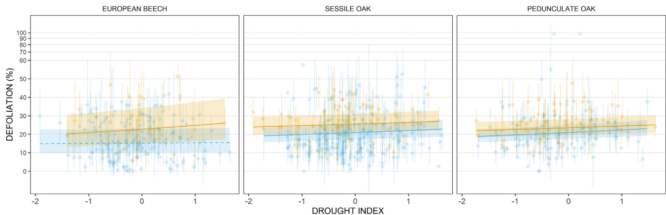
Fig. 2. Effect of drought index on crown defoliation in European beech, sessile oak and pedunculate oak in absence (blue) and presence (yellow) of insect damage. The raw data are represented by an average value of crown defoliation by plot (dots) and its standard deviation (vertical lines). Solid lines represent the crown defoliation of a tree predicted by the models after a back-transformation of the logarithmic values at an average value of stand density, N: P ratio and for a median year (2006). The line patterns indicate whether the slope of the relationship was significant (solid line) or not (dashed line). Shaded areas represent the confidence intervals to the regression lines at 95% (For interpretation of the references to colour in this figure legend, the reader is referred to the web version of this article.)
