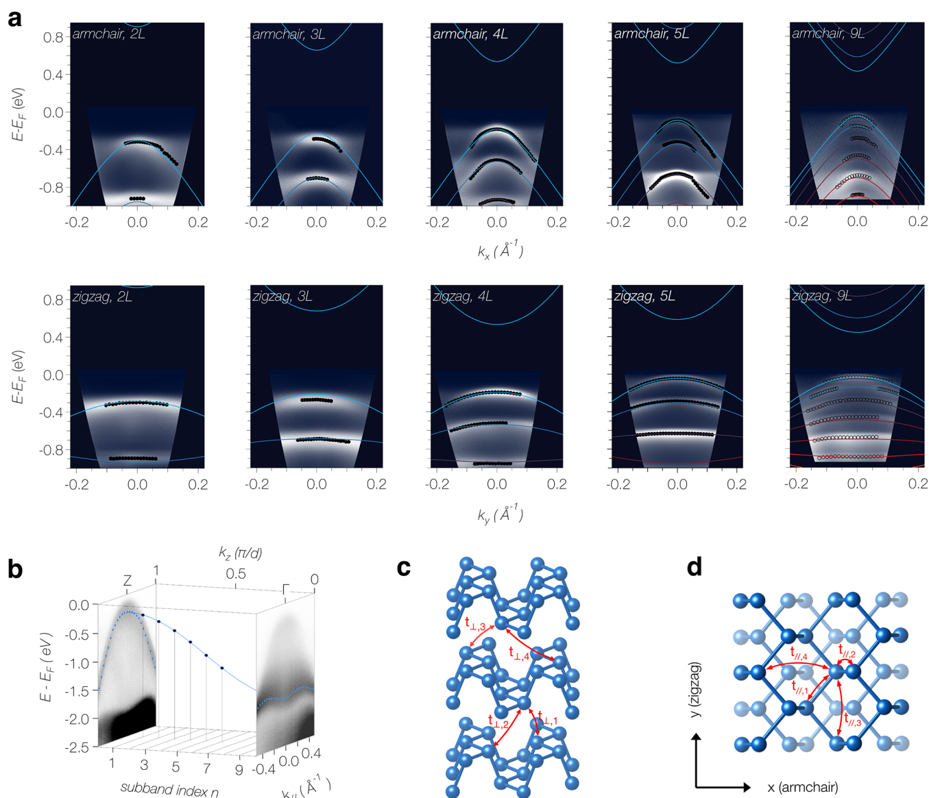
Figure 2. Subband dispersion in ultra thin mechanically exfoliated BP. (a) \mu -ARPES data of 2L–9L BP acquired at a sample plate temperature of T = 4.5 K with linearly polarized 6 eV light (see Methods ). Energies are relative to the Fermi level E_F . Solid colored lines are the result of a global tight-binding fit to subband energies extracted from 2L, 3L, 4L, and 5L data (filled black circles). For details, see main text and Supporting Information , section III. The same tight-binding model is overlaid on the 9L data (open black circles), which were not included in the fit. (b) Model of the subband energies for 9L BP. Gray scale plots show the in-plane dispersion of bulk BP along the zigzag direction measured at T = 50 K (to avoid charging) and photon energies of h\nu = 20.1 and 36.6 eV to select k_z near the Z- and \Gamma point of the bulk Brillouin zone. Blue symbols indicate the dispersion of the bulk valence band. The measured subband energies for 9L BP (black symbols) are well described by the bulk dispersion along \Gamma Z and the quantization condition for k_z introduced in the main text. (c,d) Structural model of BP with the 8 tight-binding parameters used in the fit.
