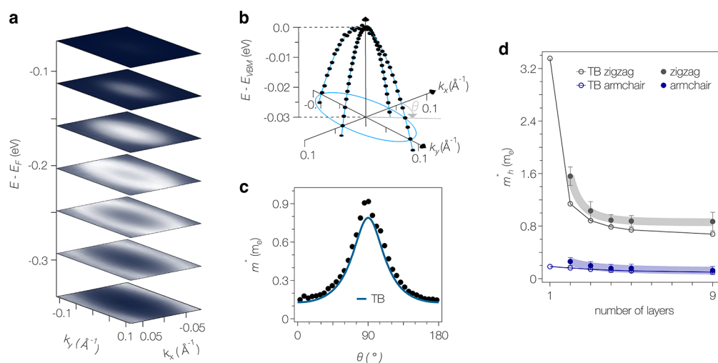
Figure 3. Dispersion and effective mass near the valence band edge. (a) Stack of constant energy contours of the topmost quantum well state in 4L BP. (b) Low-energy band dispersion extracted from curvature plots together with parabolic fits. (c) Anisotropy of the effective mass extracted from the 3D data set in (a) together with the angle dependence of the effective mass obtained from the tight-binding (TB) model. (d) Thickness dependence of the effective masses along both high-symmetry directions. Thick shaded lines are guides for the eye.
