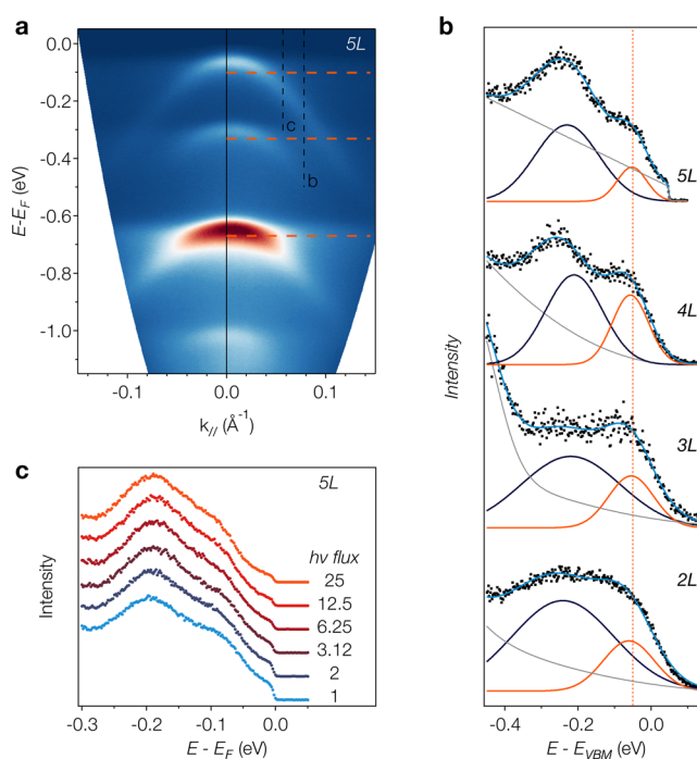
Figure 4. Dispersionless spectral features in few-layer BP. (a) ARPES data of 5L BP along the armchair direction shown without normalization of the intensities applied in Figure 2. (b) EDCs of the highest subband in 2L–5L BP showing a two-peak structure away from the \Gamma point at k_{\parallel} \approx 0.08 \text{ \AA}^{-1} , indicated by a dashed line in (a). (c) EDC at position c indicated in panel (a). The photon flux relative to the first spectrum is indicated in the figure. No significant variation of the spectral line shape is detected when varying the photon flux over more than an order of magnitude.
