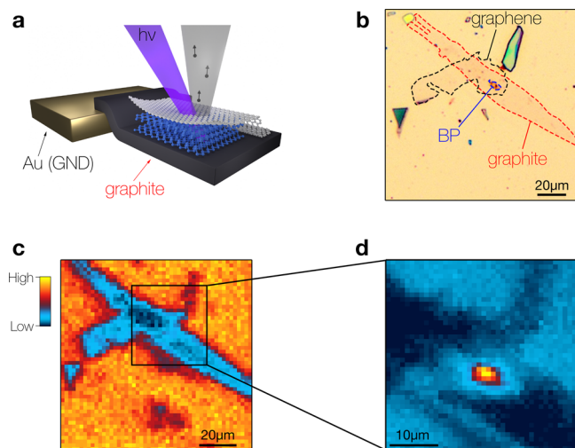
Figure 1. Concept of the laser \mu -ARPES experiments on few layer BP. (a) Schematic of the microfocus photoemission setup and of the graphene/BP/graphite heterostructures prepared for this study. (b) Optical micrograph of a \sim 3 \times 7 \mu\text{m}^2 few-layer BP crystal encapsulated in graphite/graphene and supported on a Au-coated Si/SiO 2 substrate. (c,d) \mu -ARPES photocurrent maps of the device shown in (b) acquired with linear polarizations of the light that (c) minimize and (d) maximize emission from BP.
