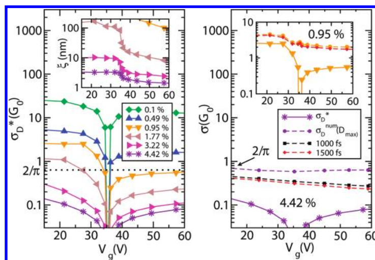
Figure 3. Left panel: \sigma_D^*(V_g) (main frame) of chemically-modified graphene for several epoxide-defects densities n_i = 0.1 – 4.42\% . Right panel: Kubo conductivities for n_i = 4.42\% (main frame) and n_i = 0.95\% (inset) at different elapsed computational times. \sigma_D^*(V_g) at n_i = 4.42\% is also given for comparison. The localization lengths computed using \xi(E) = \ell_e \exp(\pi\sigma_D^{\text{num}}(E)/2G_0) are also given (left panel, inset).
