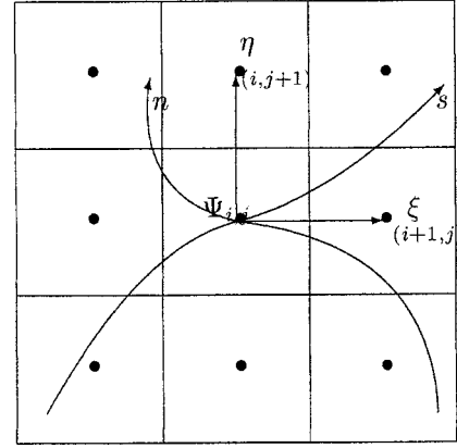
FIG. 1. Grid and naming convention.
