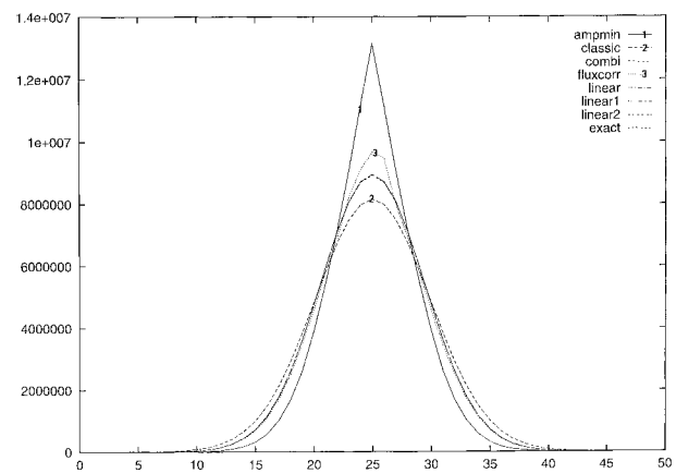
FIG. 21. Integral on \eta in the function of the grid point; the exact solution is indistinguishable from the linear solutions. AMPMIN not only shows the reduced diffusion as before but also the effect of the inconsistent flux calculations, which allow an unphysical peak in the integrated field to remain. FLUXCORR has a slightly higher peak than the exact solution, while the CLASSIC method reduces the peak.
