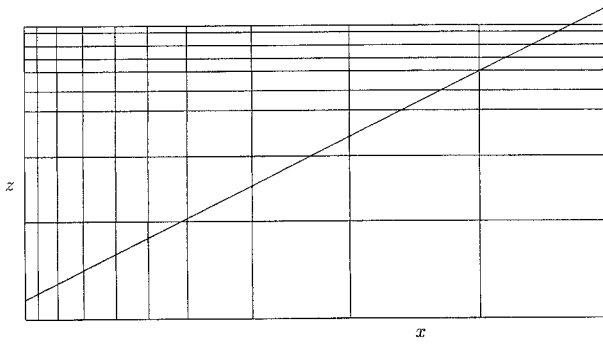
FIG. 2. Representation of an isopycnal line in physical space, with a numerical grid superimposed. Depending on the discrete grid, the isopycnal line can significantly change its vertical position relative to the numerical grid from one horizontal grid point to the next.
