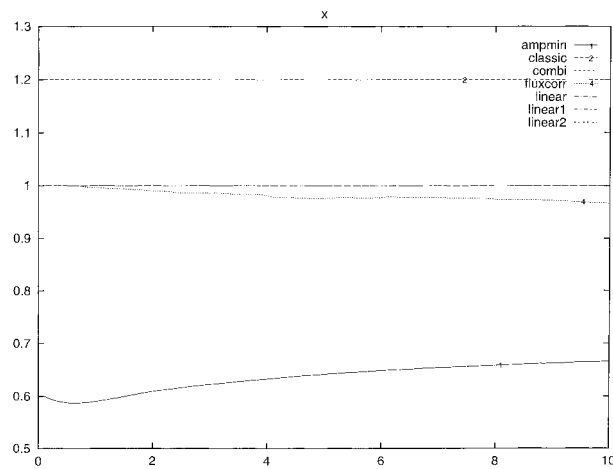
FIG. 18. Evolution of the measure of the horizontal diffusion. AMPMIN clearly reduces diffusion while increasing the horizontal background diffusion by 20% in CLASSIC can clearly be seen on this integral quantity. All linear schemes have the correct average horizontal diffusion while FLUXCORR slightly reduces it.
