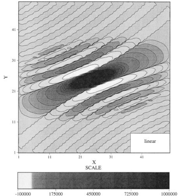
FIG. 9. Linear scheme LINEAR. Diffusion of a Dirac signal along y = 0.4x after 100 time steps. This standard scheme clearly introduces strong diapycnal diffusion and dispersion with significant under-shootings (in white).
