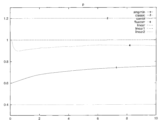
FIG. 20. Evolution of the measure of the direction of the diffusion. Consistently with the analysis of the horizontal and vertical diffusion, the average direction of diffusion is correct for the linear schemes, too flat for the CLASSIC scheme and slightly more upward oriented for the FLUXCORR scheme. AMPMIN and COMBI modify the direction very strongly.
