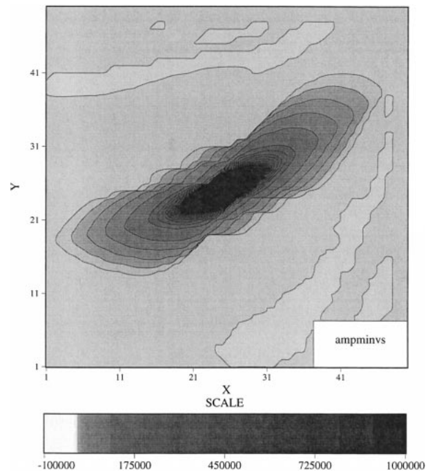
FIG. 23. AMPMIN method for the variable slope experiment showing that the diffused field follows the density field by bending the patch along the isolines.
