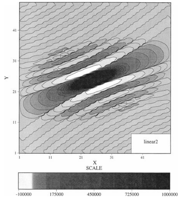
FIG. 11. Second modified linear scheme LINEAR2. The solution is very similar to the standard solution in this case with a slightly reduced propagation of information into the diapycnal direction.
