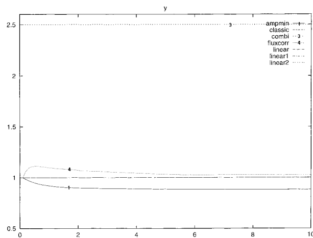
FIG. 19. Evolution of the measure of the vertical diffusion. As for the horizontal diffusion, AMPMIN reduces the diffusion, and the linear schemes behave correctly. The FLUXCORR method slightly increases the vertical diffusion while the inconsistent COMBI method shows the strong additional vertical diffusion consistent with the analysis of the numerical stencil.
