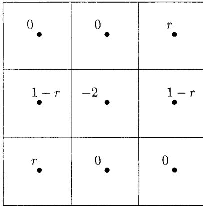
FIG. 7. Stencil for the inconsistent linear method COMBI. A slope parameter r \in [0, 1] was assumed. For the sake of clarity, no multiplication constant was included.
