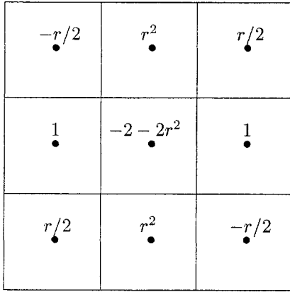
FIG. 3. Stencil for the standard LINEAR discretization in the case of constant slopes and grid spacings. For the sake of clarity, no multiplication constant was included. We assume that we reference fluxes and points compared to the central point of the control volume, whose coordinates are thus i, j . For fluxes, when they are not referenced by coordinates, they correspond to either the interface i + 1/2, j or i, j + 1/2 .
