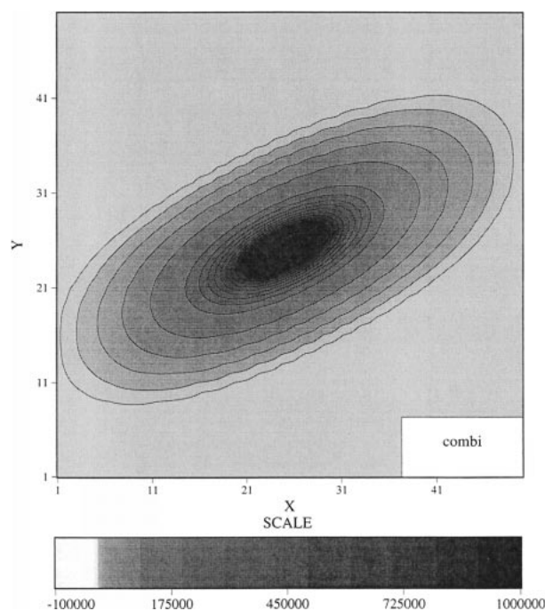
FIG. 13. Inconsistent combination of horizontal and diagonal diffusion COMBI. Clearly the diapycnal dispersion was replaced by a diapycnal diffusion ensuring a monotonic solution that propagates strongly in the diapycnal direction.
