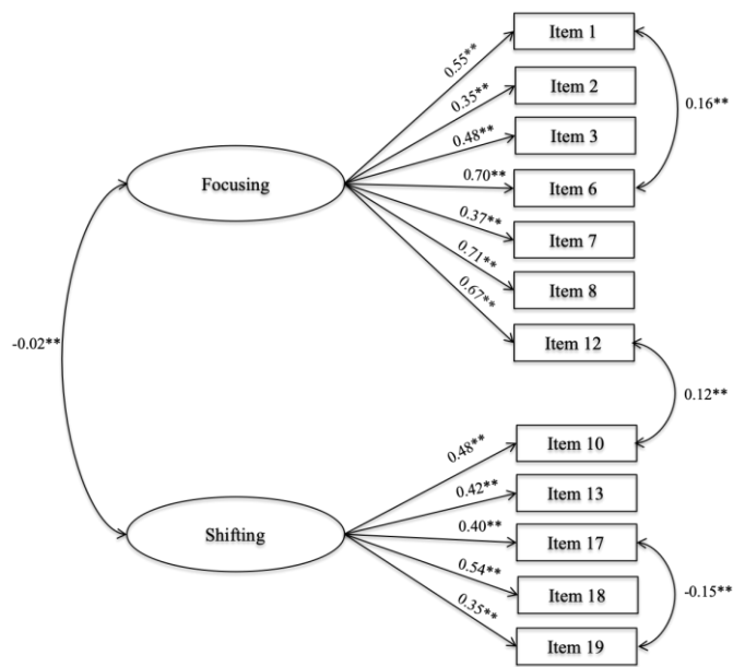
Figure 2. Path diagram depicting the two-factor solution (model 3 corrected) of the French version of the Attentional Control Scale.
