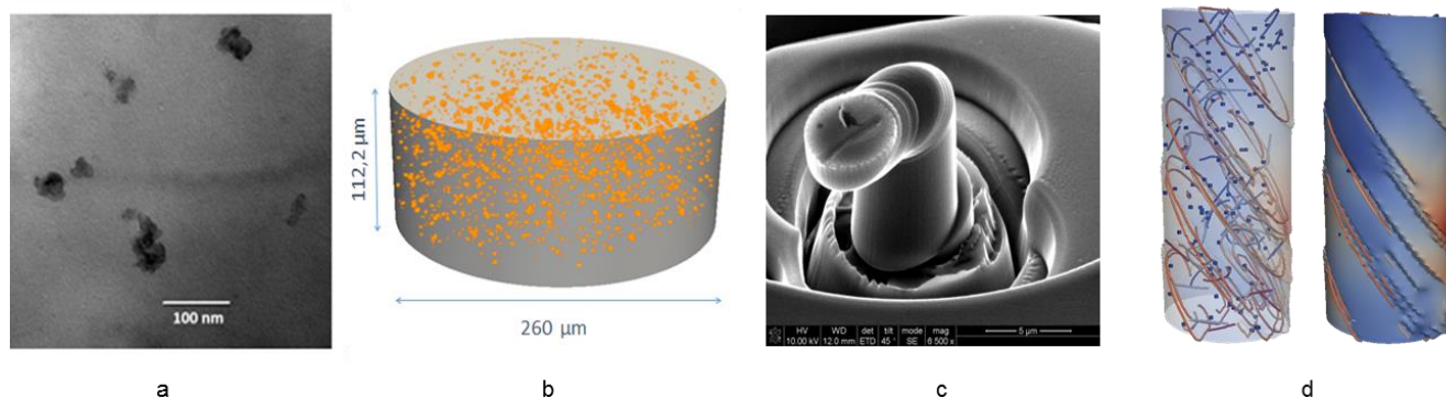
Figure 1 - TEM micrograph showing the Y 2 O 3 particles in the FSPed sample (a). Synchrotron X-ray microtomography confirms the homogeneous dispersion of particles (b). Post-compression structure (c). 3D dislocation dynamics simulations of a micropillar ( \varnothing=10 \mu m and h=25\mu m) with cubic particles ( f_v=0.1\% and \varnothing=250 nm) (d).
