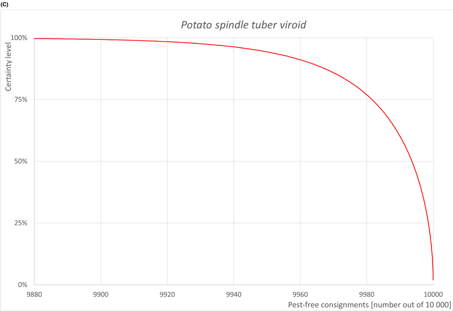
FIGURE A.9 (A) Elicited uncertainty of pest infection per 10,000 bags (containing 105 unrooted cuttings per bag) for potato spindle tuber viroid (histogram in blue – vertical blue line indicates the elicited percentile in the following order: 1%, 25%, 50%, 75%, 99%) and distributional fit (red line); (B) uncertainty of the proportion of pest-free bags per 10,000 (i.e. = 1 – pest infection proportion expressed as percentage); (C) descending uncertainty distribution function of pest infection per 10,000 bags.
