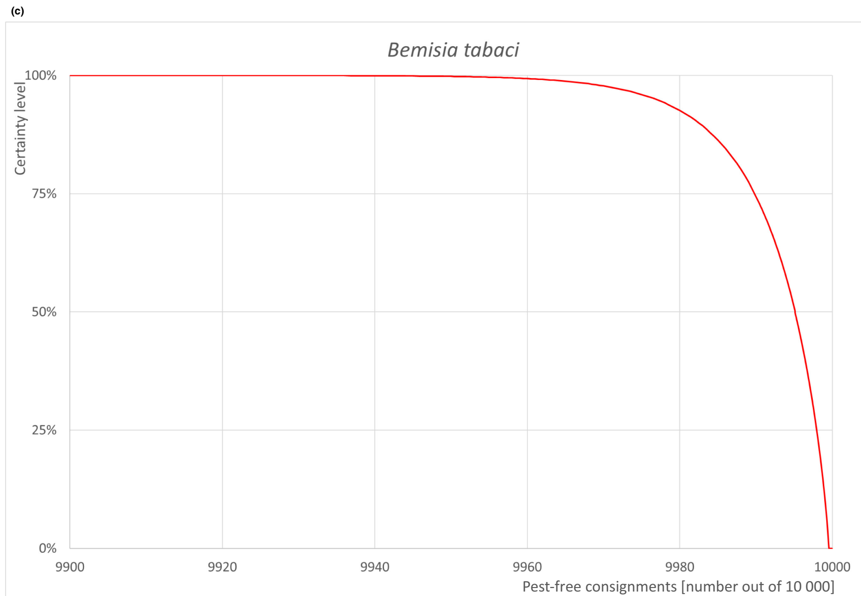
FIGURE A.3 (A) Elicited uncertainty of pest infestation per 10,000 bags (containing 105 unrooted cuttings per bag) for B. tabaci (histogram in blue – vertical blue line indicates the elicited percentile in the following order: 1%, 25%, 50%, 75%, 99%) and distributional fit (red line); (B) uncertainty of the proportion of pest-free bags per 10,000 (i.e. = 1 – pest infestation proportion expressed as percentage); (C) descending uncertainty distribution function of pest infestation per 10,000 bags.
