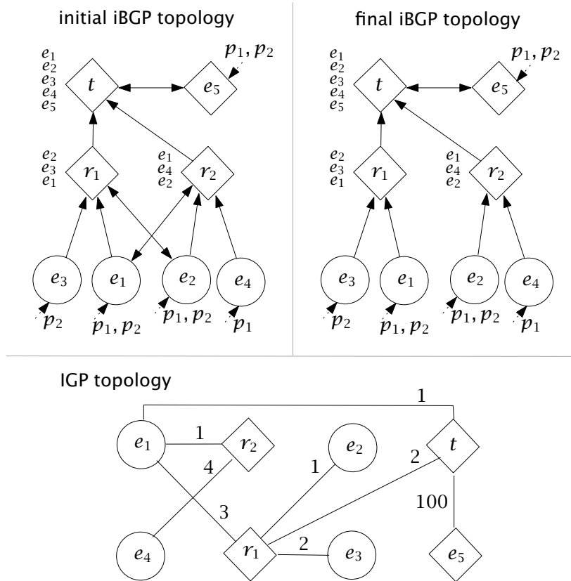
Figure 6.8 Pyramid gadget, an iBGP topology change case in which unintended traffic shifts occur in every reconfiguration ordering.
