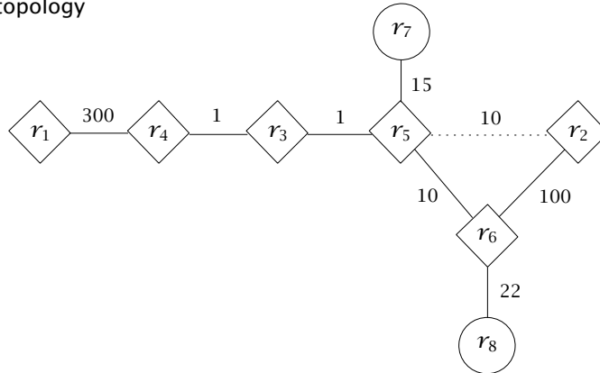
Figure 7.5 The horizontal gadget. Migrating the IGP on a per-destination basis does not guarantee the absence of BGP-induced forwarding loop. In this reconfiguration scenario, r_2 is the considered destination and contradictory reconfiguration constraints exist between r_5 and r_6 .
