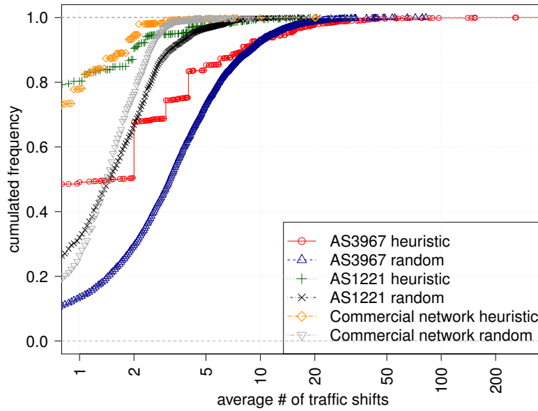
Figure 4.2 Cumulative distribution function (CDF) of the average amount of traffic shifts created between each pair of routers when performing the migration by increasing the AD of the initial protocol.
