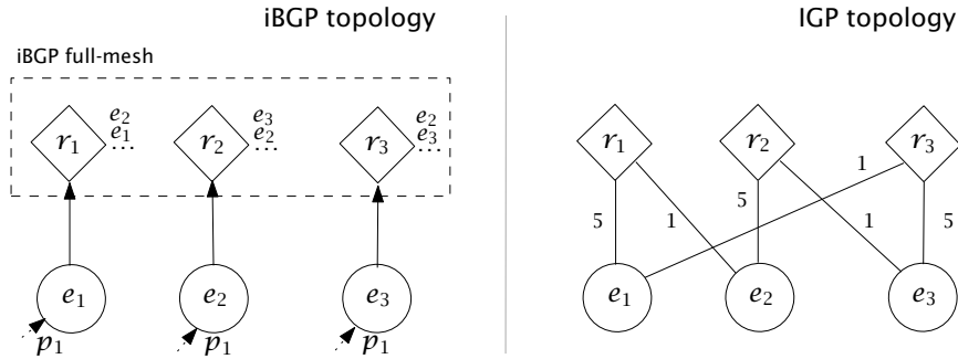
Figure 5.2 An example of BGP configuration in which no stable solution exists (taken from [66]).
