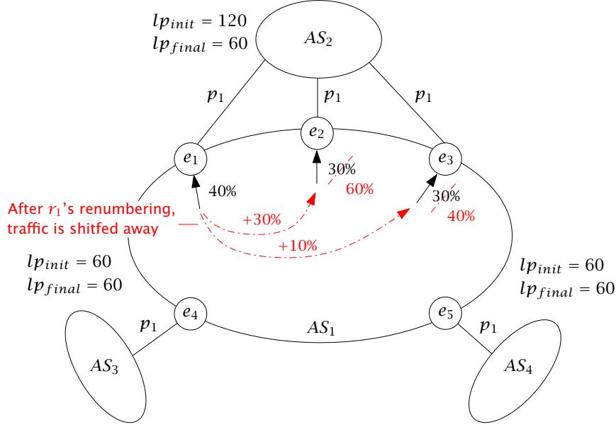
Figure 6.3 Lowering the LP applied on the eBGP sessions with s_2 (e.g. due to a change of the peering agreement) triggers significant traffic shifts. Here, 40% of the traffic destined to p_1 transiently shifts to e_2 and e_3 after having lowered the local-preference of e_1 .
