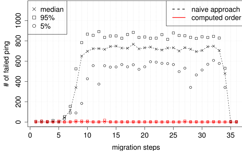
Figure 3.13 Our system guarantees that no packet is lost during migration while long-lasting connectivity disruptions can happen with a naive approach.
