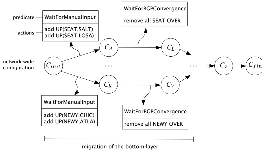
Figure 8.2 Snapshot of a migration graph.
