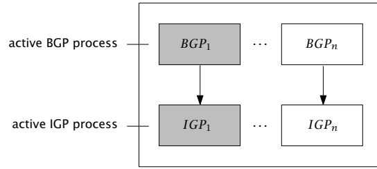
Figure 7.12 Abstract view of a combined ships-in-the-night framework. To gracefully accommodate combined reconfiguration scenarios, ships-in-the-night techniques should be available at any levels. Also, it should be possible for a protocol A depending on a protocol B to choose which instance of B it wants to depend on.
