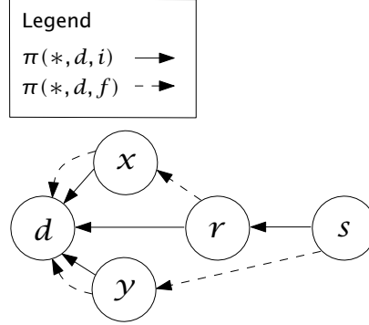
Figure 2.4 Example of a LS to LS reconfiguration in which a traffic shift occurs during the migration if r is migrated before s as the actual path of s becomes \pi(s, d, t) = (s \ r \ x \ d) which corresponds neither to the initial path, nor to the final one.
