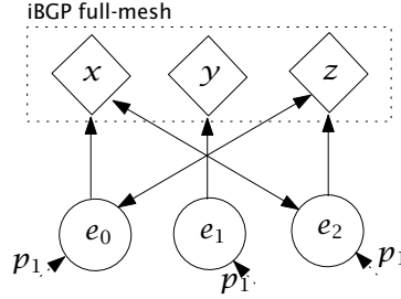
Figure 5.7 Spurious OVER can create forwarding loops.
