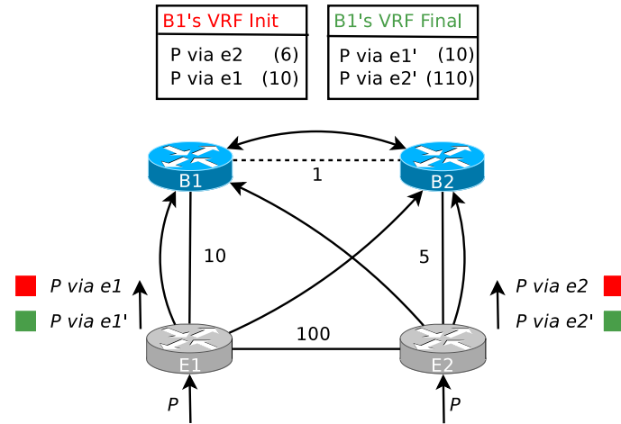
Figure 7.13 Extension of the reconfiguration framework to support for combined reconfigurations. To make two different BGP namespaces (i.e. VRFs) depend on two different IGPs, BGP next-hops can be rewritten according to the namespace such that each next-hop is only reachable via a particular IGP. In this flat2hierarchical reconfiguration, e1 and e2 are only reachable via the initial IGP and will be set as next-hops for the routes announced in the initial namespace. Similarly, e1' and e2' are only reachable via the final IGP and will be set as next-hops for the routes announced in the final namespace.
