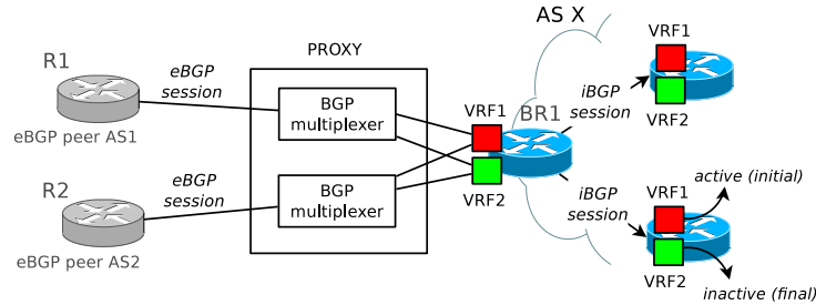
Figure 6.11 Architecture of our solution.
