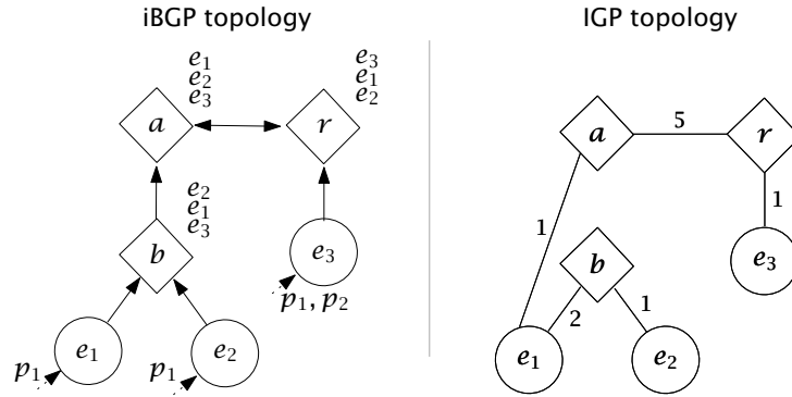
Figure 5.4 An example of BGP configuration which exhibits visibility issues. Indeed, a prefers e_1 , but it never learns the route since b only reflects e_2 .
