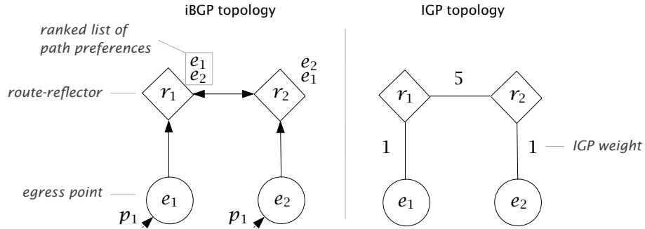
Figure 5.1 Graphical notations used in the thesis when referring to an iBGP configuration
