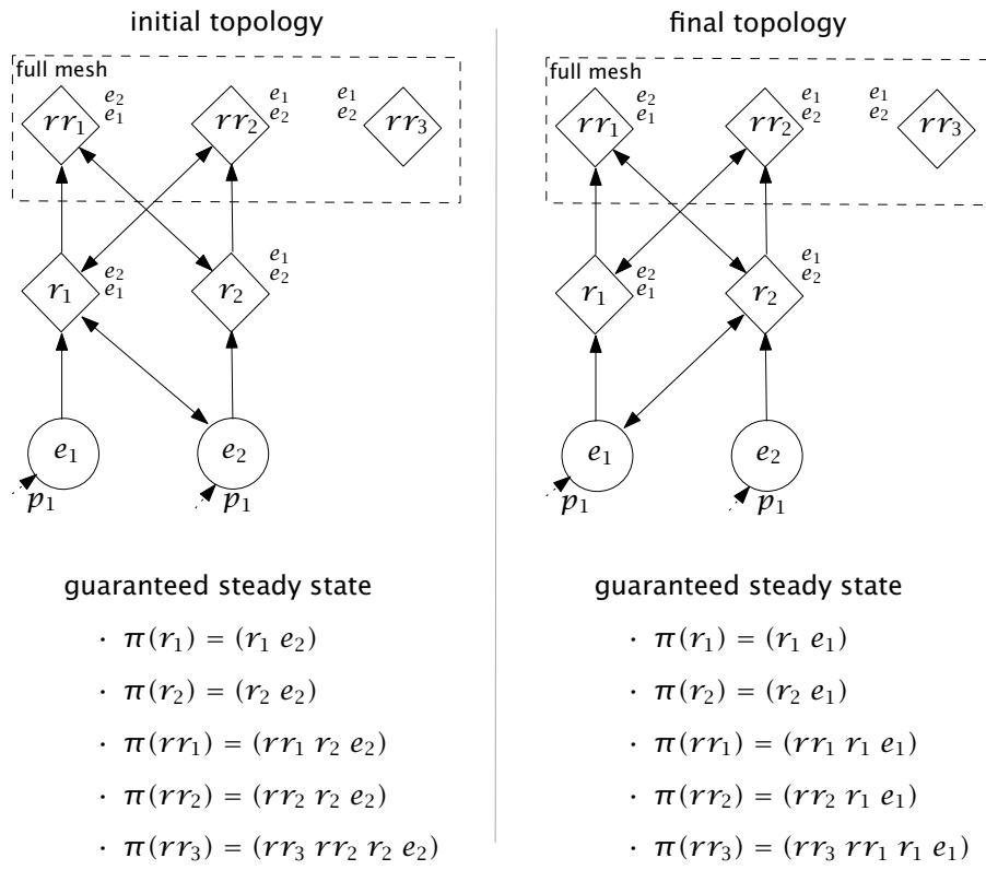
Figure 6.6 Double-Cross gadget.
