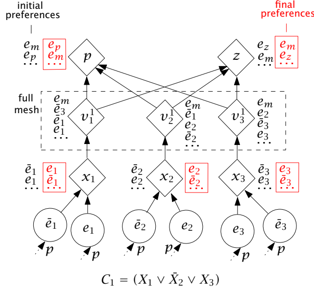
Figure 7.11 Example of the translation of a 3-SAT clause.
