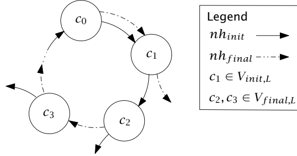
Figure 3.6 Abstract representation of a migration loop.
