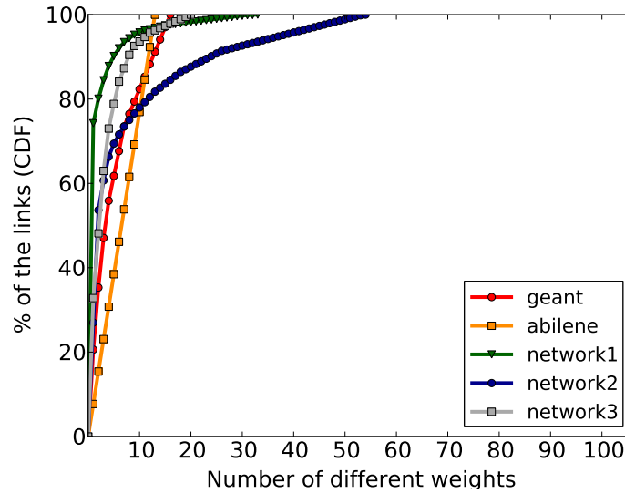
Figure 3.17 A few number of weights account for the majority of the links.
