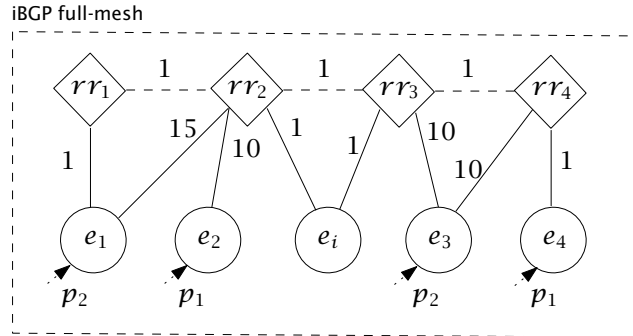
Figure 7.4 Roller-Coaster Gadget. Migrating the IGP can create migration loops that cannot be avoided at the BGP-level even when a full-mesh of iBGP session is used.
