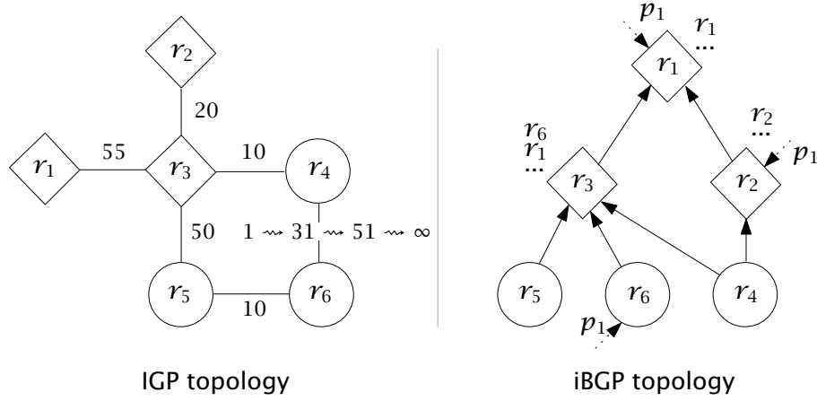
Figure 7.9 Scissors gadget. Applying the metric-increment technique to avoid transient IGP loops cause forwarding loops to BGP destinations.
