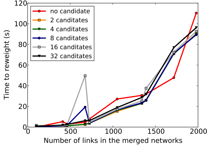
Figure 3.19 All networks can be reweighted in less than 2 minutes.
