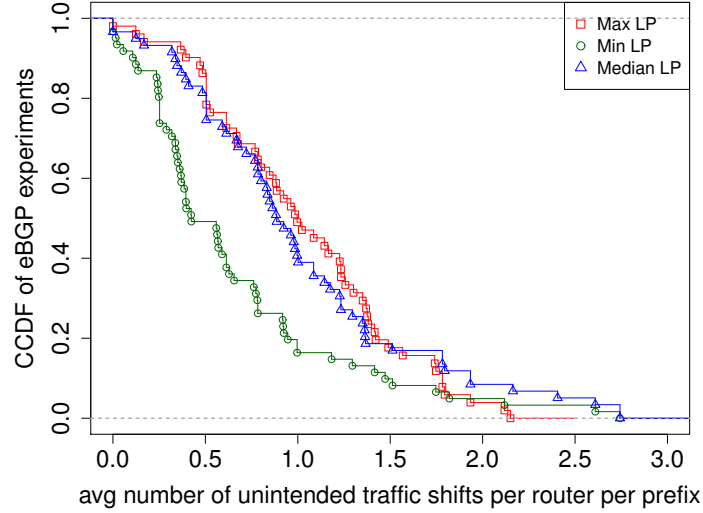
Figure 6.4 Average number of next-hop changes per-prefix each router in a Tier-1 sees during the modification of the LP attribute of all the eBGP sessions with a neighboring AS.
