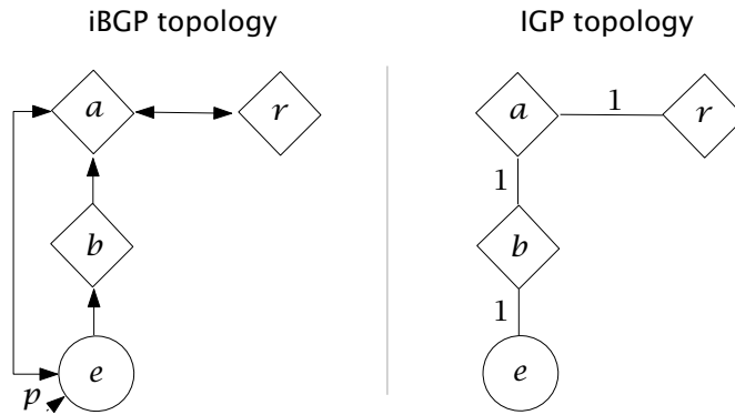
Figure 5.5 The OVER-RIDE gadget. Due to iBGP propagation rules, a does not propagate routes that it receives on its OVER session with e to r . Consequently, r ends up without any route to e while a valid signaling path exists: (e \ b \ a \ r) .
