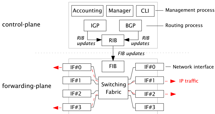
Figure 1.1 Sketch of an IP router. Modern IP routers are divided in two dedicated planes: the control-plane , in charge of IP routing, and the forwarding-plane , in charge of IP forwarding.
