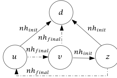
Figure 3.8 In some migration scenarios, the Routing Trees Heuristic generates unnecessary constraints.
