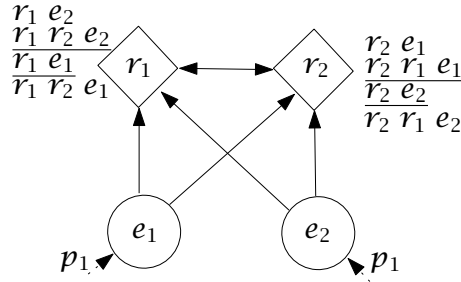
Figure 5.8 Redundant topologies hardly satisfy the prefer-client condition.
