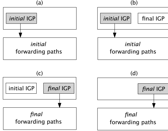
Figure 2.2 Details of the SITN IGP reconfiguration of one router. (a) The initial IGP configuration is the only one dictating the forwarding paths being used. (b) The final IGP configuration is then introduced in another IGP process. (c) Once the final IGP has converged, the preference is given to the final IGP so that it starts dictating the forwarding paths being used. (d) Once all routers have been migrated, the initial IGP is removed as it is not used anymore.
