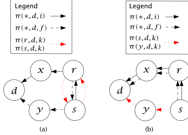
Figure 2.3 Abstract examples of (a) a forwarding loop and (b) a traffic shift.
