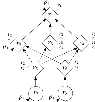
iBGP topology
