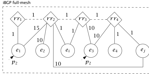
Figure 7.3 Divorce Gadget. No combined migration ordering is loop-free for flat2hierarchical scenarios even if there exists a safe ordering at the IGP and at the BGP level.
