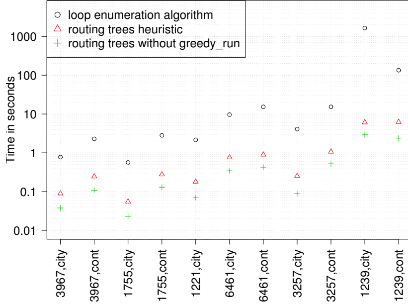
Figure 3.12 Time taken to compute an ordering in flat2hier (Rocketfuel topologies). Results for other scenarios are similar.
