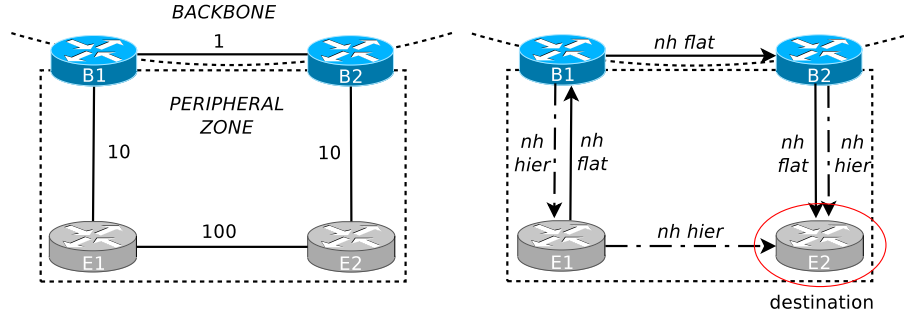
Figure 3.1 Bad Square Gadget. When the IGP hierarchy is modified, B1 starts preferring intra-zone path and forwards traffic destined to E2 via E1 . Since initially E1 forwards traffic destined to E2 to B1 , E1 must be migrated before E1 to avoid forwarding loops.
