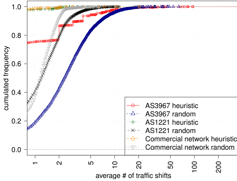
Figure 4.6 CDF of the average amount of traffic shifts created between each pair of routers when performing the migration by removing the initial protocol. Results for other scenarios are similar.
