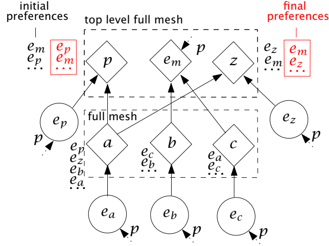
Figure 7.10 Basic structure for our reduction.
