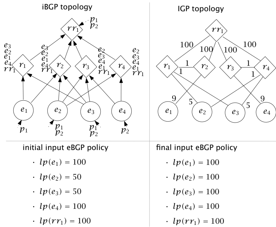
Figure 6.9 Carousel gadget, an eBGP policy reconfiguration case in which forwarding loops occur in every reconfiguration ordering.
