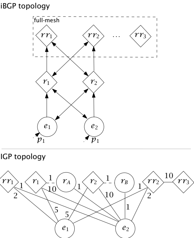
Figure 7.7 Heavy-Cross gadget, an IGP reconfiguration scenario (flat2hierarchical) in which a dissemination-free reconfiguration ordering does not exist.
