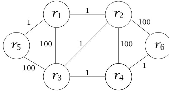
Figure 4.3 Shifty gadget. In this DV2LS reconfiguration scenario, no per-router ordering is free from traffic shifts. In particular, migrating any of r_1, r_2, r_3 or r_4 creates at least one traffic shift.
