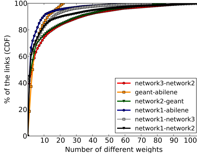
Figure 3.18 Translated weights exhibit similar distribution of the original ones.
