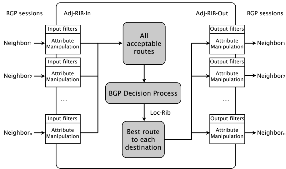
Figure 1.3 A schematic view of a BGP router. The Adj-RIB-In contains the BGP routes received from neighboring routers. The Loc-RIB contains the best route. The Adj-RIB-Out contains the BGP routes announced to neighboring routers.
