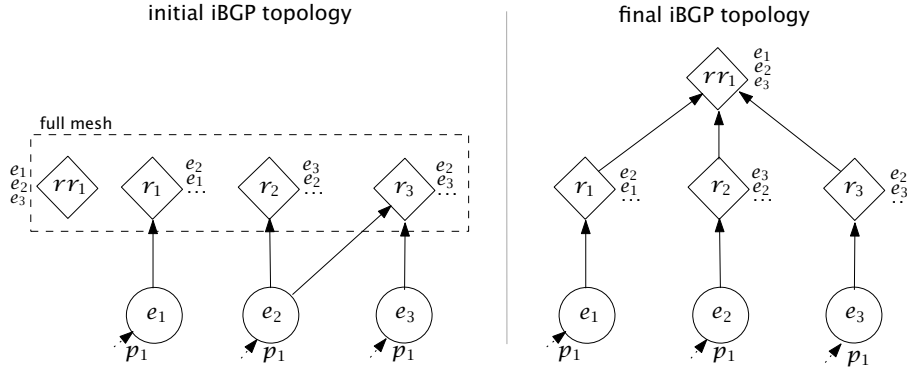
Figure 6.1 An example in which the bottom-up strategy, suggested by the current best practices, creates routing oscillations during the reconfiguration.
