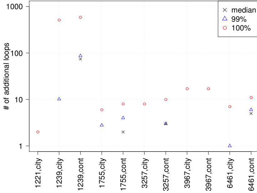
Figure 3.15 Average number of additional forwarding loops created by a single-link failure in flat2hier reconfiguration scenarios on Rocketfuel topologies. Missing points are equal to 0.
