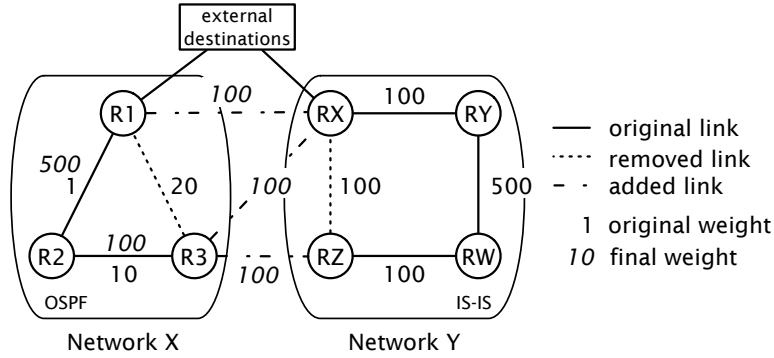
Figure 3.16 Merging scenario in which network X and Y are merged together
