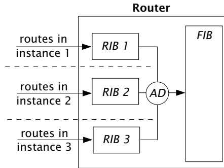
Figure 2.1 Model of a router running multiple IGPs. A specific routing table (RIB) is maintained for each protocol. The best routes of each protocol are installed in the router-wide forwarding table (FIB). When a route for a prefix p is available in more than one protocol, the one with the smallest AD is installed.
