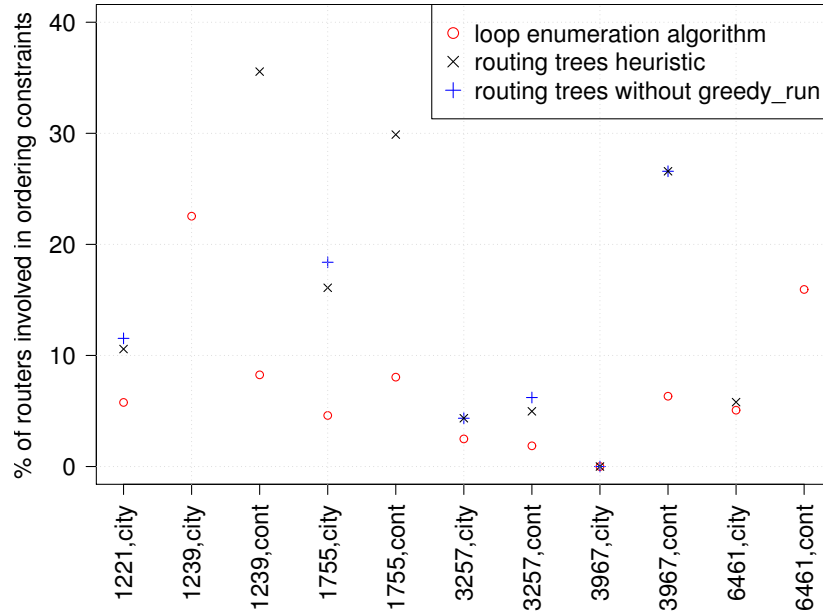
Figure 3.11 Percentage of routers involved in the ordering in flat2hier (Rocketfuel topologies). Results for other scenarios are similar.
