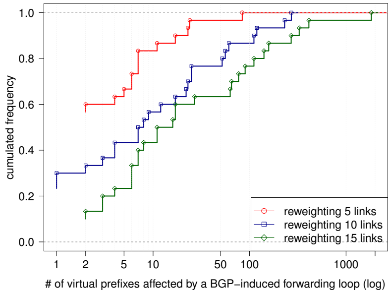
Figure 7.2 Numerous BGP-induced forwarding loops can appear during IGP changes, even when state of the art techniques are applied.
