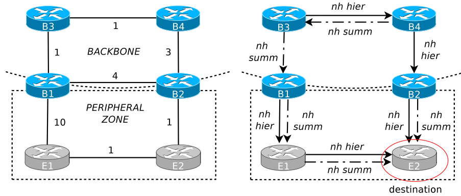
Figure 3.3 Route summarization gadget. When summarization is introduced or removed, a specific migration ordering is needed between B3 and B4 to avoid forwarding loops.
