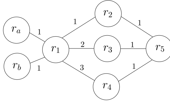
Figure 4.1 In this simple reconfiguration scenario, up to 36 traffic shifts can be created when replacing a DV IGP by the corresponding LS IGP.
