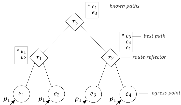
Figure 1.4 An iBGP route-reflection topology. With route-reflection, iBGP routers are hierarchically organized in clients and route-reflectors. Route-reflectors relay iBGP routes to and from their respective clients. Route-reflection also reduces the visibility of the BGP routes. In this topology, r_3 is only aware of the two routes announced by its clients while actually four routes are globally known.
