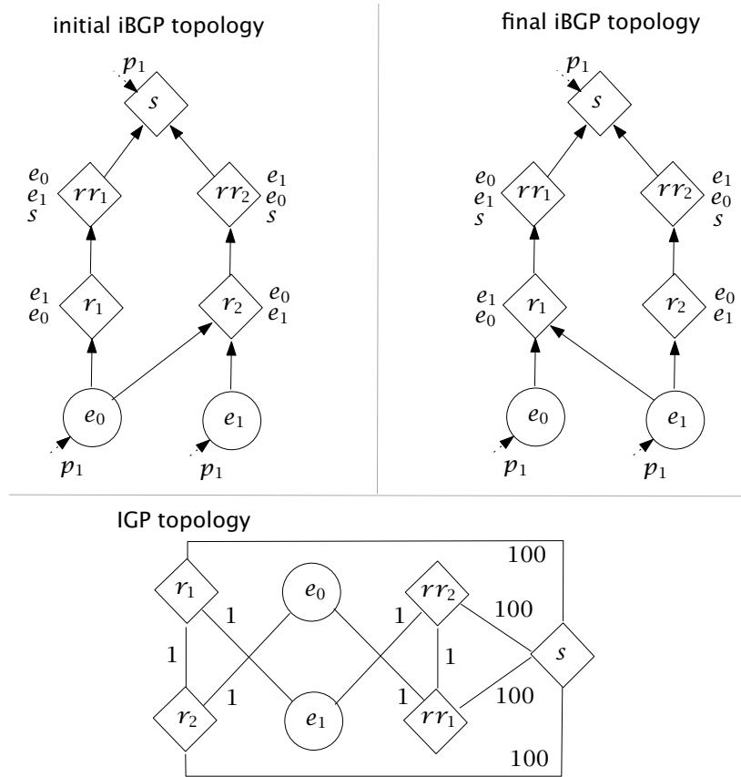
Figure 6.7 Pylon gadget, an iBGP topology change case in which a loop-free reconfiguration ordering does not exist.
