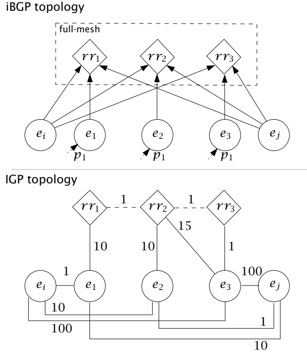
Figure 7.8 Go-With-the-Flow gadget. No IGP reconfiguration ordering can prevent BGP traffic shifts in intermediate configurations.
