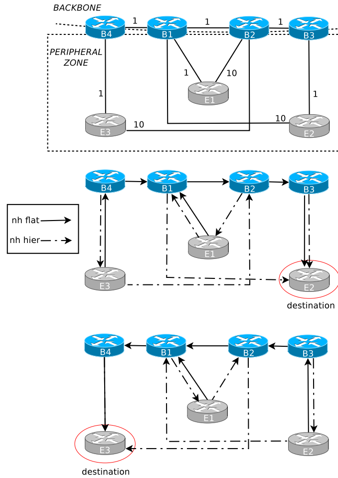
Figure 3.2 Loop Gadget. No migration ordering is loop-free for flat2hier and hier2flat scenarios because of contradictory constraints between B1 and B2 for destinations E2 and E3 .
