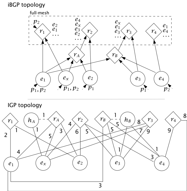
Figure 7.6 Revisited Twice-Bad. Migrating the IGP can create routing oscillations that cannot be avoided at the BGP-level.
