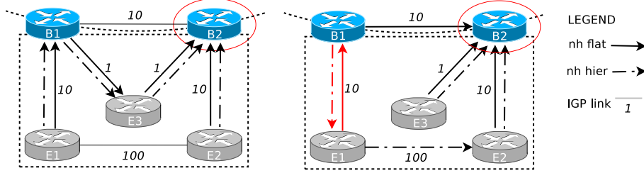
Figure 3.14 Link failures can change the reconfiguration ordering to be followed. In a flat2hier scenario on this topology, a forwarding loop can appear between E1 and B1 if B1 is migrated before E1 and link ( B1 E3 ) fails.
