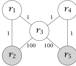
Figure 4.5 Unpopular gadget. In this DV2LS reconfiguration scenario, the Minimal Traverse heuristic is not able to find a per-router ordering free from traffic shifts while there exists one (i.e., r_2 \ r_5 \ r_3 \ r_1 \ r_4 ).
