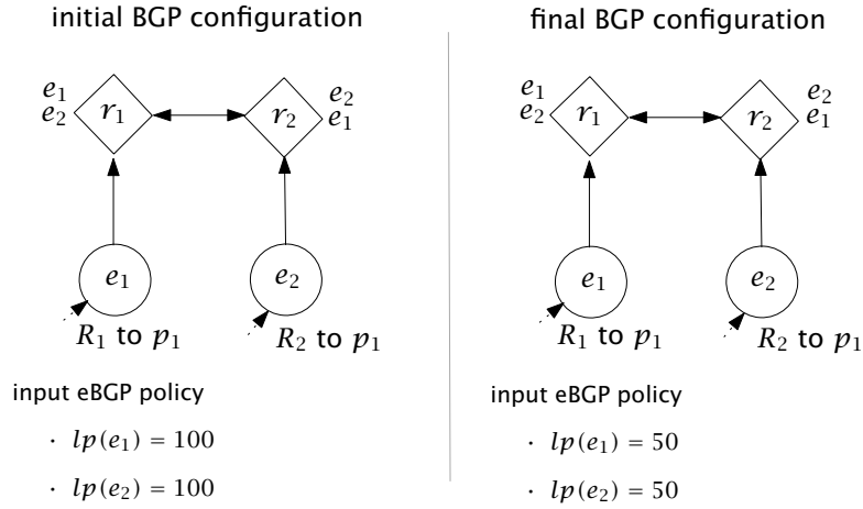
Figure 6.10 Fragile gadget, an eBGP policy reconfiguration case in which unintended traffic shifts occur in every reconfiguration ordering.
