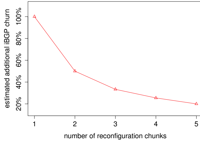
Figure 6.14 Scalability evaluation of BGP SITN with respect to churn.
