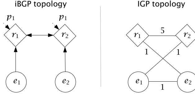
Figure 5.3 An example of BGP configuration in which a forwarding loop exists in the stable state between e_1 and e_2 (taken from [66]).
