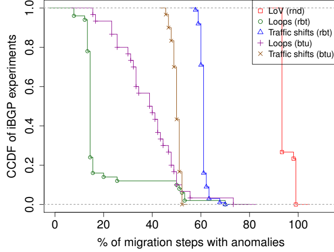
Figure 6.2 Percentage of the migration process affected by anomalies during a full-mesh to route reflection reconfiguration of a Tier-1.
