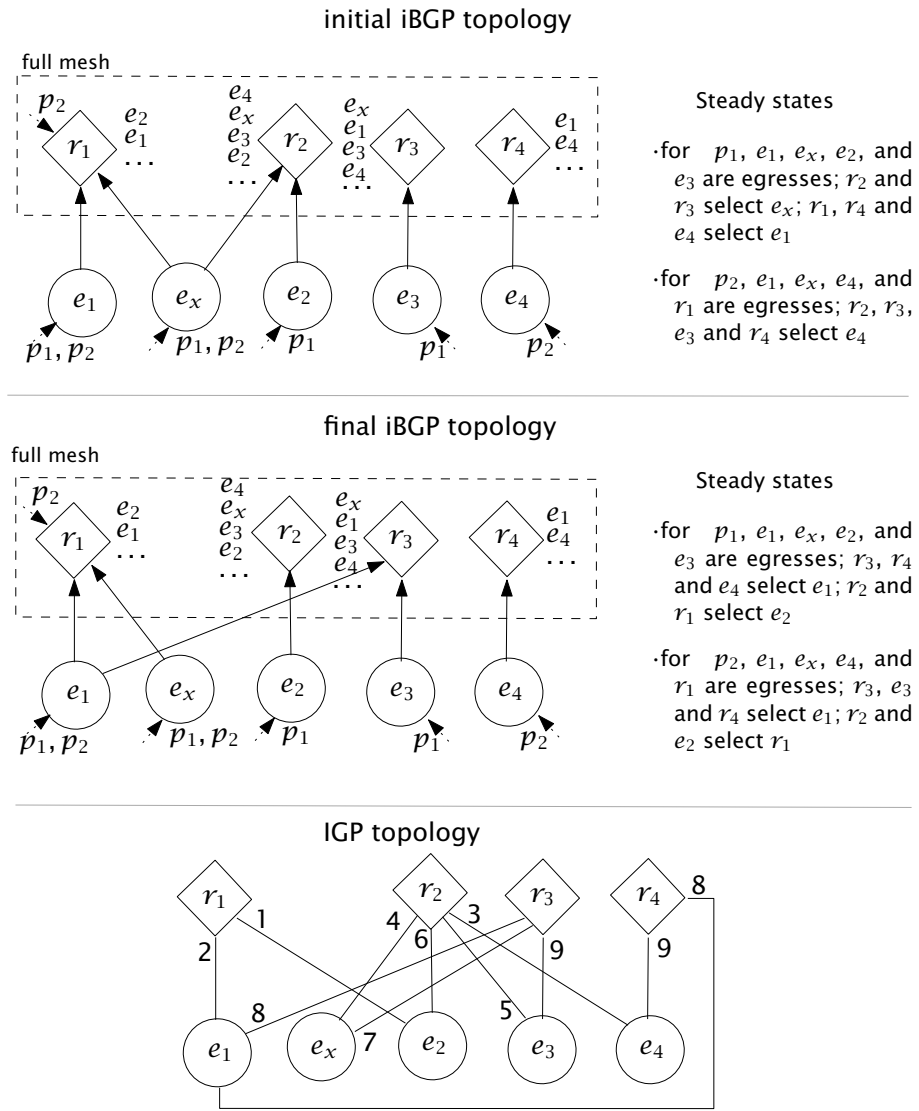
Figure 6.5 Twice-Bad gadget, an iBGP topology change case in which an oscillation-free reconfiguration ordering does not exist.
