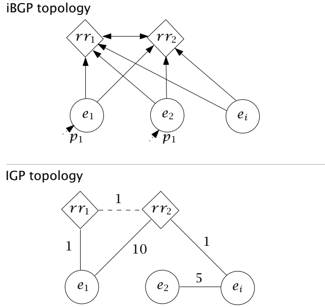
Figure 7.1 Myopia gadget. Migrating the IGP can create BGP-induced forwarding loops. In this flat2hierarchical scenario where rr_1 and rr_2 become ZBR, reconfiguring rr_2 before e_i creates a BGP-induced loop for destination p_1 .
