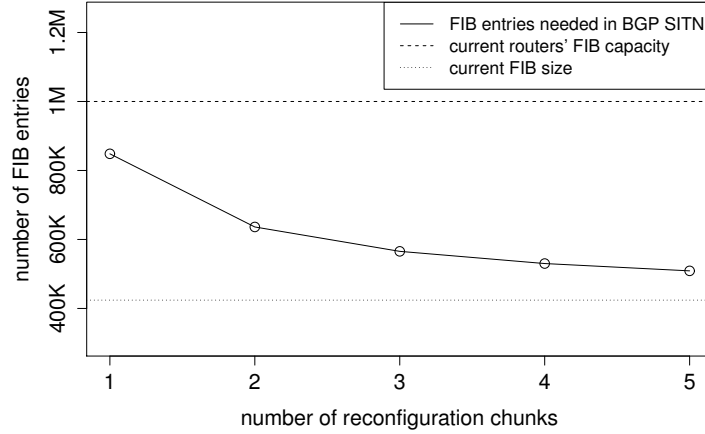
Figure 6.13 Scalability evaluation of BGP SITN with respect to FIB size.
