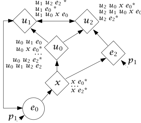
Figure 5.6 Spurious OVER can create routing oscillations.
