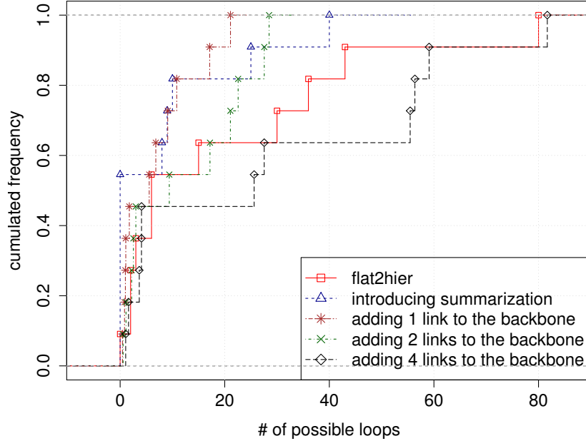
Figure 3.10 CDF of the number of loops that can arise on Rocketfuel topologies. In the worst case, up to 80 different forwarding loops can be created during the reconfiguration.
