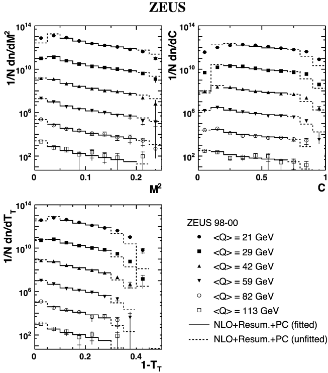
Fig. 6. Differential distributions for the event shapes M^2 , C and 1 - T_T . The distributions are normalised such that n refers to the number of events in the (x, Q^2) bin after the \mathcal{E}_{\text{lim}} cut and N to the total number of events in the (x, Q^2) bin before the \mathcal{E}_{\text{lim}} cut. The differential cross section has been scaled for clarity by factors 10^n , where n = 12, 10, 8, 6, 4, 2 for \langle Q \rangle = 21, 29, 42, 59, 82 and 113 GeV, respectively. The solid (dashed) curves show the points used (omitted) in the fit to NLL resummed calculation matched to NLO plus power corrections.
