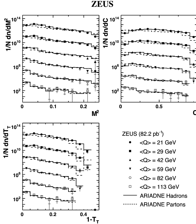
Fig. 4. Differential distributions for the event shapes M^2 , C and 1 - T_T . The distributions are normalised such that n refers to the number of events in the (x, Q^2) bin after the \mathcal{E}_{\text{lim}} cut and N to the total number of events in the (x, Q^2) bin before the \mathcal{E}_{\text{lim}} cut. The differential cross section has been scaled for clarity by factors 10^n , where n = 12, 10, 8, 6, 4, 2 for \langle Q \rangle = 21, 29, 42, 59, 82 and 113 GeV, respectively. Predictions of ARIADNE at the hadron (solid lines) and parton (dashed lines) levels are shown.
