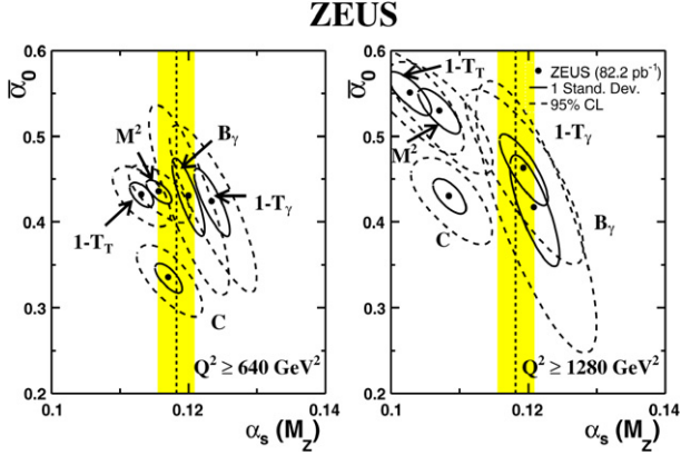
Fig. 9. Extracted parameter values for (\alpha_s, \bar{\alpha}_0) from fits to differential distribution of shape variables using M2mod matching for two different Q^2 intervals.
