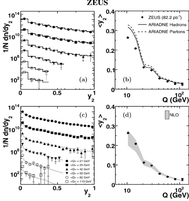
Fig. 10. (a), (c) Differential distribution for y_2 , scaled for clarity by different factors for each \langle Q \rangle -value, and (b), (d) mean distribution of y_2 versus Q compared with predictions from (a), (b) ARIADNE and (c), (d) NLO QCD calculations using DISENT. The ARIADNE predictions are shown for the hadron (solid) and parton (dashed) levels. The NLO calculation (shaded band) uses the CTEQ4A3 proton PDFs.
