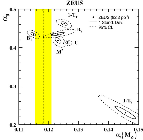
Fig. 3. Extracted parameter values for (\alpha_s, \bar{\alpha}_0) from fits to the mean values of the shape variables. The vertical line and shaded area indicate the world average value of \alpha_s(M_Z) [51].
