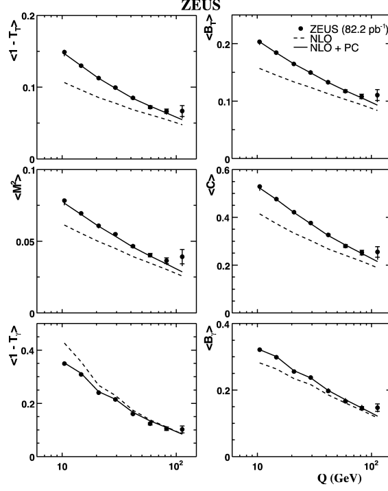
Fig. 2. The mean values of event-shape variables as a function of Q . The solid lines are the results of the fit to the data of the predictions of the sum of NLO pQCD calculations from DISASTER++ and the power corrections. The dashed lines are the DISASTER++ contribution to the fit alone.
