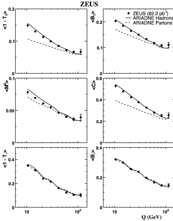
Fig. 1. The mean values of event-shape variables as a function of Q . The solid and dashed lines are the hadron and parton level predictions from ARIADNE, respectively.
