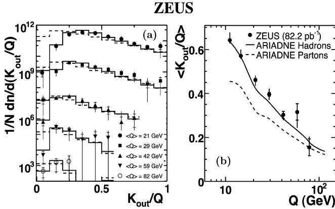
Fig. 11. (a) Differential distribution for K_{OUT}/Q , scaled for clarity by different factors for each \langle Q \rangle value, and (b) mean distribution of K_{OUT}/Q versus Q , compared with predictions from ARIADNE for the hadron (solid) and parton (dashed) levels.
