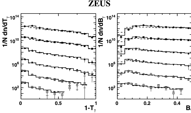
Fig. 5. Differential distributions for the event shapes 1 - T_\gamma and B_\gamma . Other details as in Fig. 4.
