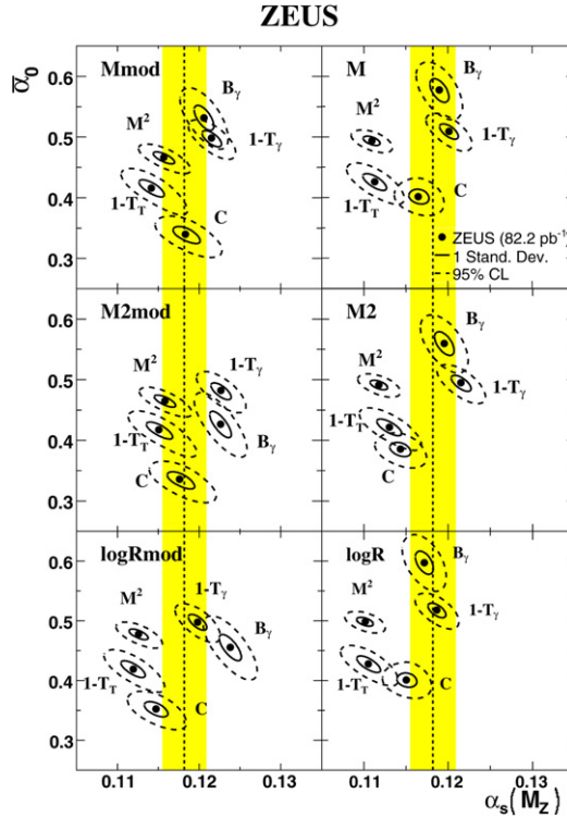
Fig. 8. Extracted parameter values for (\alpha_s, \bar{\alpha}_0) from fits to differential distribution of shape variables for the different matching techniques, which are discussed in Section 6.2.
