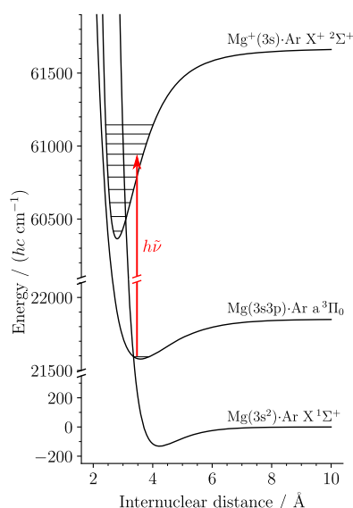
Figure 1. Excitation scheme from the metastable \text{Mg}(3s3p)\cdot\text{Ar a } ^3\Pi_0 state to the \text{Mg}^+(3s)\cdot\text{Ar X}^+ ^2\Sigma^+ state. The ionic potential curve was derived from the data measured in this work and ref 6, as explained in detail in Section 4.1. The potential curves corresponding to the neutral triplet and singlet states are Morse-type potentials based on the molecular parameters from ref 12.
