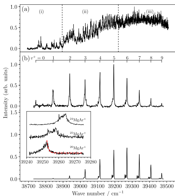
Figure 2. (a) Photoionization spectrum of MgAr in the vicinity of the \text{Mg}^+(3s)\cdot\text{Ar } X^+ 2\Sigma^+ \leftarrow \text{Mg}(3s3p)\cdot\text{Ar } a^3\Pi_0 ionization threshold with the three distinct regions (i)–(iii) described in the text. (b) Measured (upper trace) and calculated (lower trace) overview PFI-ZEKE photoelectron spectra of the \text{Mg}^+(3s)\cdot\text{Ar } X^+ 2\Sigma^+ \leftarrow \text{Mg}(3s3p)\cdot\text{Ar } a^3\Pi_0 ionizing transition. The calculations of Franck–Condon factors were performed using the potential curves shown in Figure 1. The measured intensities of transitions to low- v^+ states are much higher than predicted by the calculation because of channel interactions. The inset shows a MATI spectrum of the transition to the v^+ = 6 level of ^{24}\text{MgAr}^+ , ^{25}\text{MgAr}^+ , and ^{26}\text{MgAr}^+ , from which isotopic shifts and the absolute vibrational assignment were determined.
