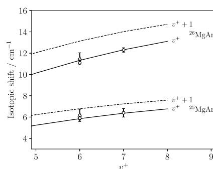
Figure 4. Isotopic shifts of the v^+ = 6 and 7 levels of ^{25,26}\text{MgAr}^+ with respect to ^{24}\text{MgAr}^+ determined from PFI-ZEKE photoelectron (circles) and MATI (triangles) spectra, respectively. The solid line is the prediction for the case that the lowest observed level corresponds to v^+ = 0 (see Figure 2b). The dashed line corresponds to the case where the lowest observed level would be v^+ = 1 . The shifts were predicted from potential curves, which were fitted to the experimental data, as explained in Section 4.1.
