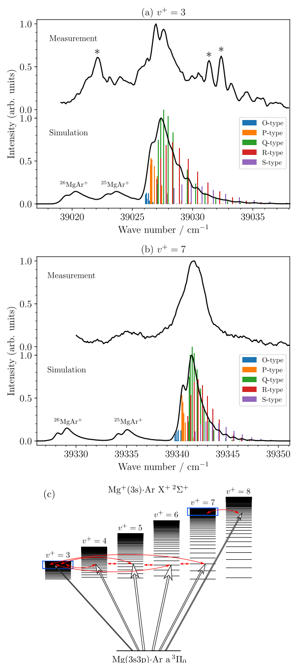
Figure 3. (a, b) High-resolution experimental (upper trace) and calculated (lower trace) PFI-ZEKE photoelectron spectra of the transitions to the \text{Mg}^+(3s) \cdot \text{Ar } X^+ 2\Sigma^+ , v^+ = 3 and 7 states. The calculation of the rotational structure was performed using the model of Buckingham et al., 20 assuming photoionization from a pure p orbital, a rotational temperature of 3 K, and a resolution (full width at half maximum, FWHM) of 0.6 cm -1 . Whereas the calculated spectrum of the v^+ = 7 band is in agreement with the experimental spectrum and exhibits the isotope structure, the spectrum of the v^+ = 3 band reveals several perturbations (marked with asterisks) originating from the channel interactions illustrated in (c) (see the text for details).
