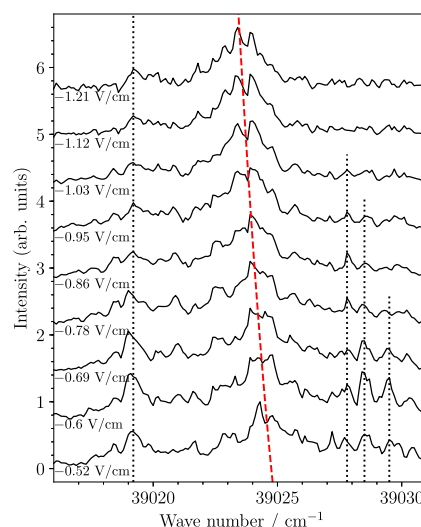
Figure 5. PFI-ZEKE photoelectron spectra of the \text{Mg}^+(3s)\cdot\text{Ar } X^+ 2\Sigma^+ (v^+) \leftarrow \text{Mg}(3s3p)\cdot\text{Ar } a^3\Pi_0 (v'' = 0) ionizing transition without correction of the field-induced shift of the ionization thresholds. The corresponding electric-field-pulse strengths are indicated below each spectrum. The vertical dotted line indicates the position of a perturber line. The dashed curve indicates the position of the main line of the PFI-ZEKE photoelectron spectrum.
