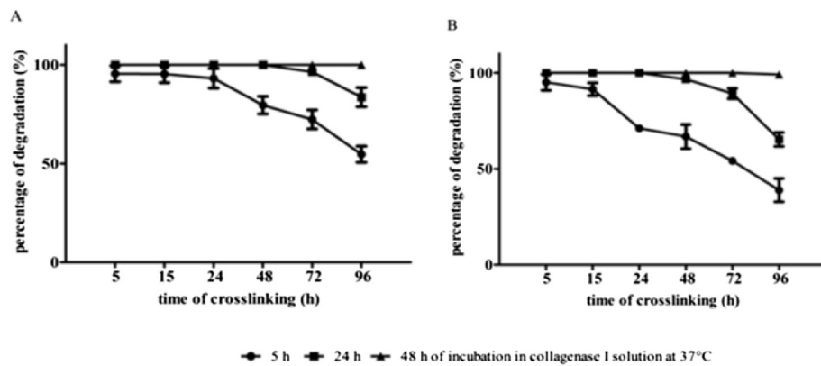
Fig. 5. In vitro enzymatic (collagenase I) degradation of gelatin microspheres ( n = 3 ; \pm SD) crosslinked using 0.1 w/v % (A) and 0.5 w/v % (B) genipin and different crosslinking times.
