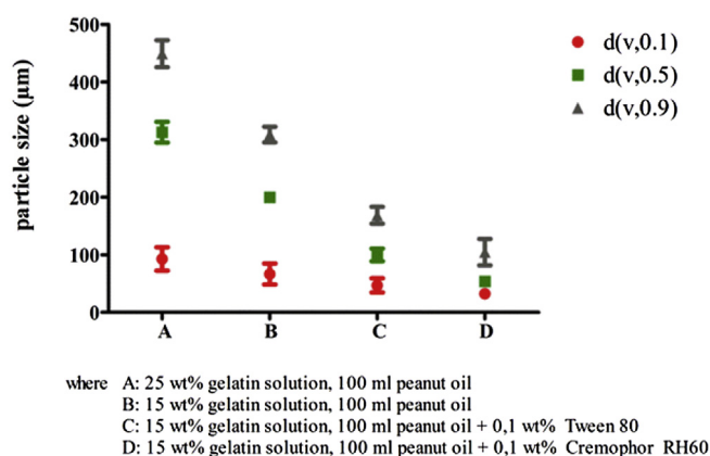
Fig. 2. Influence of the composition of the emulsion on the size of the gelatin microspheres ( n = 3 ; \pm SD).
