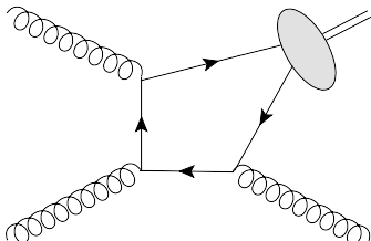
FIG. 2: One of the 6 Feynman diagrams for gg \rightarrow J/\psi g at order g_s^3 with vertex \Gamma_\mu .
