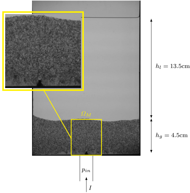
Fig. 5: Initial situation for the experimental setup. Settled polystyrene grains form a bed of height h_g in ethanol. The height of fluid above the bed is h_l . Air is injected at constant inflow-rate I = 6.5 \text{ mL/min} in the injection pipe where the pressure p_{in} is measured. \Omega_M is the area centred around the injector in which motion of grains are considered.
