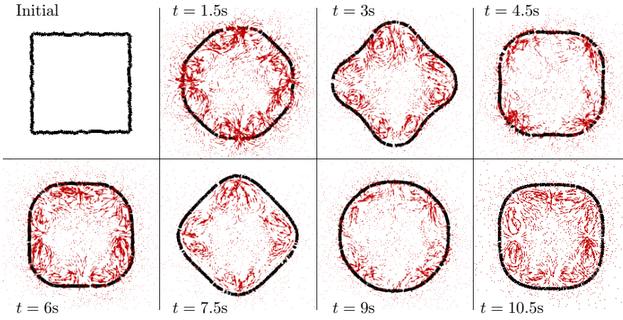
Fig. 1: Time evolution of an air drop with initial square shape surrounded by ethanol in the absence of gravity. A constant time step of 1.5s is taken between successive snapshots. The interface is represented by the black line on the pictures where the phase indicator function is equal to 0.5. Red arrows represent the fluid velocity field.
