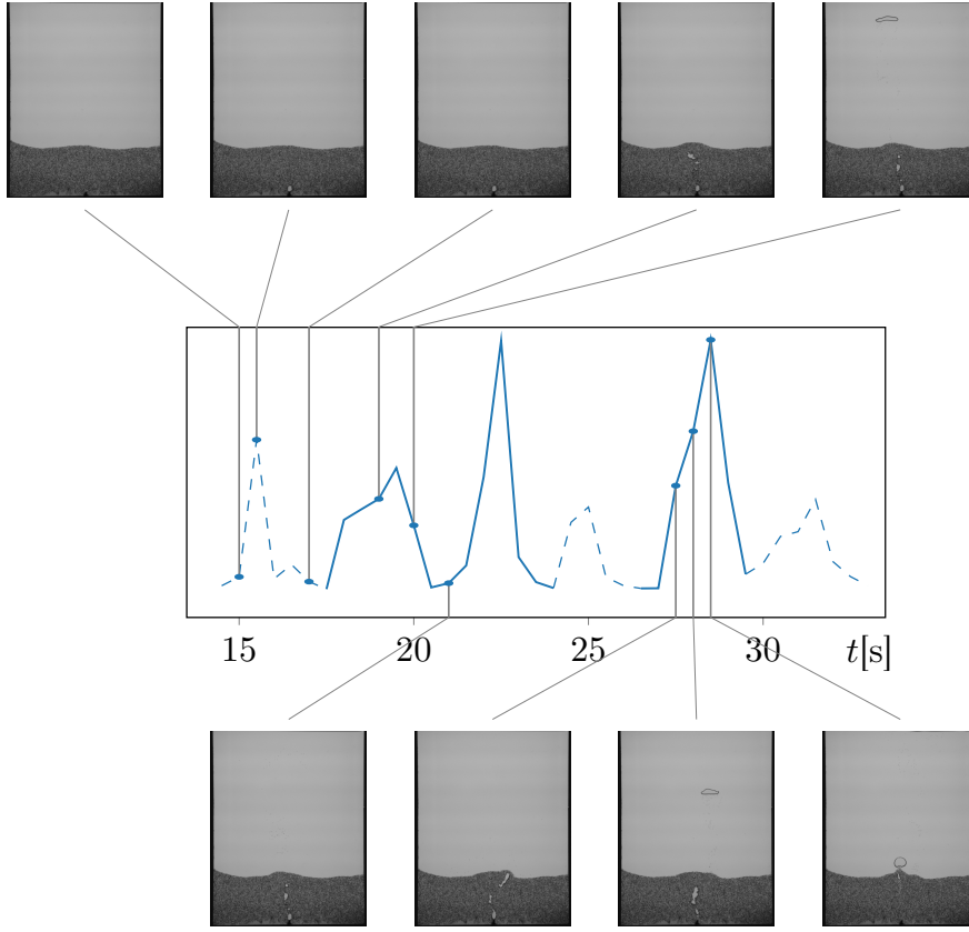
Fig. 7: Successive events can be related to motions in the granular bed. Events are located in time on the difference curve used to determine a motion during the experiment. Some peaks are related to a cavity creation without bubble emission (top images) while two bubbles can be created during the same motion peak (bottom images).
