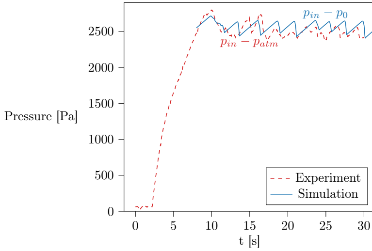
Fig. 12: Comparison of the differential pressure signals in the injection pipe obtained numerically and experimentally for the case h_g = 4.5 cm and I = 13 mL/min ( Ca = 1.2 \cdot 10^{-2} , Re_s = 196.3 and \Delta t = 1.125 \cdot 10^{-4} s). p_0 is the reference pressure for the simulation and p_{atm} is the atmospheric pressure.
