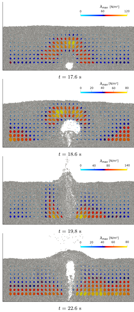
Fig. 15: Representation of the stress tensor inside the granular medium at different times. The stress tensor is represented by ellipses giving the eigenvectors direction and coloured with respect to their greatest eigenvalue \lambda_{max} .
