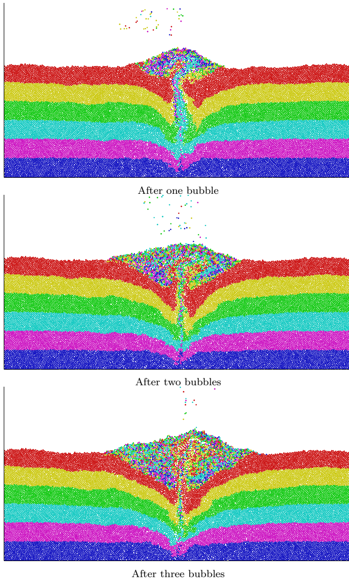
Fig. 14: Configuration of the grains inside the bed after the passage of one, two and three bubbles for the case h_g = 4.5 cm and I = 6.5 ml/min. Grains are colored with respect to their initial height.
