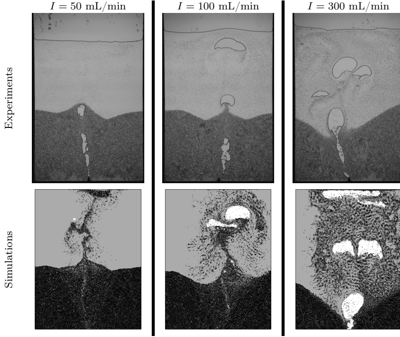
Fig. 17: Granular bed states for h_g = 9 cm and I = 50 mL/min ( Ca = 1.4 \cdot 10^{-2} , Re_s = 229.0 and \Delta t = 2.5 \cdot 10^{-4} s), I = 100 mL/min ( Ca = 2.4 \cdot 10^{-2} , Re_s = 392.5 and \Delta t = 1.125 \cdot 10^{-4} s) and I = 300 mL/min ( Ca = 2.6 \cdot 10^{-2} , Re_s = 425.2 and \Delta t = 5.625 \cdot 10^{-5} s) after 10 s. The fluid-grains interface takes a flat W-like shape for the smaller inflow rate while for the intermediate inflow rate the angles are sharper. With the higher inflow rate the number of suspended grains is more important so that the sliding planes ended around the air invasion channel forming a V-like shape interface.
