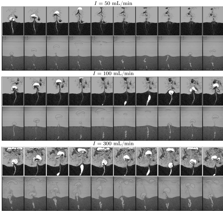
Fig. 16: Comparison between simulations and experiments of the air invading a granular bed of height h_g = 9 cm at inflow rate I = 50 mL/min (top), I = 100 mL/min (middle) and I = 300 mL/min (bottom). For each case, the simulation corresponds to the first row of images. The time step between two successive images is 0.1 s.
