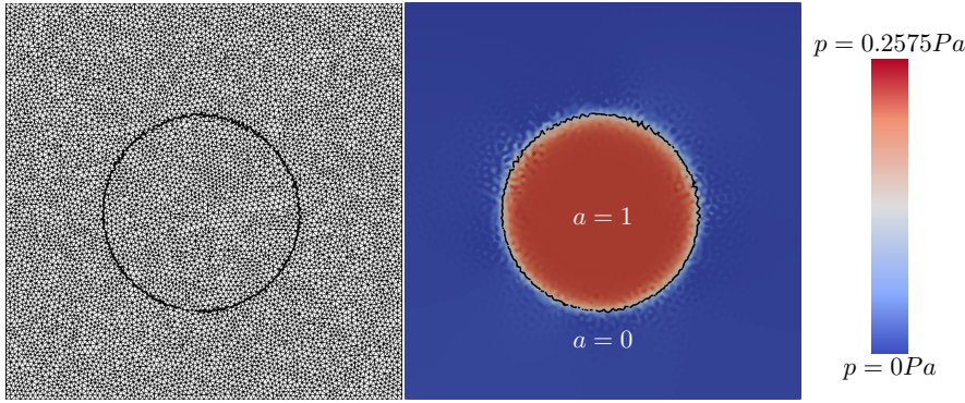
Fig. 2: State of the air drop with an initial square shape surrounded by ethanol at t = 40 s. Left figure shows the mesh used for the computation and right figure shows the pressure field. The interface is the black line located where the phase indicator function is equal to 0.5. Oscillations in the pressure field can be seen near the interface where spurious currents are located.
