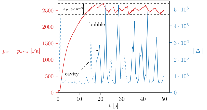
Fig. 6: Evolution of the differential pressure in the injection pipe and Manhattan norm of the difference between pixels of two successive image captures situating in time important motions in the granular bed for the case h_g = 4.5 cm and I = 6.5 mL/min. p_{atm} is the atmospheric pressure. Dashed parts of the Manhattan norm curve represent the movements that are not associated with a bubble emission.
