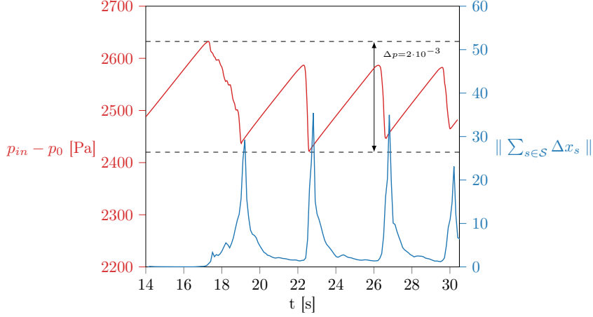
Fig. 11: Simulated evolution of the differential pressure pressure in the injection pipe and norm of the displacement of all grains in time for the case h_g = 4.5 cm and I = 6.5 mL/min ( Ca = 8 \cdot 10^{-3} , Re = 130.8 and \Delta t = 2.5 \cdot 10^{-4} s). p_0 is the reference pressure.
