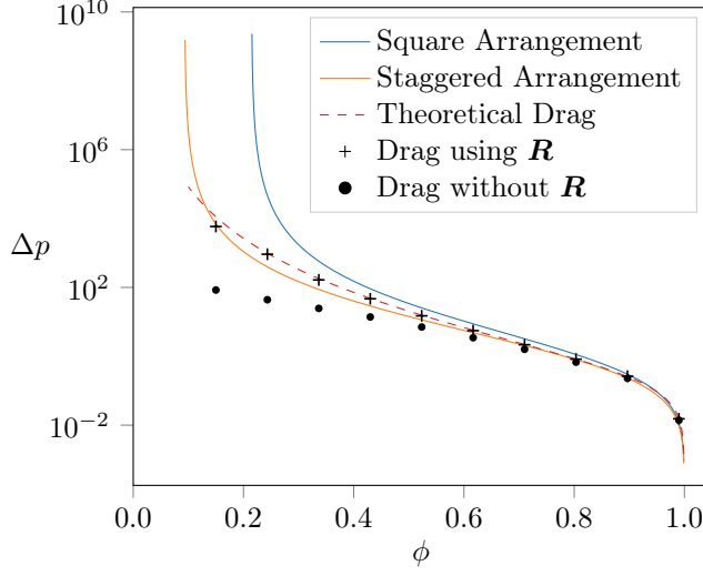
Fig. 4: Pressure drop accross a porous medium for \mathbf{u} = 10^{-5}\text{m/s} in the x-direction and \mu = 1 \text{ Pa}\cdot\text{s} . Solid lines show the results obtained using the formulas of Tamayol and Bahrami [54] for a square arrangement (blue) and for a staggered arrangement (orange). Dashed line presents the results obtained by balancing theoretically the drag force given in Equation (18) and the marks present the results obtained by the use of the complete numerical model.
