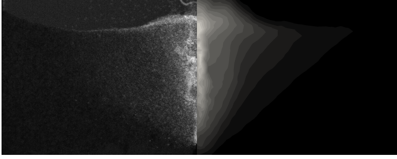
Fig. 13: Representation of the area where the motion are dominant after 30.5 s for the case h_g = 4.5 cm and I = 6.5 mL/min. The experiment (left) is compared to the simulation (right). In the simulation, the Eulerian representation of the grains velocity is cumulated over time to determine areas where the motion are dominant while in the experiment we make use of the cumulative pixels intensity difference between two successive image captures.
