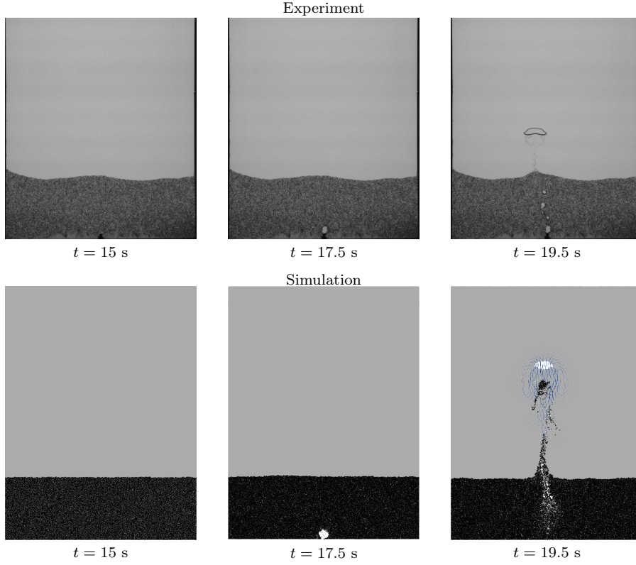
Fig. 8: Comparison between experimental and numerical results shows the system evolution during one period of gas invasion for h_g = 4.5 cm and I = 6.5 mL/min. The left figures show the initial bed, the middle ones the cavity creation as the pressure increases in the pipe, the right ones a bubble ascent with grains in its wake.
