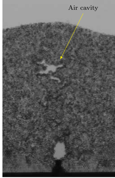
Fig. 10: Granular bed fracture due to air invasion creates cavities in which air may be clogged.
