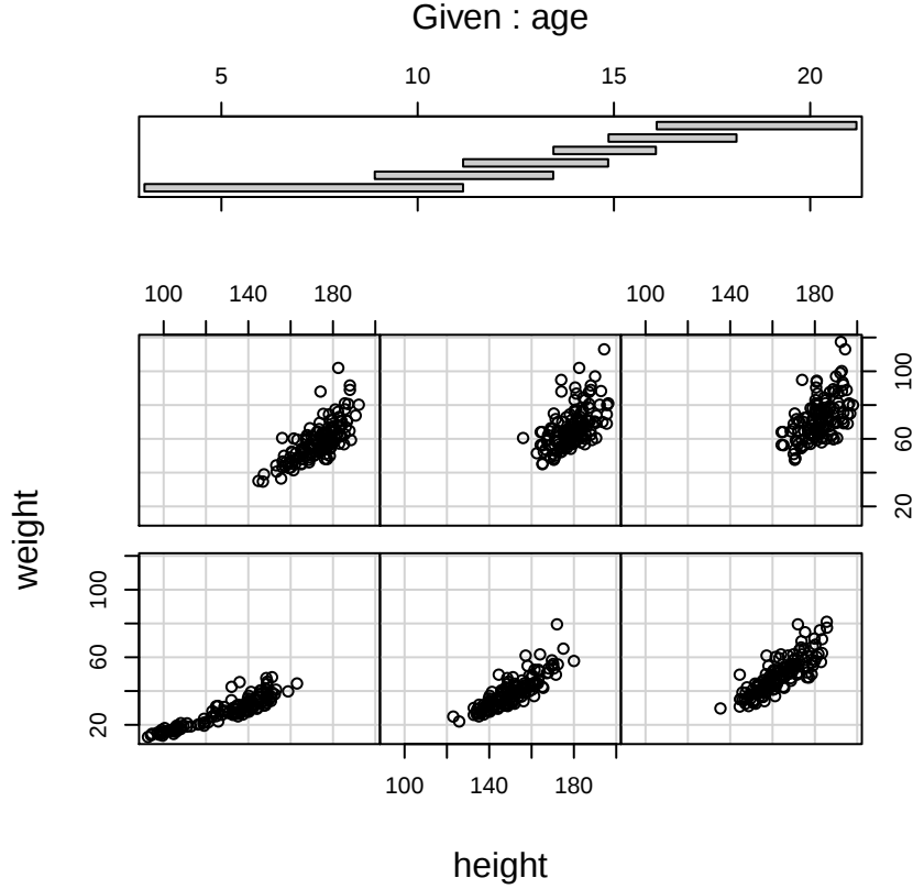
Figure 1: Growth dataset (for 441 Dutch boys): conditional scatterplot of weight versus height for different age classes.
