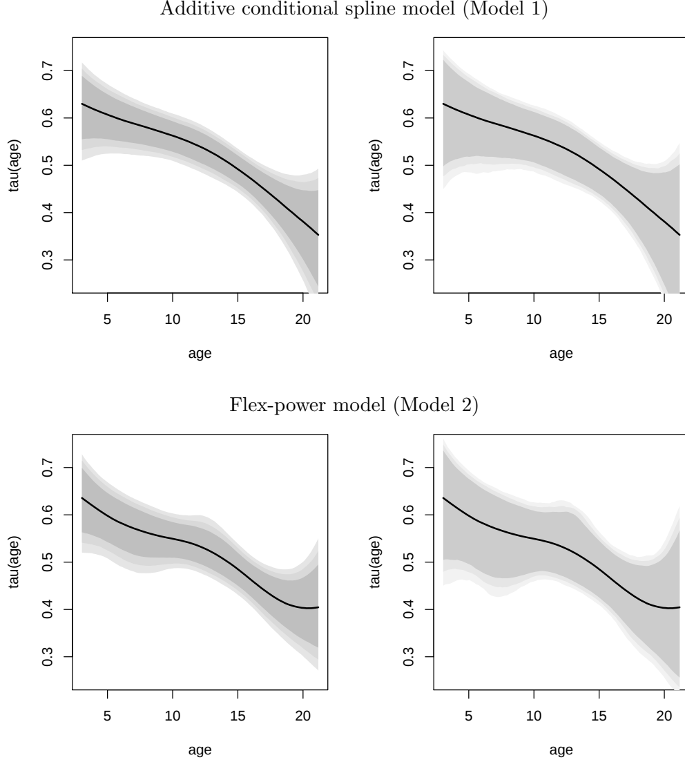
Figure 6: Growth dataset: fitted (solid line) conditional Kendall's tau under the additive conditional spline and the flex-power Archimedean copula models. Grey areas corresponds to .80, .90 and .95 pointwise (left panel) or simultaneous (right panel) credible regions for \tau(\text{age}) .
