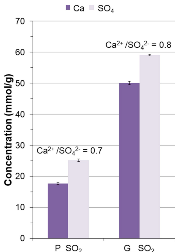
Fig. 5. Ratio of \text{Ca}^{2+} to \text{SO}_4^{2-} abundance (mmol/g) in \text{SO}_2 -exposed pumice (P_ \text{SO}_2 ) and glass (G_ \text{SO}_2 ) measured in solutions extracted after 60 min leaching in deionized water. The data are shown as the mean \pm standard error of the mean ( n = 3 ).
