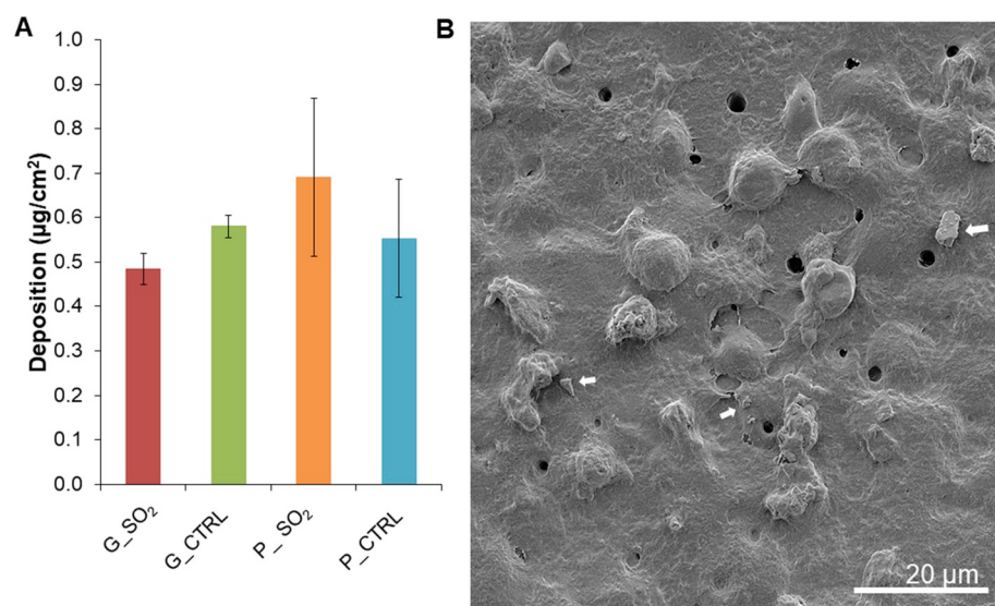
Fig. 7. Deposition of nebulized respirable fraction of SO 2 -exposed and control glass and pumice samples. A) Average mass deposition (μg/cm 2 ) of SO 2 -exposed glass (G_SO 2 ) and pumice (P_SO 2 ) and their respective controls (G_CTRL and P_CTRL) quantified using a quartz crystal microbalance (QCM), following their dry nebulisation using a dry powder insufflator (DP-4, Penn Century, USA). Data are shown as the mean ± standard error of the mean, related to the following repetitions for each exposure: G_SO 2 and G_CTRL n = 5, P_SO 2 and P_CTRL n = 3. B) Representative scanning electron micrograph of the apical side of the multicellular lung model, showing deposited particles (indicated with white arrows). The image was collected at 2 kV and 16.13 mm working distance. Scale bar is 20 μm.
