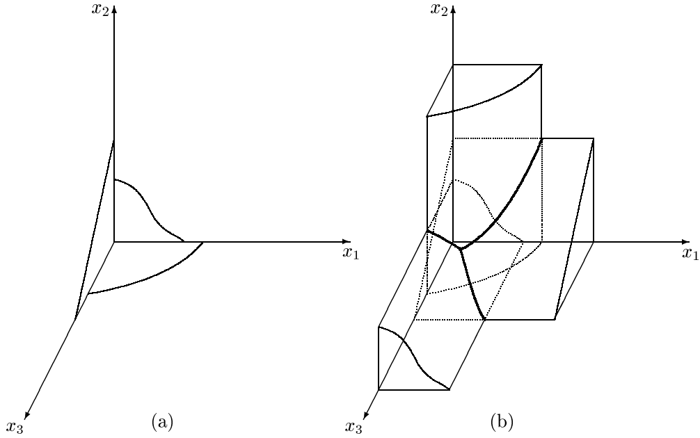
Figure 2: Aspirations in three-agent NTU games: In the picture, N = \{1, 2, 3\} , V(\{1\}) = V(\{2\}) = V(\{3\}) = -\mathbb{R}_+ , and V(N) = -\mathbb{R}_+ . The set of aspiration in V is the union of three thick curves in (b).
