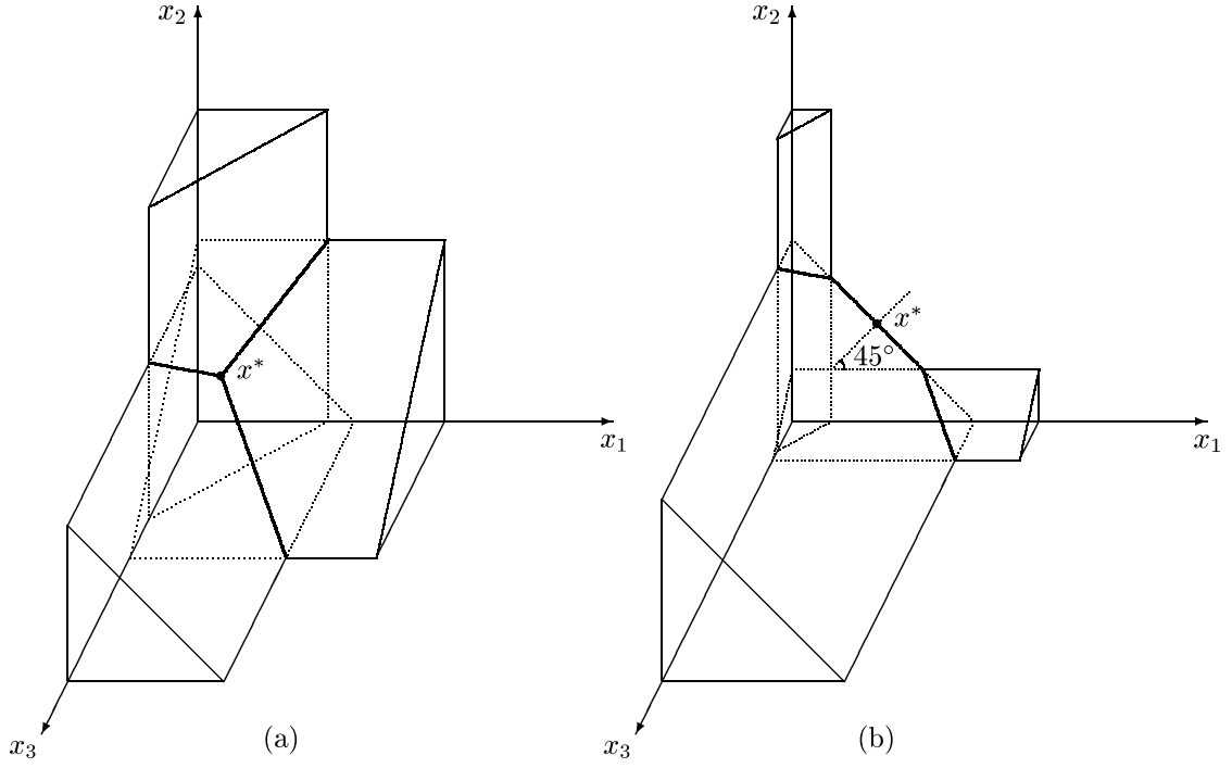
Figure 4: The aspiration nucleolus and the aspiration kernel in three-agent TU games. In both panels, V(\{1, 2, 3\}) = -\mathbb{R}_+^{\{1,2,3\}} and the payoff vector chosen by the aspiration nucleolus is indicated as x^* . It can be shown that for the three-agent case, the aspiration kernel is single-valued so that it coincides with the aspiration nucleolus.
