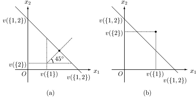
Figure 3: The aspiration nucleolus and the aspiration kernel in two-agent TU games. (a) If v(\{1,2\}) \geq v(\{1\}) + v(\{2\}) , then the aspiration nucleolus selects the “standard solution” payoff vector: each agent is given first her individual worth, and then what remains is divided equally. (b) Otherwise, it selects (v(\{1\}), v(\{2\})) . It is easy to see that the aspiration nucleolus and the aspiration kernel coincide for the two-agent case.
