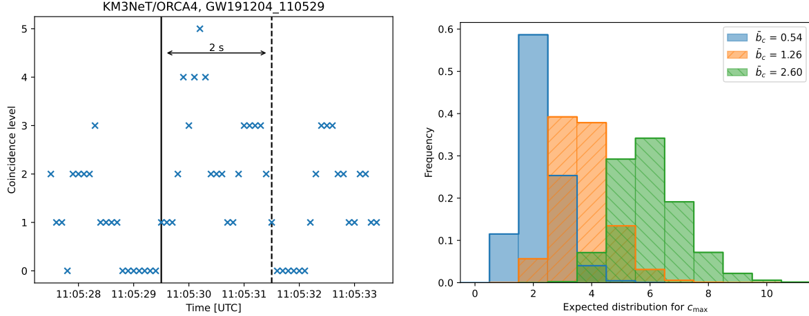
Figure 3. Timeline of the coincidence levels around GW191204_110529 (left) and distribution of the maximum coincidence level c_{\text{max}} for different values of the mean rate \bar{b}_c (right). On the left, the solid black line indicates the GW event time, and the dashed black line is the end of the 2s time window during which the search is made.
