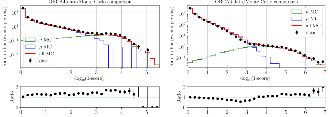
Figure 6. Comparisons of the score for upgoing events in data and Monte Carlo simulations, for the ORCA4 (left) and ORCA6 (right) detector configurations.
