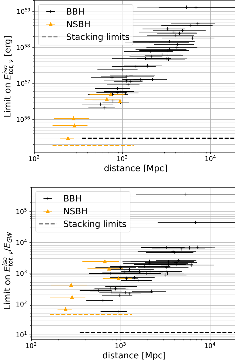
Figure 9. 90% upper limits on the total energy E_{\text{tot},\nu}^{\text{iso}} emitted in neutrinos of all flavors (top) and on the ratio f_{\nu}^{\text{iso}} = E_{\text{tot},\nu}^{\text{iso}}/E_{\text{GW}} (bottom) as a function of the source luminosity distance, assuming an E^{-2} spectrum and isotropic emission. The horizontal bars indicate the 5-95% range of the luminosity distance estimate, and the markers/colors correspond to the different source categories. The dashed bars correspond to the upper limits from the stacking analysis for BBH and NSBH categories.
