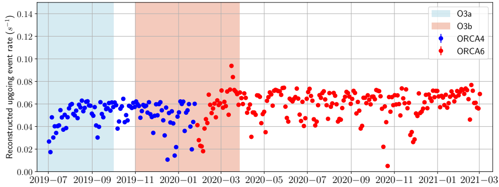
Figure 5. Rate of reconstructed upgoing events averaged over intervals of two days, for the two detector configurations ORCA4 (blue points) and ORCA6 (red points) in the data set. The shaded regions indicate the O3a and O3b periods.
