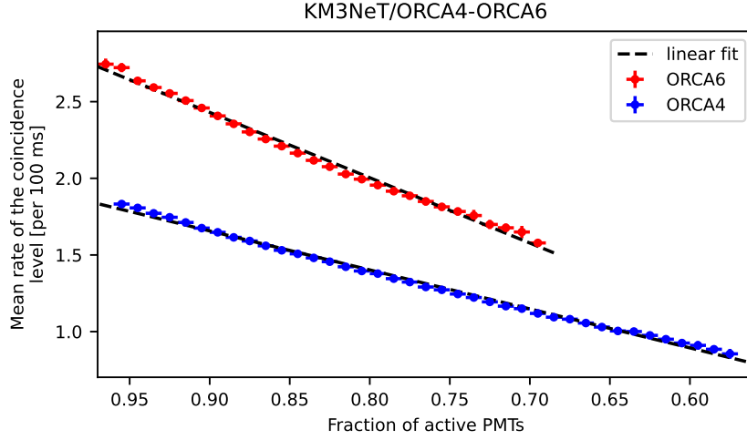
Figure 2. Mean rate of the coincidence level as a function of the fraction of active PMTs for ORCA4 (blue) and ORCA6 (red). The crosses indicate averaged values over the full periods, and the dashed lines are linear fits to these points.
