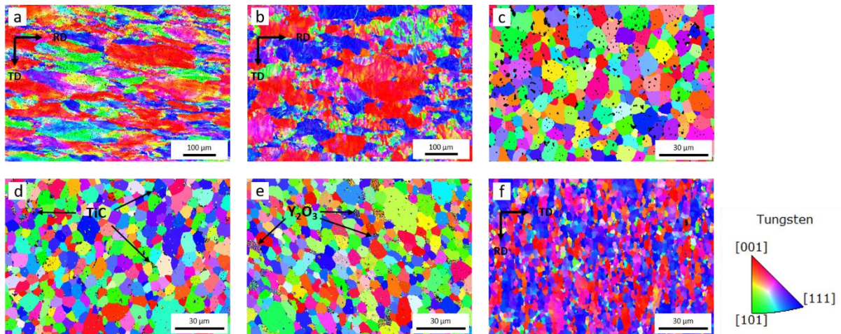
Figure 1. Normal direction (ND) Inverse pole figure (IPF) of baseline and advanced W; (a) IGP; (b) CEFTR; (c) FG; (d) W1TiC; (e) W2YO; and (f) W0.5ZC
