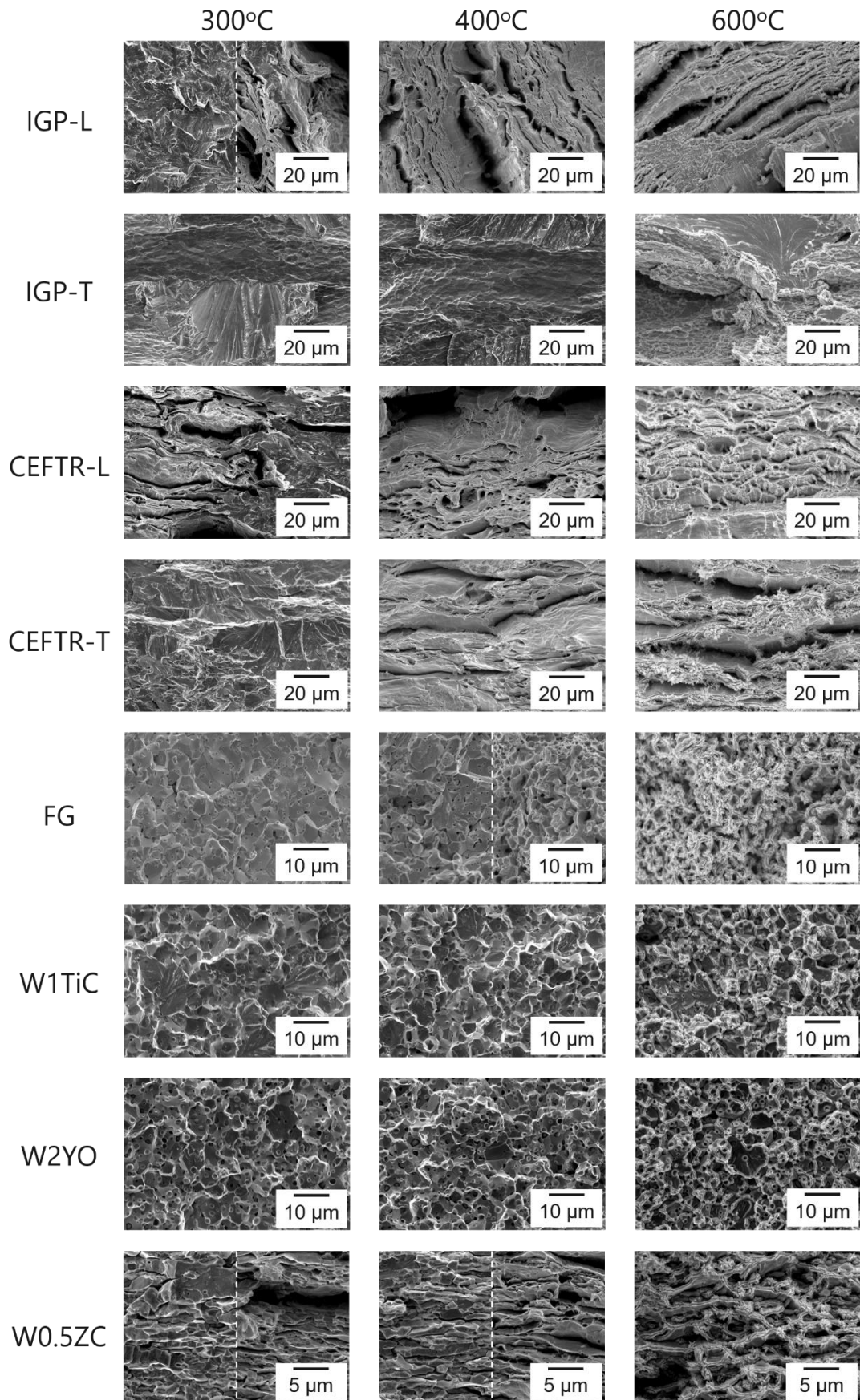
Figure 7. High magnification of fracture surface, as observed by SEM
