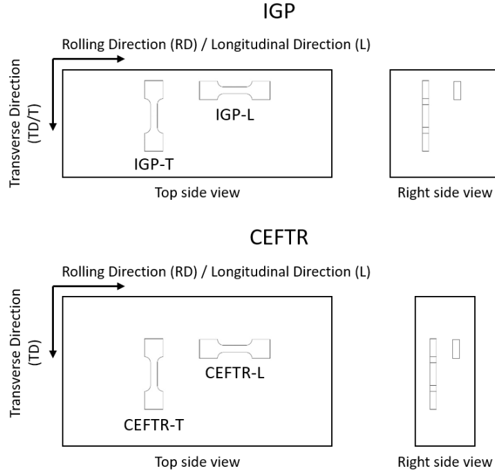
Figure 3. Sample orientation
