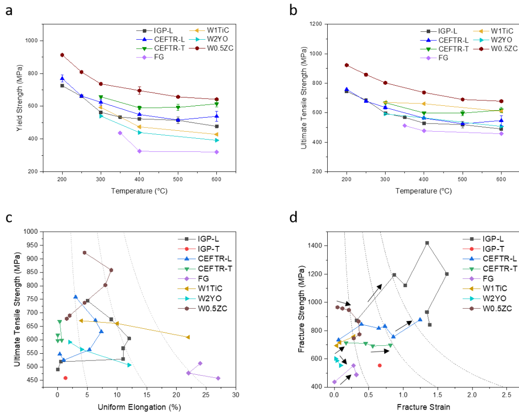
Figure 5. Comparison of the mechanical properties of baseline and advanced W as a function of test temperature; (a) YS; (b) UTS; (c) UTS vs. uniform elongation; (d) Fracture strength vs. fracture strain, the arrows indicate the trend of increasing/reducing the test temperature.
