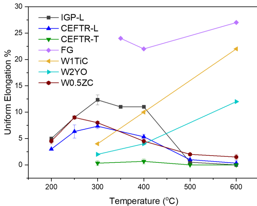
Figure 8. The variation of uniform elongation with temperature
