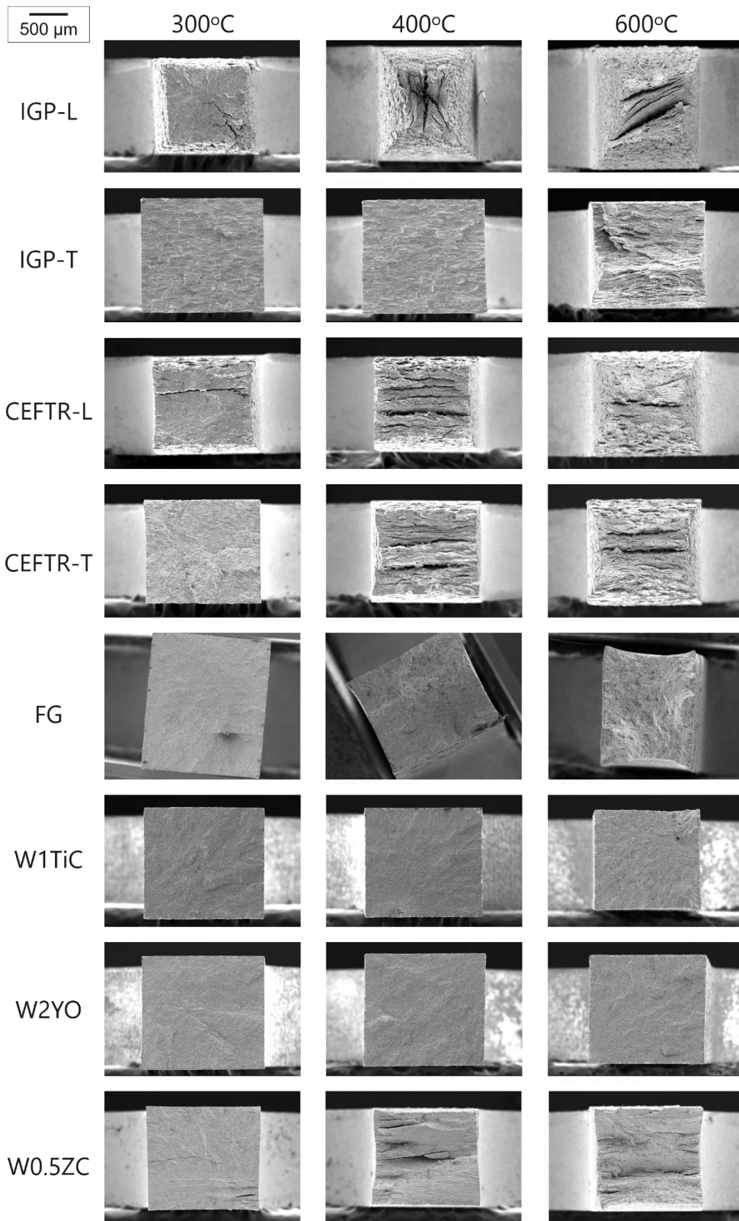
Figure 6. Macroscopic appearance of fracture surface, as observed by SEM. The length scale bar, to be applied for all the micrographs, is depicted in the upper left corner.
