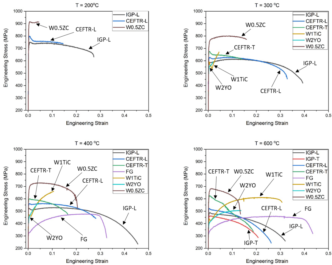
Figure 4. Stress-strain curve of baseline and advanced W
