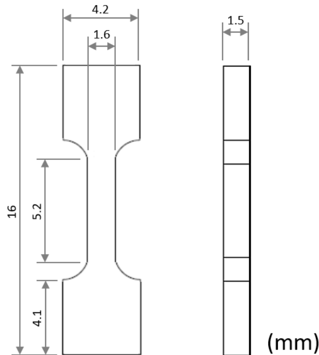
Figure 2. Sketch of small dog-bone shaped specimens
