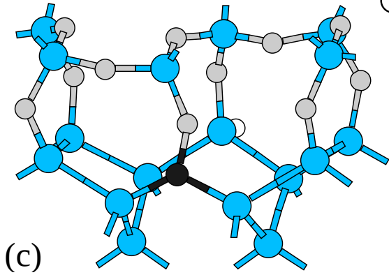
FIG. 1. Models of the Si(001)-SiO 2 interface (a) before N incorporation (from [12]), (b) including a N-Si 3 (model I) configuration, and (c) including a N-Si 2 O (model IV) configuration. L -1 , L 0 and L 1 label the Si layers.
