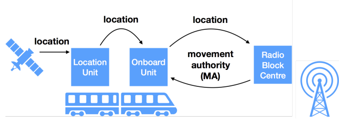
Fig. 1. ERTMS Level 3 moving block railway signalling (adapted from [8,29])
