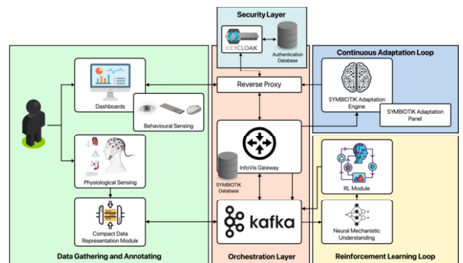
Figure 2. SYMBIOTIK high-level software architecture.
