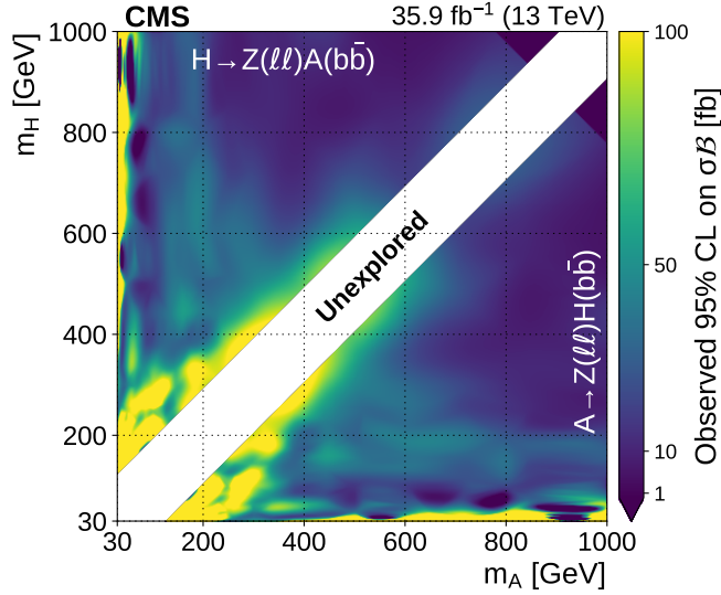
Figure 5.29. | Observed 95% CL upper limits on the product of the production cross section and branching ratio for H ( A ) \rightarrow Z\ell\ell A ( H ) \rightarrow \ell^+\ell^-b\bar{b} as a function of m_A and m_H .
