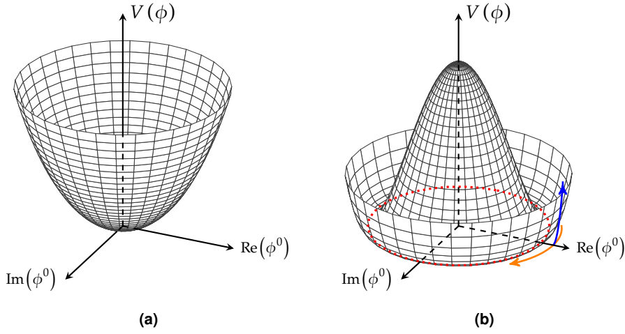
Figure 1.1. | Higgs potential, visualized as a function of the complex field \phi^0 , in the case \mu^2 > 0 (a) and \mu^2 < 0 (b).
