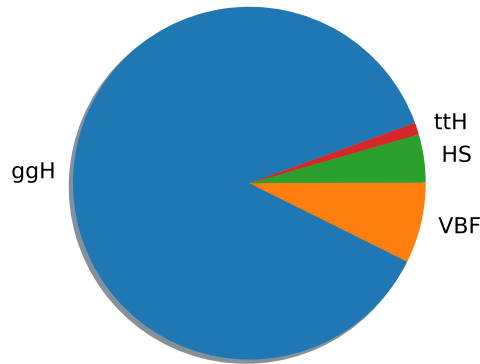
Figure 1.3. | Production modes of a Higgs boson with a mass of 125 GeV at the LHC. The production through gluon-gluon fusion ( ggH ), vector boson fusion ( VBF ), Higgs-strahlung ( HS ), and associated production with top quark pairs ( ttH ) amounts to \sim 87\% , \sim 7.4\% , \sim 4.4\% , and \sim 1\% of the total Higgs boson production, respectively.
