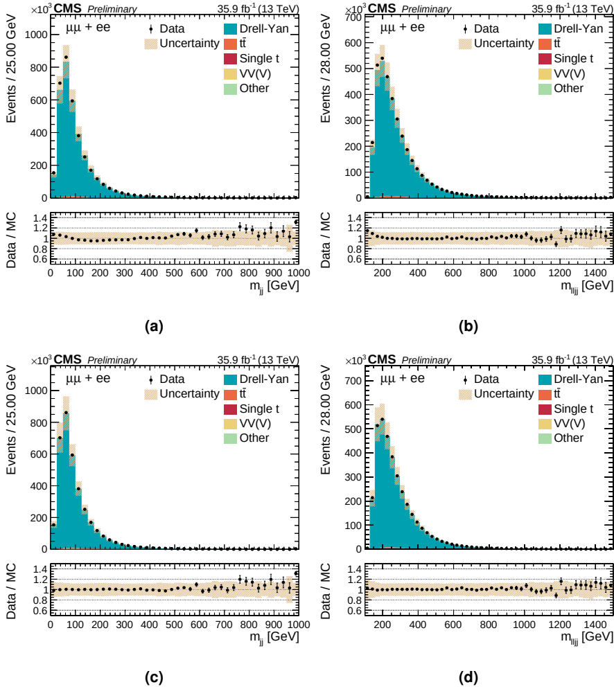
Figure 5.23. | Invariant mass distribution of the di-jet system (left) and of the \ell\ell jj system (right) in the NB control region without (upper) and with (lower) DY reweighting for SF events. Error bars indicate statistical uncertainty, while shaded bands indicate systematic uncertainties.
