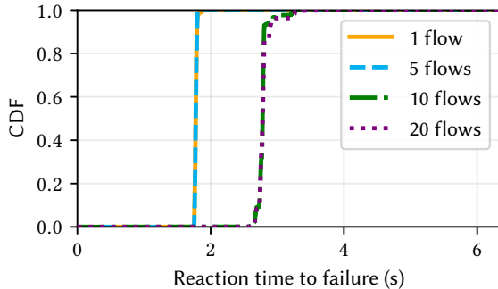
Fig. 10. CDF of the recovery time with increasing numbers of parallel flows with NRTOChanger( N=3, M=2 ).
