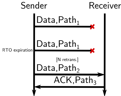
Fig. 5. Detecting failures on the forward path.
