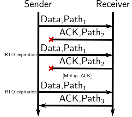
Fig. 6. Detecting failures on the return path.
