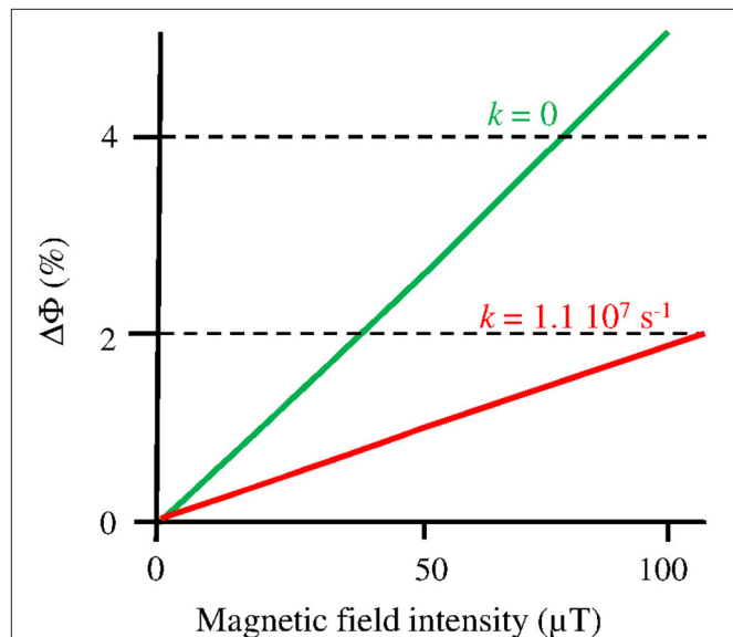
FIGURE 2 | Change (%) of the yield ( \Phi ) of \text{FADH}^\bullet in AtCry 1, thus of the constant k_1 of its photoreduction, according to the intensity B of a static MF under flash photolysis (adapted with permission from Maeda et al., 2012, © National Academy of Sciences of the United States of America). The graph focuses on the Earth strength range, where the MF effect is to increase \Phi ( k_1 ). The function \Delta\Phi(B) is shown here for k_{\text{STD}}(k) = 1.1 \cdot 10^7 \text{ s}^{-1} , where it best fits the experimental observations, and for k_{\text{STD}} = 0 , which can be the case in vivo (see text).
