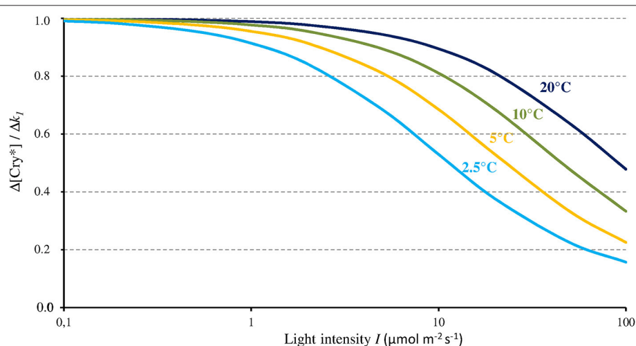
FIGURE 3 | Change of the concentration of the active form of Cry ( \text{Cry}^* ) relative to the change of k_1 (as caused by a MF) as a function of blue light intensity ( I , 350–500 nm) and for different temperatures. From that relationship, a MF can thus only express its full effect at low light intensities.
