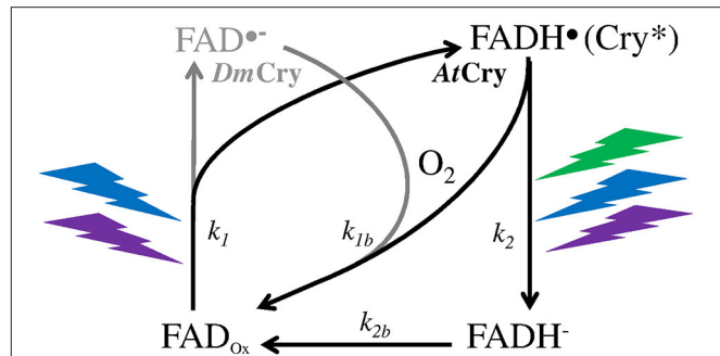
FIGURE 1 | Photocycle of the FAD cofactor of the Cry protein of the plant Arabidopsis thaliana (AtCry, in black) (Procopio et al., 2016) and of the fruit fly Drosophila (DmCry, in gray) (Arthaut et al., 2017). Under exposure to light (350–500 nm, UVA to blue), the oxidized form of AtCry is readily reduced. The radical form (neutral in AtCry, anionic in DmCry) that results from this step is the active one ( \text{Cry}^* ). The binding of that form with signaling partners causes its phosphorylation and subsequent proteolysis. In DmCry, \text{FAD}^{\bullet-} undergoes direct reoxidation with dioxygen. In AtCry, \text{FADH}^\bullet is either directly reoxidized or fully reduced by light (350–580 nm, UVA to green) and further reoxidized.
