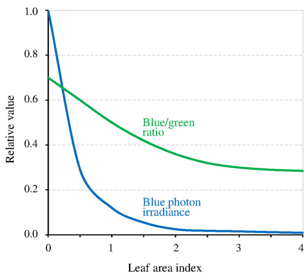
FIGURE 5 | Relative value of blue light intensity and of the blue/green ratio as a function of the density of the canopy coverage expressed as the leaf area index (an index of 1 corresponds to a single layer of leaves) (adapted with permission from Sellaro et al., 2010, © American Society of Plant Biologists).
