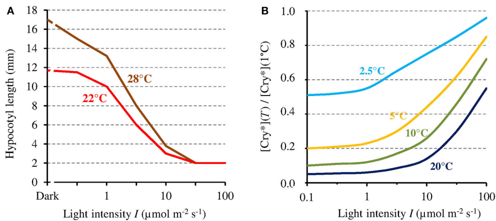
FIGURE 4 | (A) Hypocotyl growth in AtCry 1 according to blue light intensity ( I ), respectively at 22° and 28°C (adapted with permission from Ma et al., 2016, © National Academy of Sciences of the United States of America). (B) [\text{Cry}^*] expressed as its value relative to that at 1°C, at different temperatures and as a function of I , as evaluated from the present model (this assumes the function k_{1b}(T) to be linear and is thus only valid at \leq 20^\circ\text{C} [see text]). [\text{Cry}^*] varies with I and T in a way comparable but inverse to hypocotyl growth.
