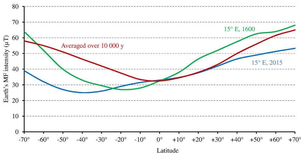
FIGURE 7 | Relation between Earth's MF intensity and latitude, averaged over the last 10,000 years according to the models CALS10k.2 or HFM.OL1.A1 (standard deviation is 2–5 \mu\text{T} ) (adapted with permission from Constable et al., 2016, © Elsevier B.V.), and at 15° longitude E, where the studies by Stenøien et al. (2002) and Ranade and García-Gil (2013) (see text) were performed, respectively in the year 1600 (source: World data center for geomagnetism, Kyoto, http://wdc.kugi.kyoto-u.ac.jp/ ), and in 2015 (source: World Magnetic Model 2015, https://www.ngdc.noaa.gov/geomag/WMM/data/WMM2015/WMM2015_F_MERC.pdf ).
