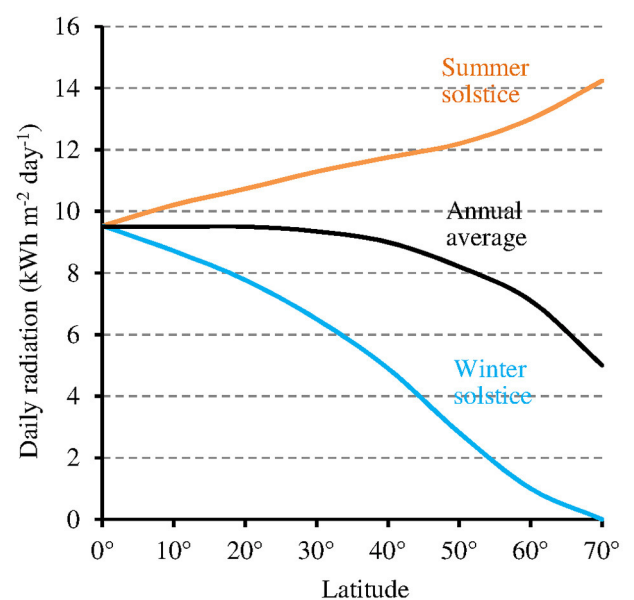
FIGURE 6 | Relation between latitude and total daily radiation under clear sky (annual average and at the two solstices of the year) (source: pvlighthouse, http://pveducation.org/pvc/drom/calculation-of-solar-insolation ).
