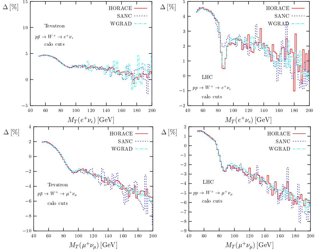
Fig. 4.4.96: The relative correction \Delta due to electroweak \mathcal{O}(\alpha) corrections to the M_T(l\nu) distribution for single W^+ production with calo cuts at the Tevatron and the LHC.
