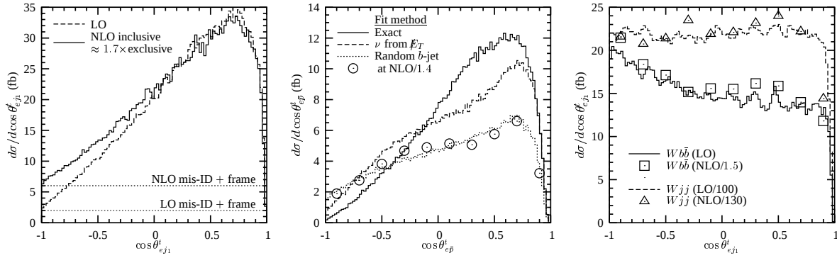
Fig. 3.2.44: Cosine of angle ( \cos \theta_{ej_1}^t ) between the charged lepton and the highest- E_T light-quark jet in the top-quark rest frame for (left) t -channel single-top-quark production, and (right) Wjj production at the Tevatron. (Center) cosine of angle between the lepton and antiproton for s -channel single-top-quark production.
