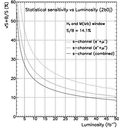
Fig. 3.4.77: Statistical sensitivity as a function of the integrated luminosity after the topological selection.
