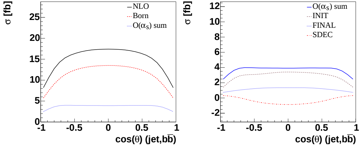
Fig. 3.2.20: Angular distance \cos\theta between a b -tagged jet and the (b\text{ jet}, \bar{b}\text{ jet}) system after selection cuts, comparing Born-level to O(\alpha_s) corrections.
