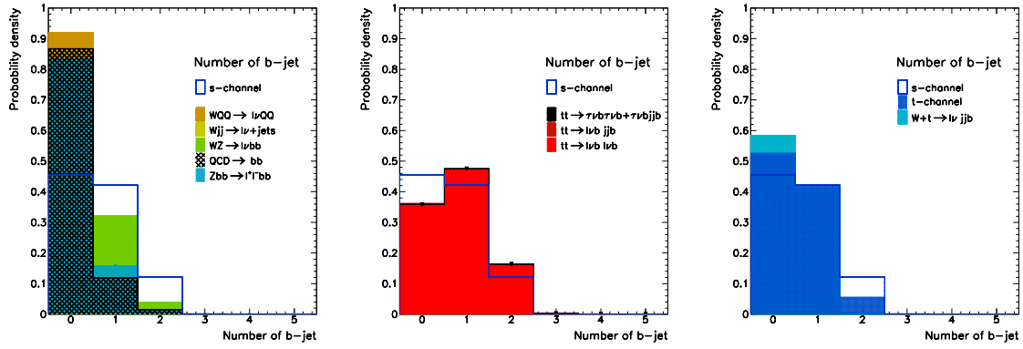
Fig. 3.4.67: Number of b-tagged jets for signal and backgrounds.
