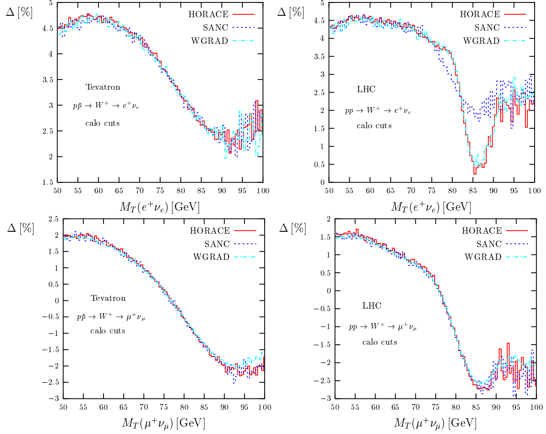
Fig. 4.4.94: The relative correction \Delta due to electroweak \mathcal{O}(\alpha) corrections to the M_T(l\nu) distribution for single W^+ production with calo cuts at the Tevatron and the LHC.
