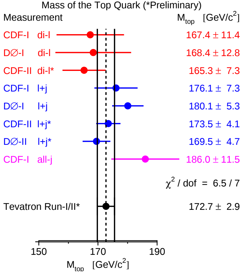
Fig. 2.4.7: The inputs for the Tevatron combined M_t combination and the resulting world average top quark mass, obtained as described in Section 2.4.
