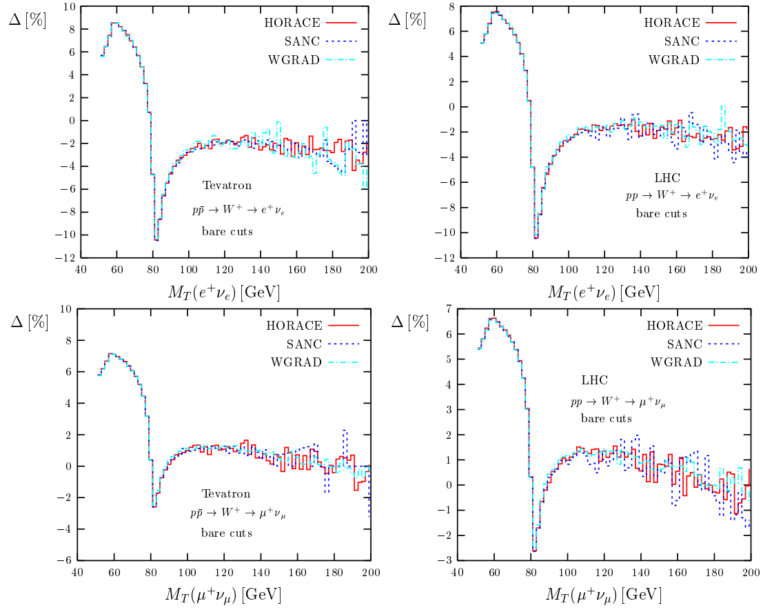
Fig. 4.4.95: The relative correction \Delta due to electroweak \mathcal{O}(\alpha) corrections to the M_T(l\nu) distribution for single W^+ production with bare cuts at the Tevatron and the LHC.
