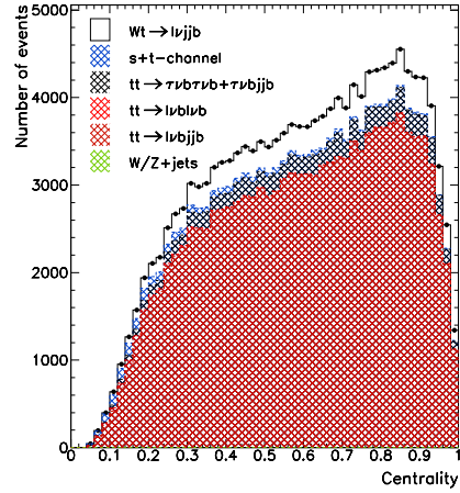
Fig. 3.4.88: Event yields for the centrality distribution for 30 \text{ fb}^{-1} .
