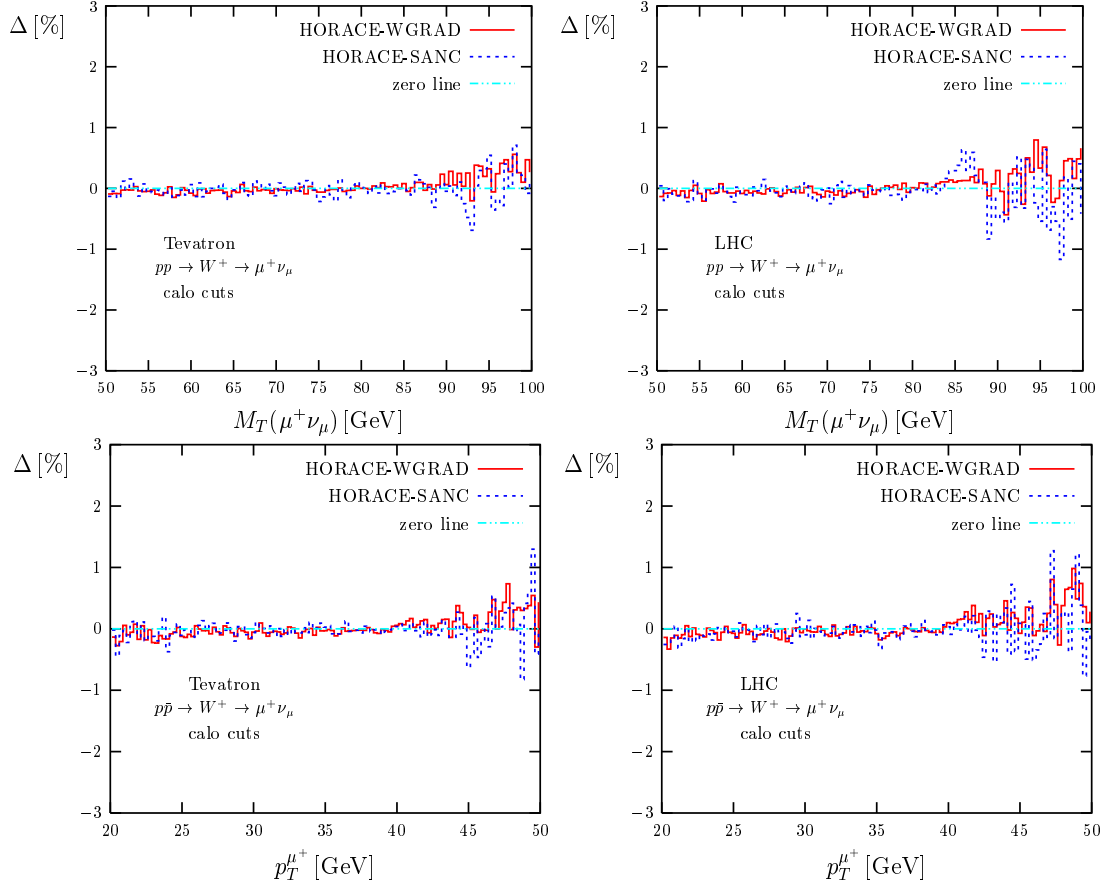
Fig. 4.4.101: Relative difference \Delta between HORACE and SANC NLO predictions as well as HORACE and WGRAD NLO predictions for the M_T(\mu^+ \nu_\mu) and p_T^{\mu^+} distributions for single W^+ production with calo cuts at the Tevatron and the LHC.
