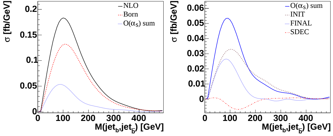
Fig. 3.2.19: Invariant mass of the (b\text{-jet}, \bar{b}\text{-jet}) system after selection cuts, comparing Born-level to O(\alpha_s) corrections. In the legend, INIT, FINAL and SDEC denotes the contributions from initial state, final state and top quark decay corrections, respectively.
