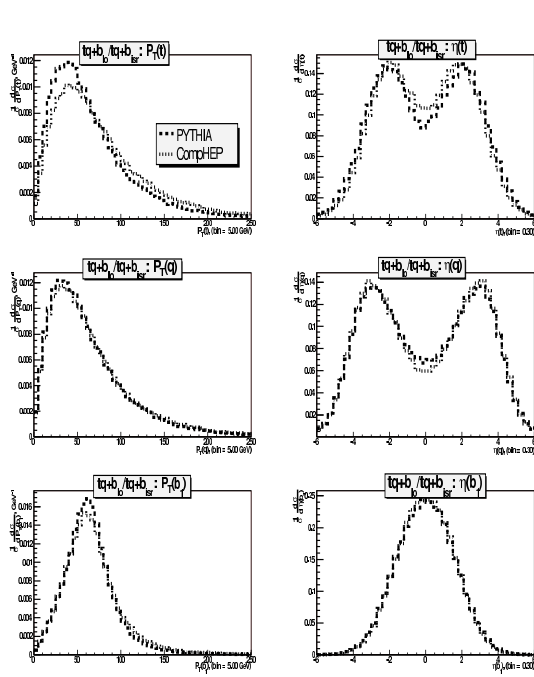
Fig. 3.2.35: The comparison of P_T and \eta distributions for the pp \rightarrow tq + b_{ISR} (PYTHIA) and pp \rightarrow tq + b_{LO} (CompHEP) simulations for the LHC. The distributions are normalized to unity and no cuts applied.
