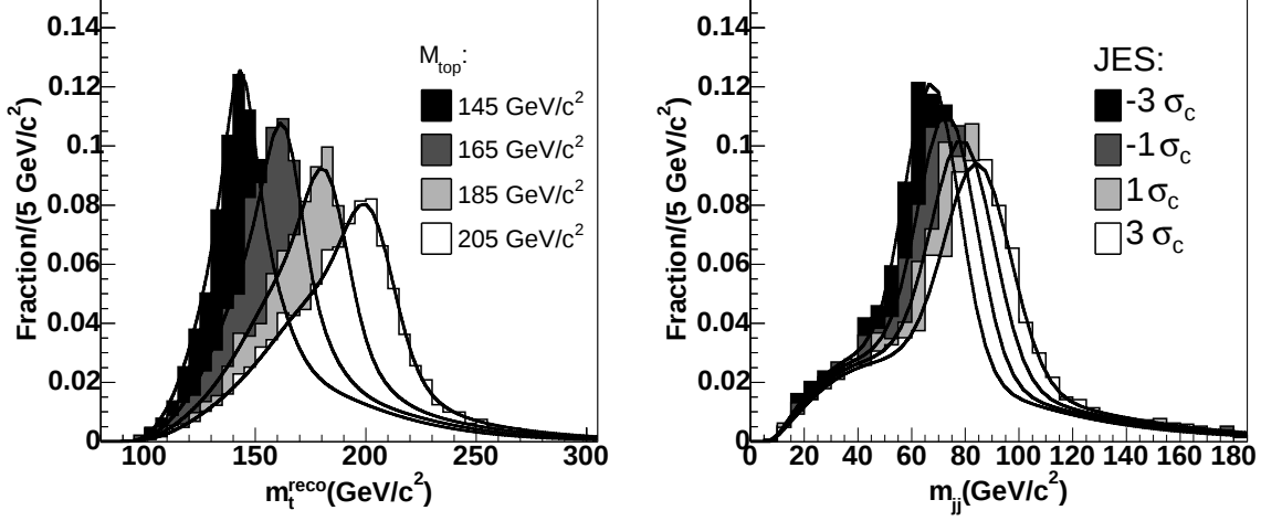
Fig. 2.2.4: [Left] Signal m_t^{reco} templates for 1-btag(T) sample are shown with top quark masses ranging from 145 \text{GeV}/c^2 to 205 \text{GeV}/c^2 and with JES set to 0. [Right] Signal m_{jj} templates for the 2-btag sample are shown with different values of the JES.
