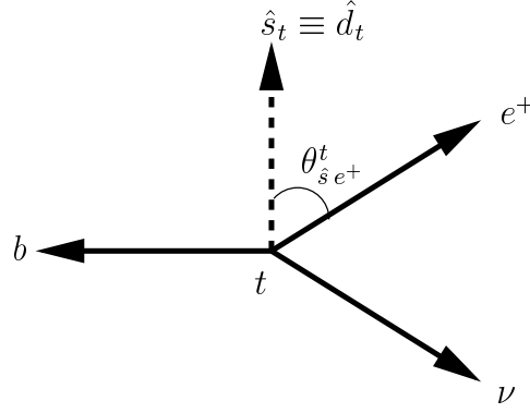
Fig. 3.2.43: Decay products of the top quark, and the angle \theta_{\hat{s} e^+}^t between the charged lepton e^+ and the spin \hat{s}_t of the top quark in the top-quark rest frame. The spin is projected in the direction of the down-type quark d in the event.
