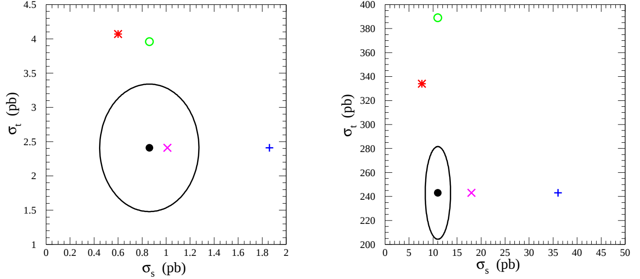
Fig. 3.2.16: Single top cross sections in the s - and t -channels in the SM (including theoretical and expected statistical uncertainties) and a few models of physics beyond the SM, at the Tevatron run II and LHC (from Ref. [81]).
