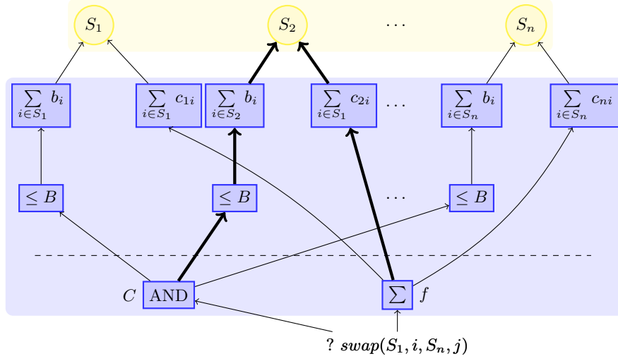
Figure 2.3: Representation of the CBLS model for the GAP. The top level represents all the set variables. The bottom level represents all the differential invariants stating the objective function and the constraints. The sums directly depends on the variables, while the differential invariants representing the global objective function and the constraints depends on other invariants. The thick edges represents the part of the model that has to be updated when the variable S_2 is modified. All differential invariants can be queried to compute their differentiation wrt the move swapping the elements i and j from variables S_1 and S_n for example. This allows to the search procedure to differentiate the model to select the best move to apply eventhough it has no knowledge about the model. This allows the model to be separated from the search procedure, as illustrated by the dashed line.
