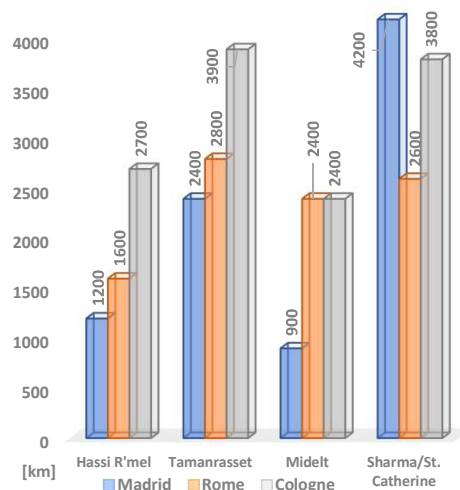
Figure 3 The pipelines/distance between H 2 production and consumption locations
