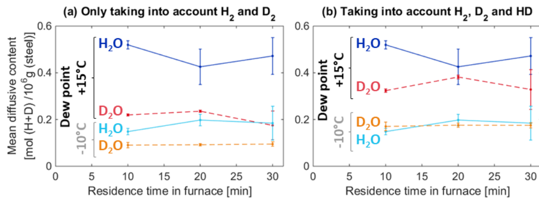
Figure 2 – Mean diffusive contents (expressed as the sum of desorbed H and D) as a function of the residence time and of the atmosphere composition by (a) only taking into account the \text{H}_2 and \text{D}_2 contributions and (b) by adding the \text{HD} contribution to previous results.
